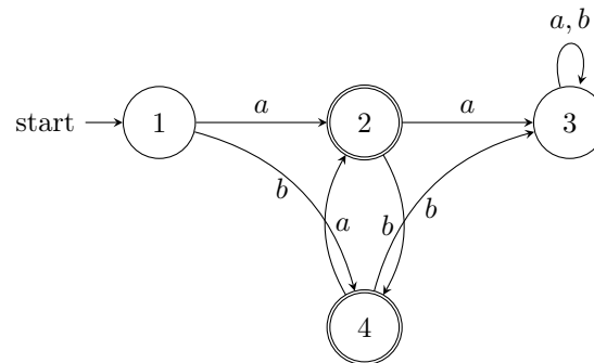
Figure 9: Automaton \mathcal{A}^{(1)}
