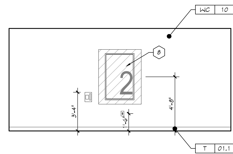
5 ELEVATOR LOBBY UPPER FLOORS SCALE: 1/4" = 1'-0"
