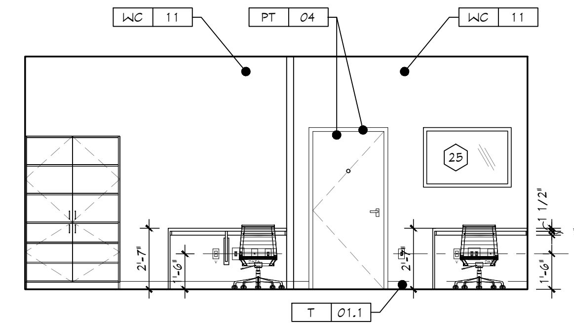
6 WORKROOM SCALE: 1/4" = 1'-0"
