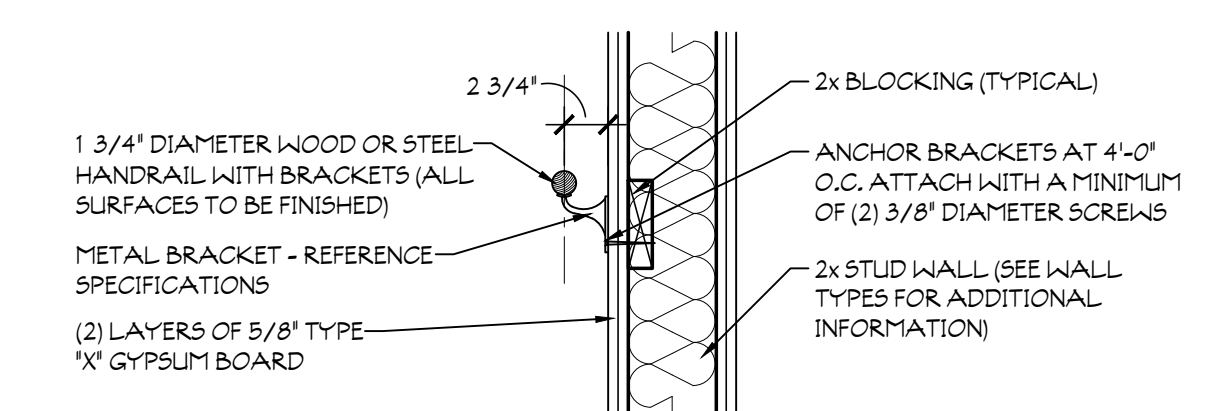
12 HANDRAIL DETAIL SCALE: 1" = 1'-0"
