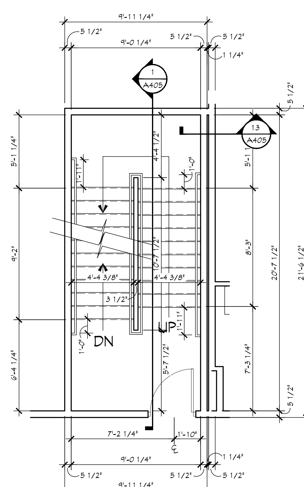
6 SECOND FLOOR STAIR PLAN #2 SCALE: 1/4" = 1'-0"
