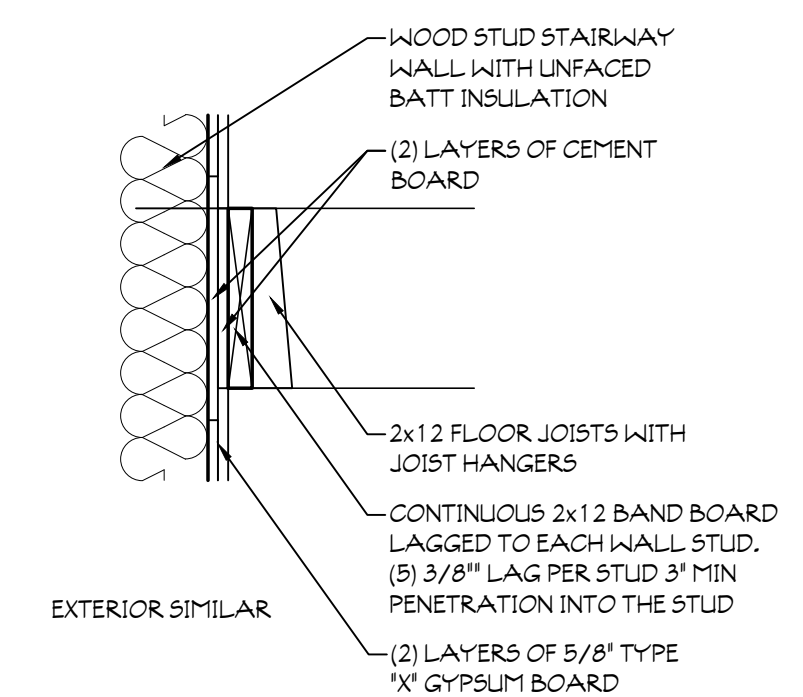
13 STAIR LANDING DETAIL SCALE: 1" = 1'-0"
