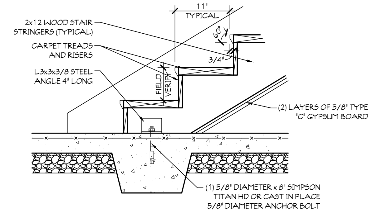
9 STAIR TO FLOOR SLAB DETAIL SCALE: 1" = 1'-0"
