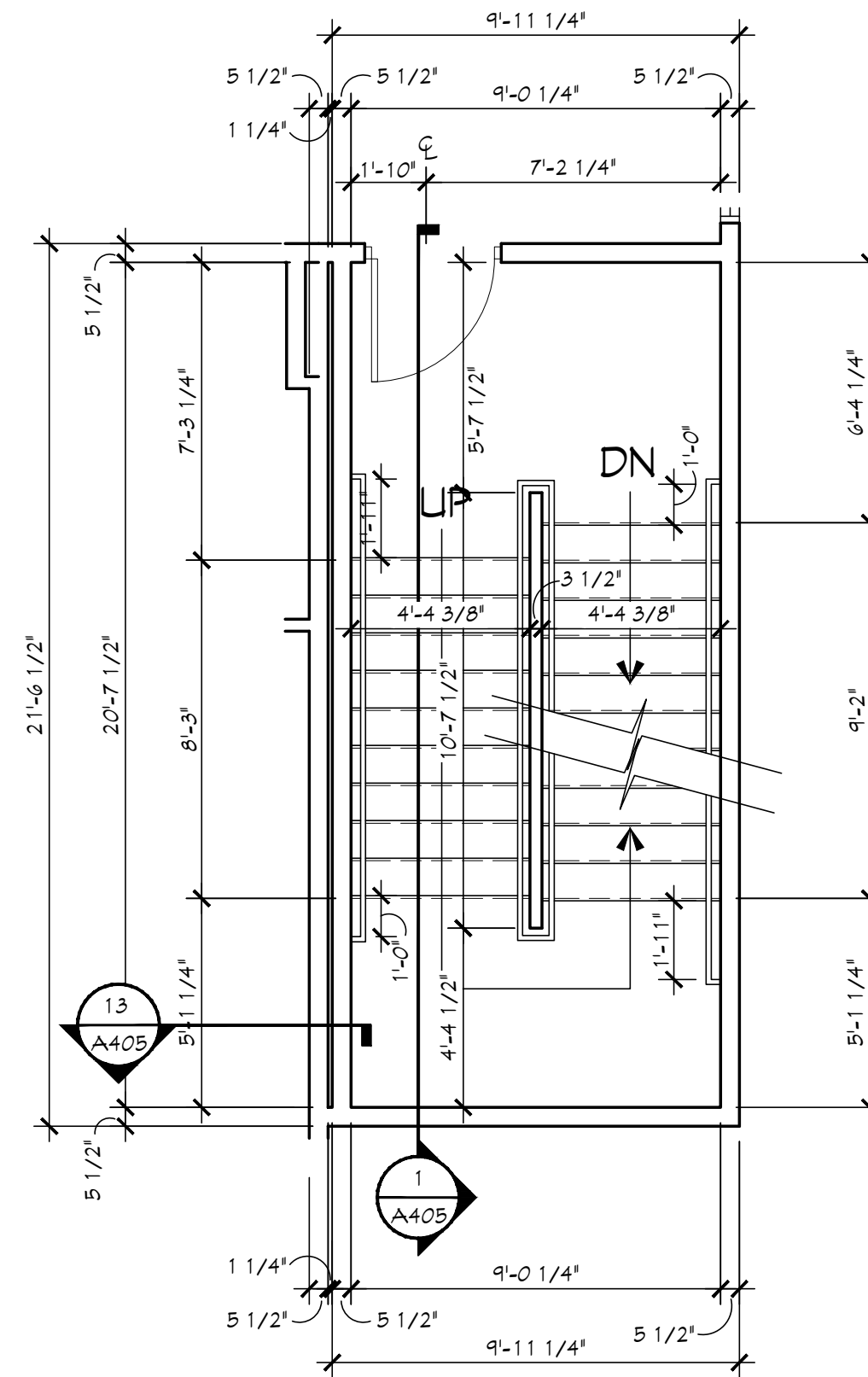
2 SECOND FLOOR STAIR PLAN #1 SCALE: 1/4" = 1'-0"
