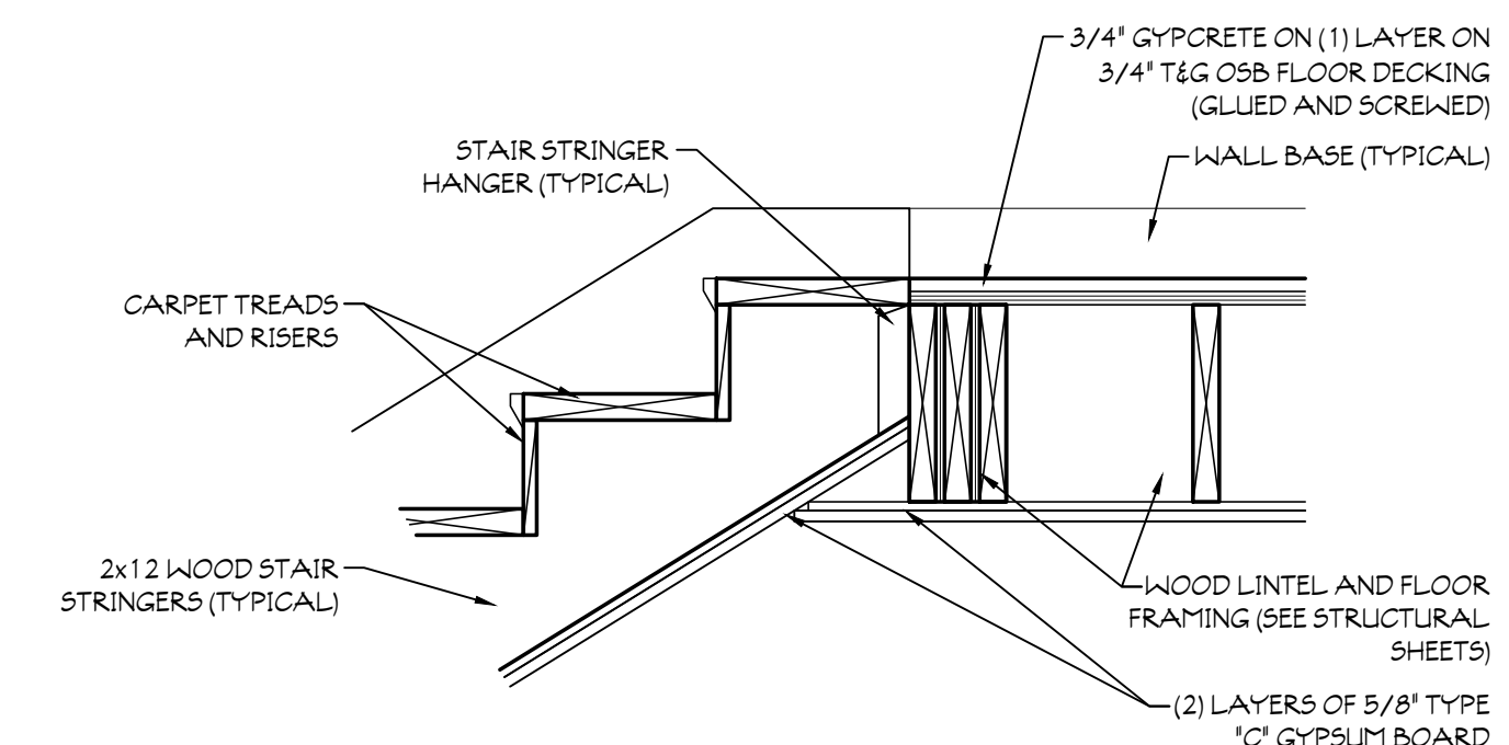
11 STAIR TO LANDING DETAIL SCALE: 1" = 1'-0"
