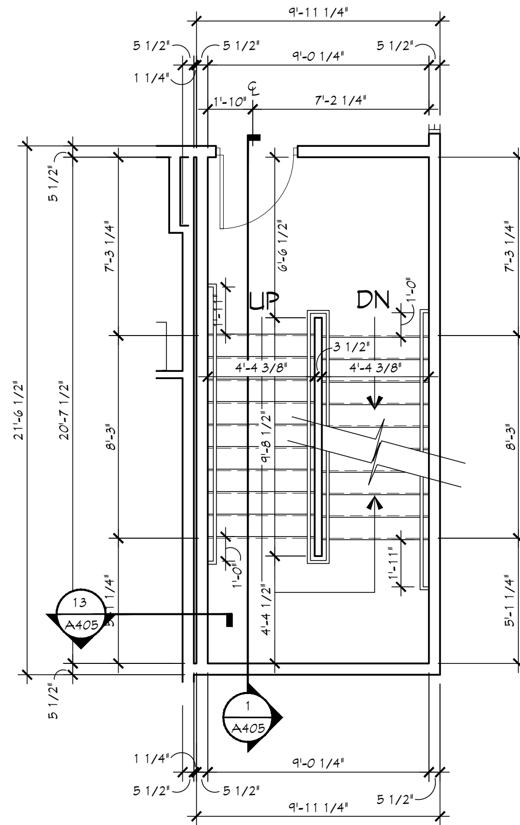
3 THIRD FLOOR STAIR PLAN #1 SCALE: 1/4" = 1'-0"
