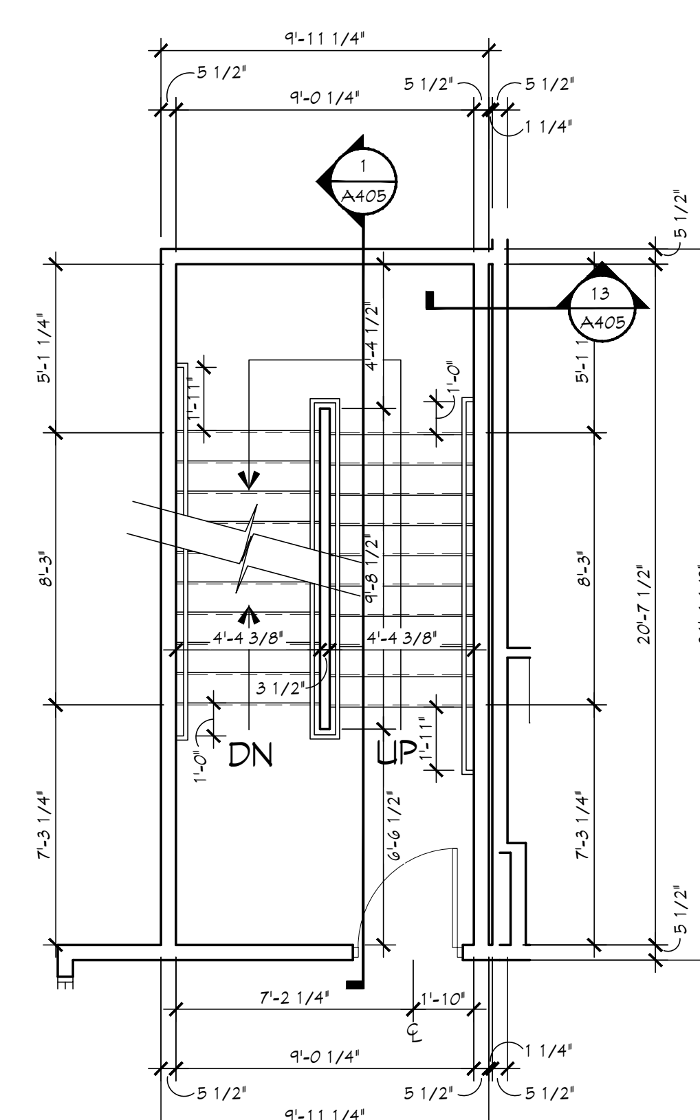
7 THIRD FLOOR STAIR PLAN #2 SCALE: 1/4" = 1'-0"
