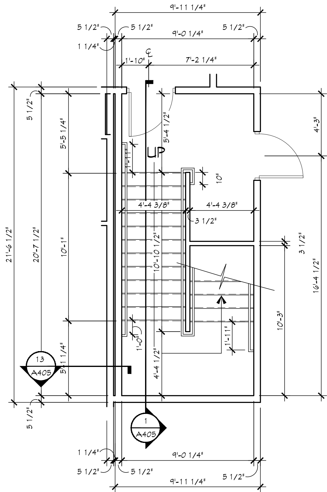
1 FIRST FLOOR STAIR PLAN #1 SCALE: 1/4" = 1'-0"
