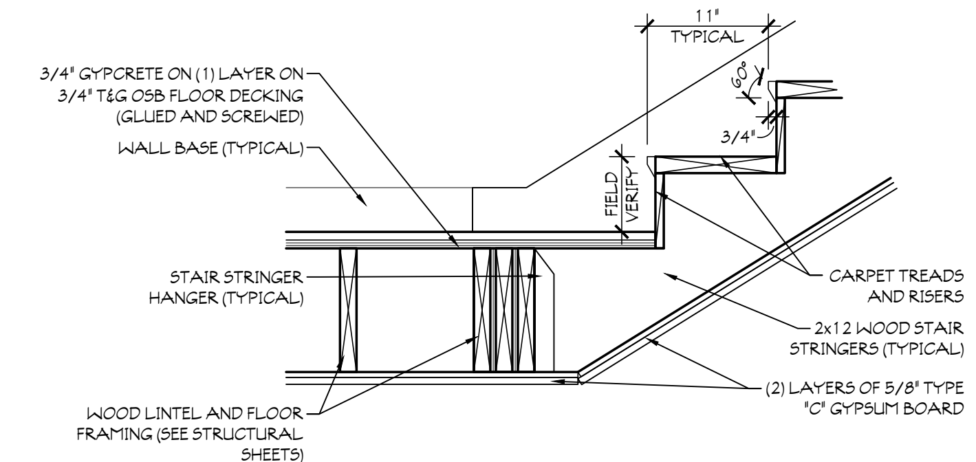
10 STAIR TO LANDING DETAIL SCALE: 1" = 1'-0"
