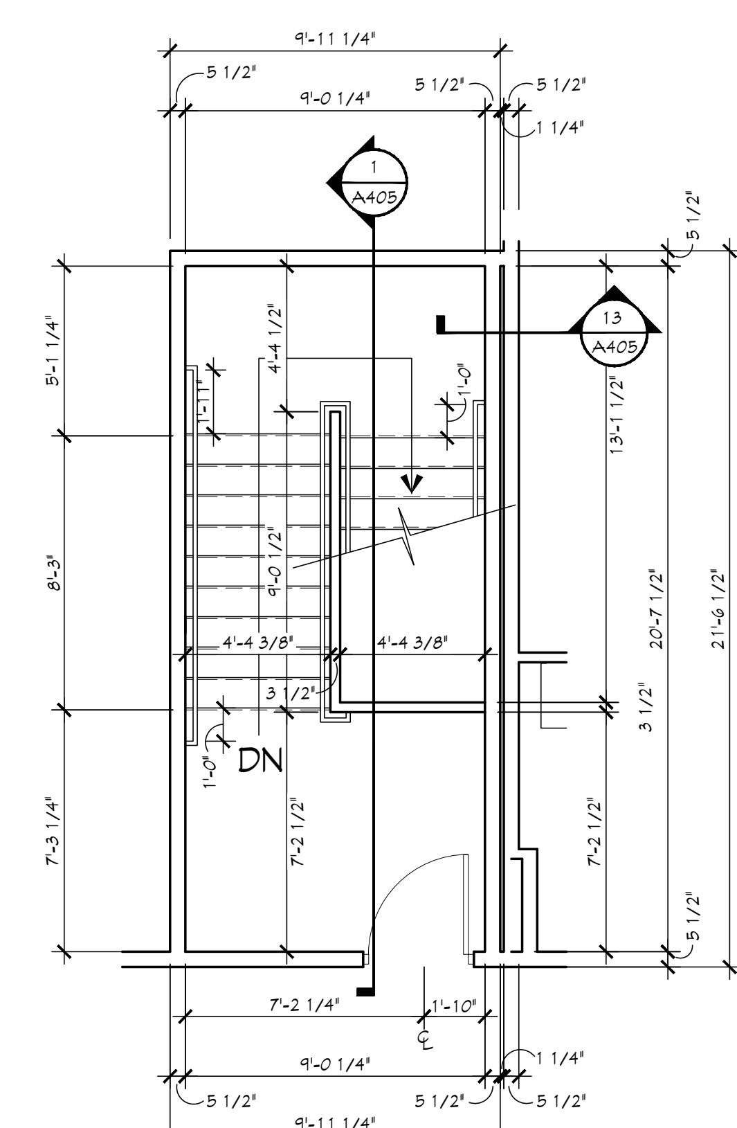
8 FOURTH FLOOR STAIR PLAN #2 SCALE: 1/4" = 1'-0"
