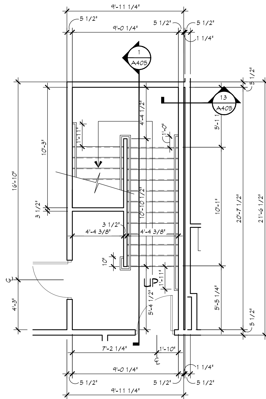
5 FIRST FLOOR STAIR PLAN #2 SCALE: 1/4" = 1'-0"
