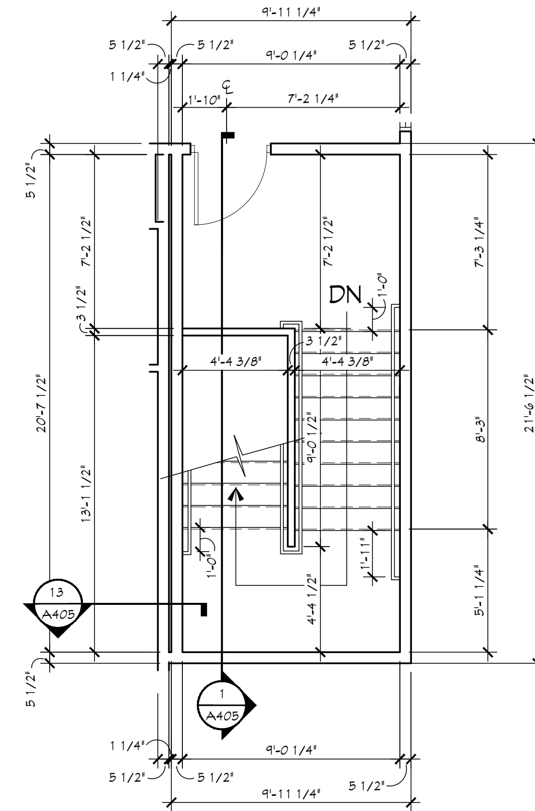
4 FOURTH FLOOR STAIR PLAN #1 SCALE: 1/4" = 1'-0"
