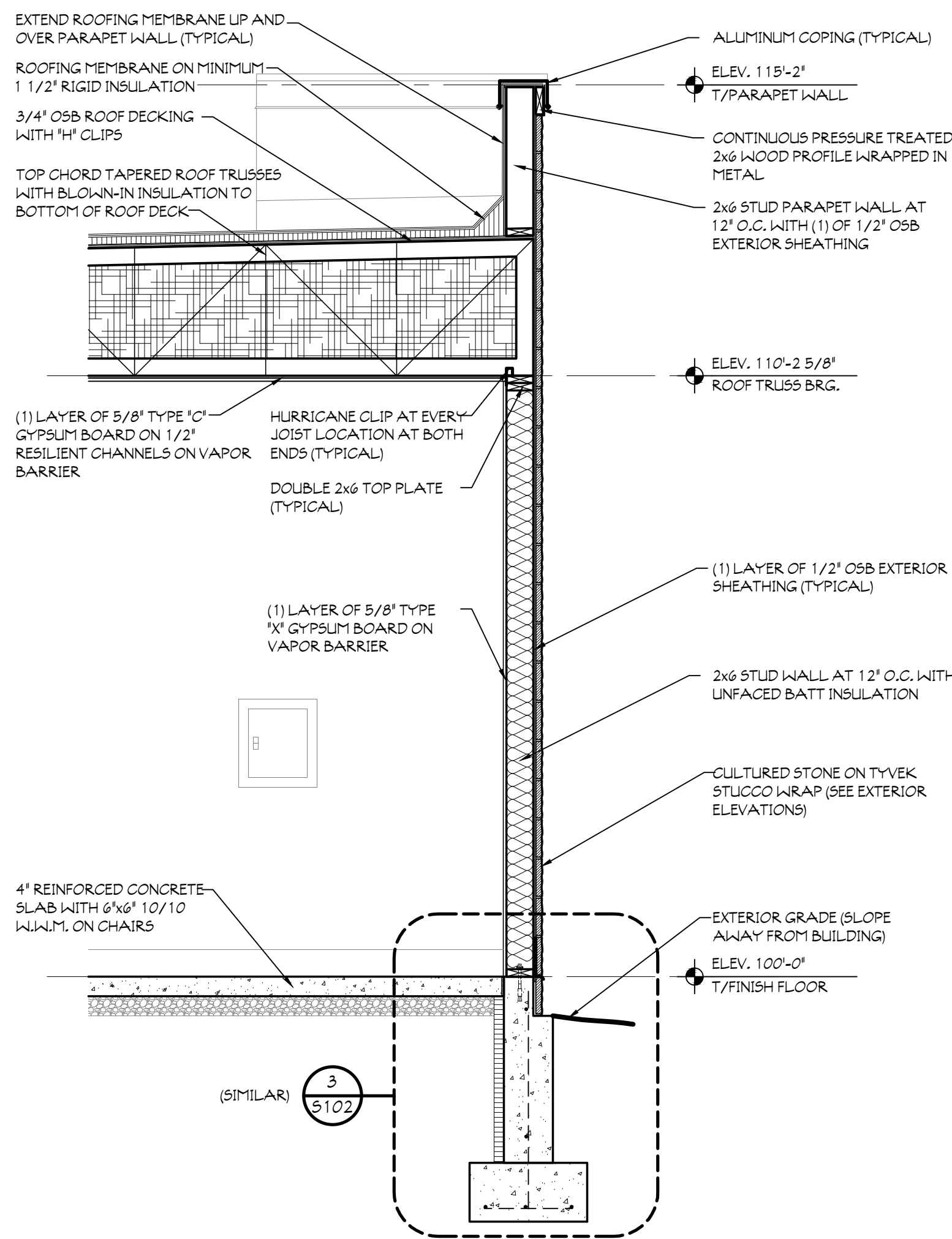
1 SINGLE STORY SECTION SCALE: 1/2" = 1'-0" AT POOL EXTERIOR WALL
