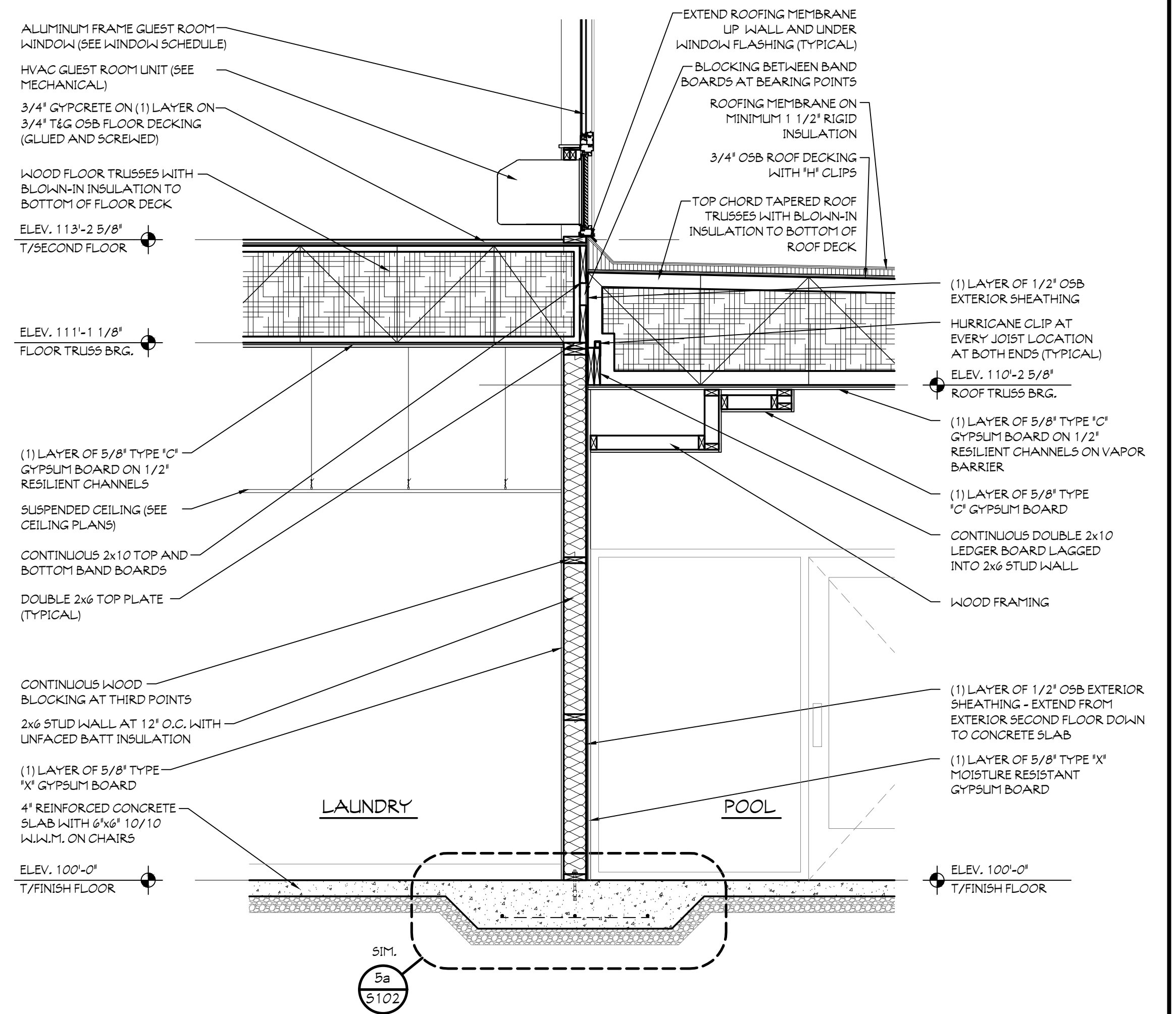
3 INTERIOR BEARING WALL SECTION SCALE: 1/2" = 1'-0" AT POOL INTERIOR WALL
