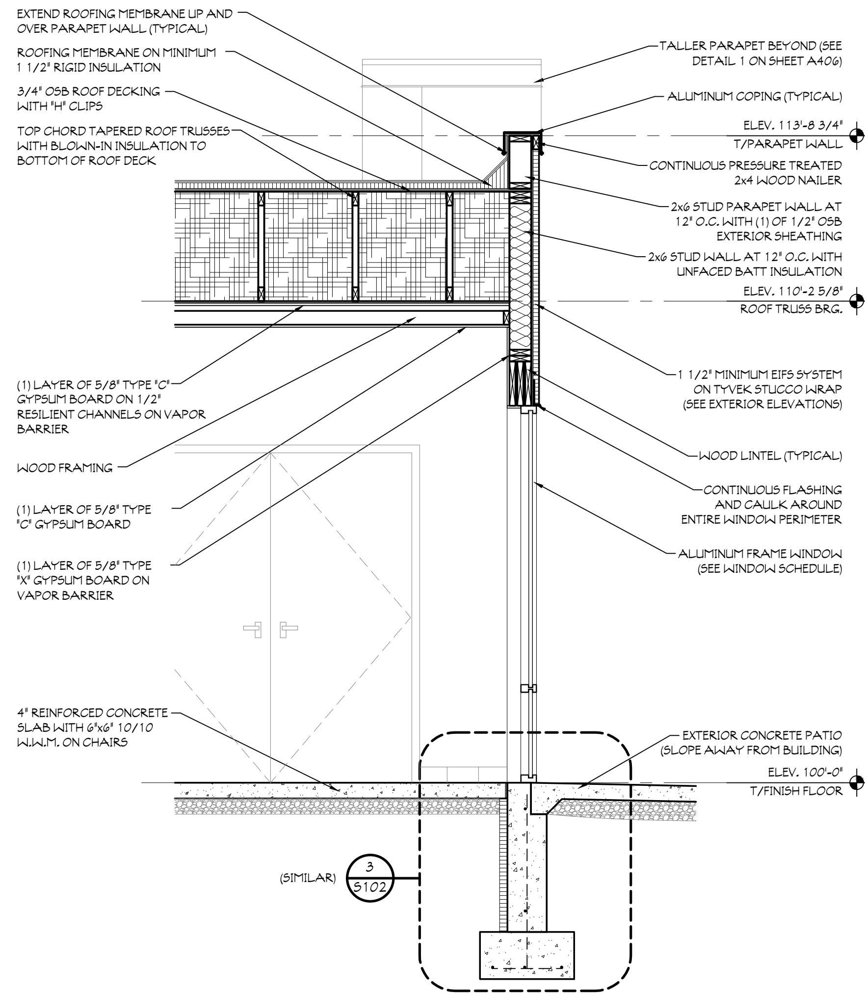
2 SINGLE STORY SECTION SCALE: 1/2" = 1'-0" AT POOL EXTERIOR WALL
