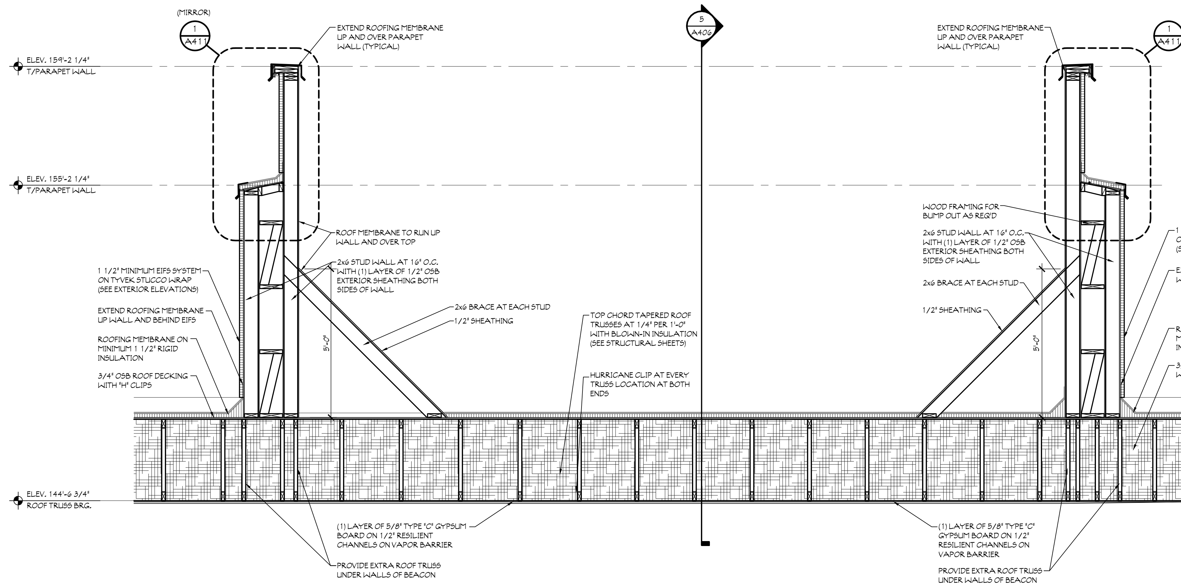
4 BEACON SECTION SCALE: 1/2" = 1'-0"
