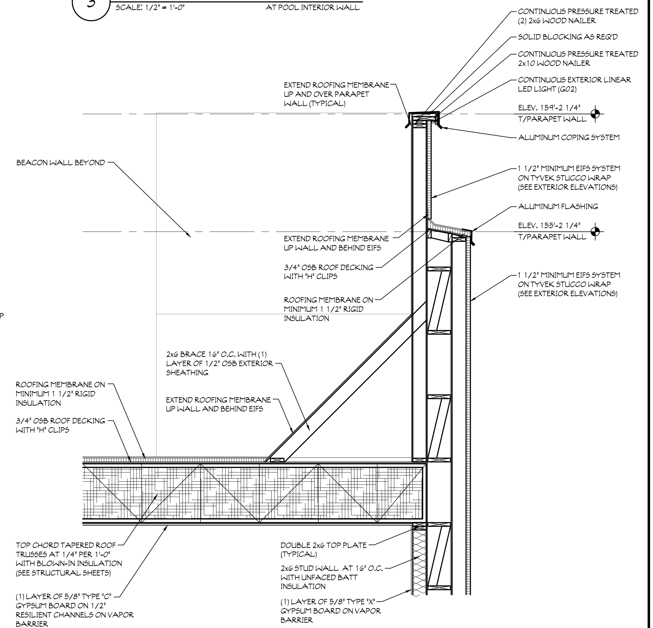
5 BEACON SECTION SCALE: 1/2" = 1'-0"
