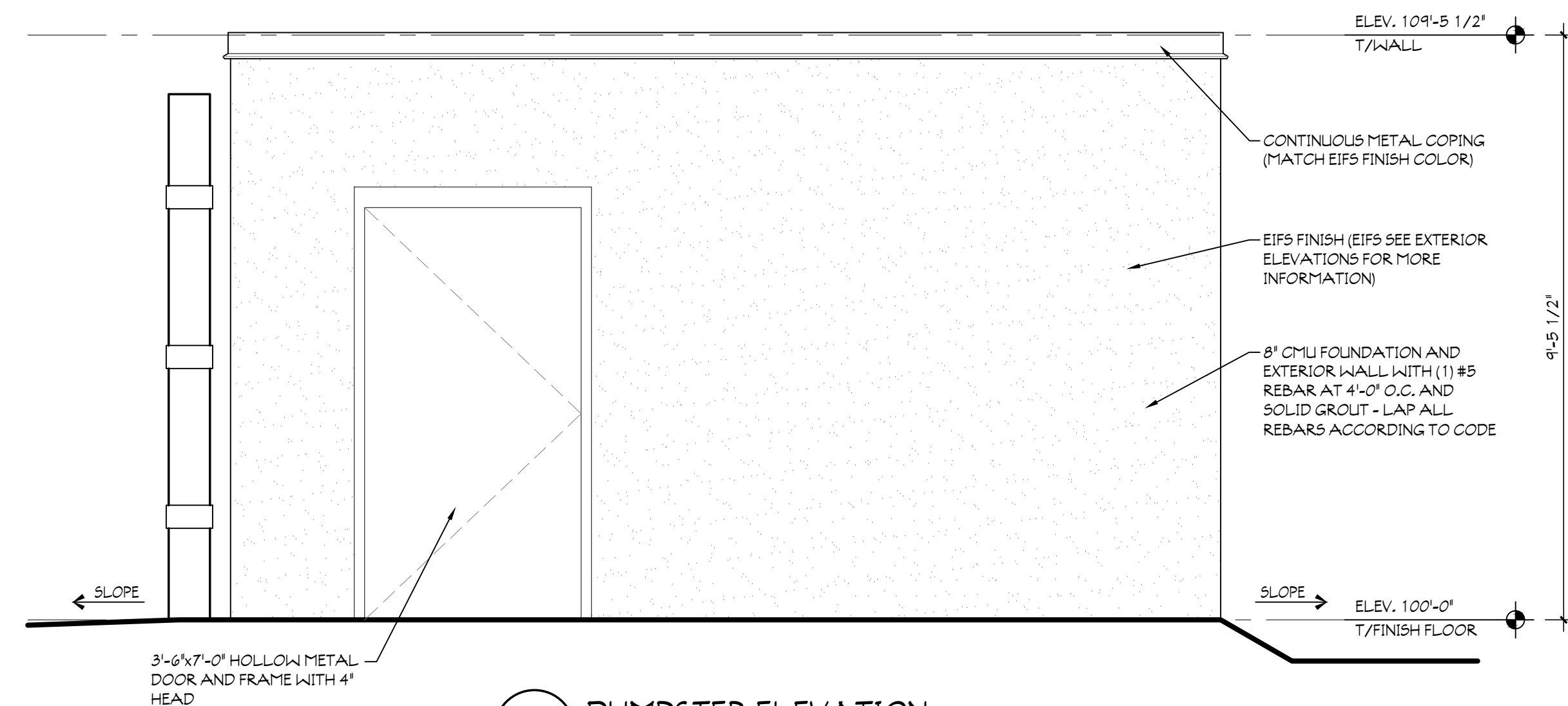
2 DUMPSTER ELEVATION SCALE: 1/2" = 1'-0" TYPICAL SIDE ELEVATION
