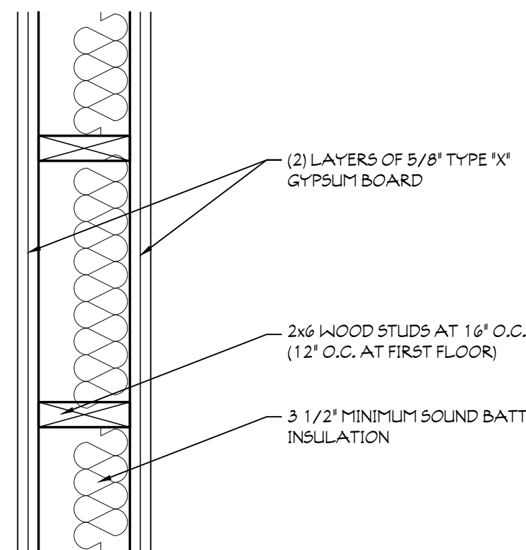
9 STAIR WALL TYPE UL# U301 SCALE: 1 1/2" = 1'-0" FIRE: 2 HOUR - STC: 56
