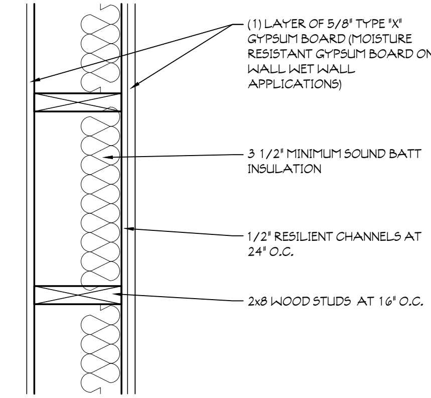
5 PLUMBING WALL TYPE UL# U305 SCALE: 1 1/2" = 1'-0" FIRE: 1 HOUR - STC: 56
