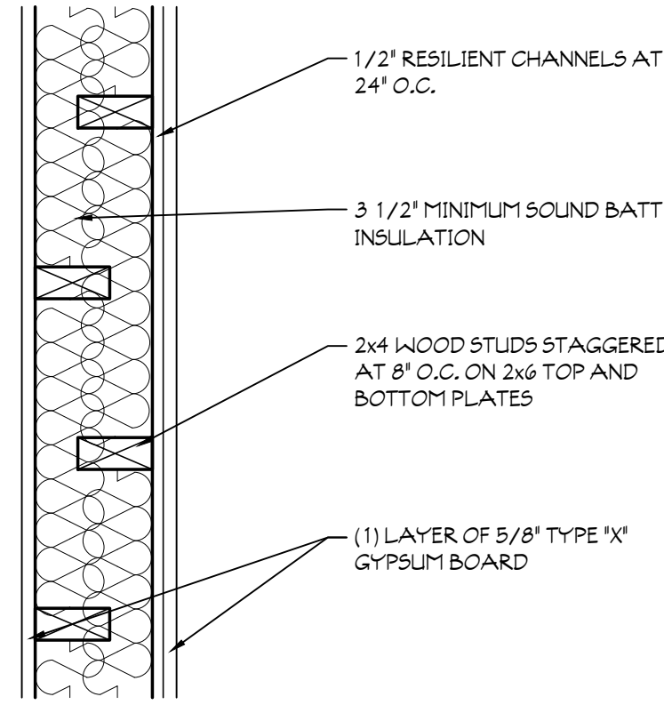
2 GUEST ROOM WALL TYPE UL# U340 SCALE: 1 1/2" = 1'-0" FIRE: 1 HOUR - STC: 51
