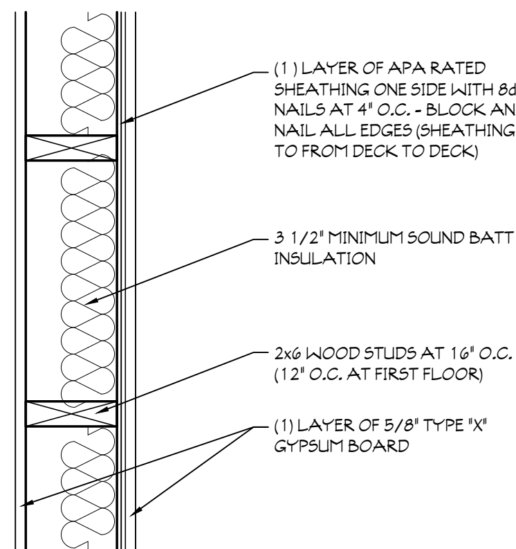
10 INTERIOR BEARING WALL UL# U311 SCALE: 1 1/2" = 1'-0" FIRE: 1 HOUR - STC: 52
