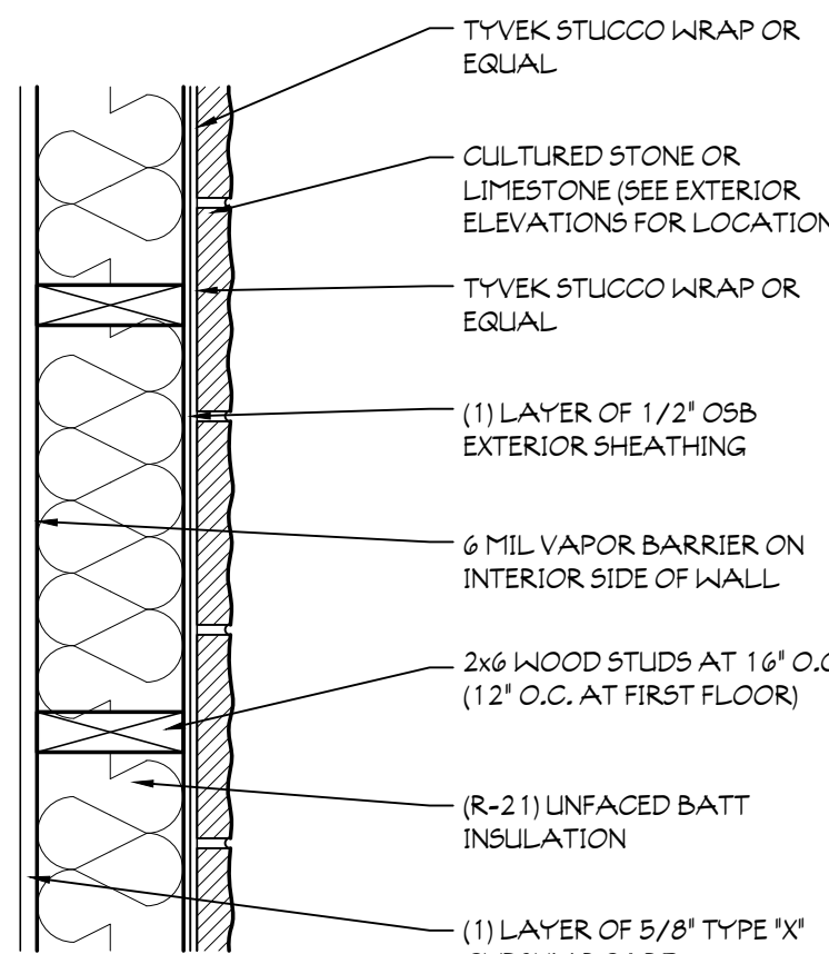
7b EXTERIOR WALL TYPE UL# U356 SCALE: 1 1/2" = 1'-0" FIRE: 1 HOUR - STC: 56
