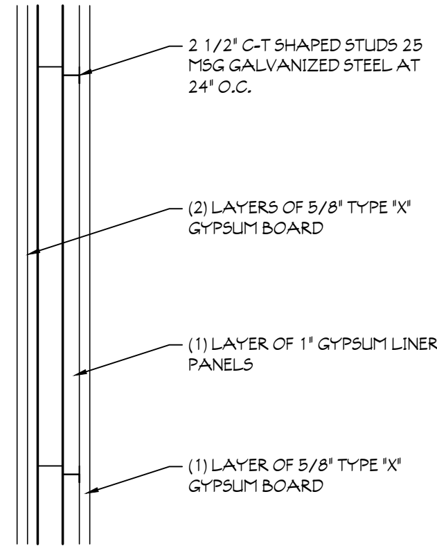
6a CHASE WALL TYPE UL# U417 SCALE: 1 1/2" = 1'-0" FIRE: 2 HOUR - STC: 43
