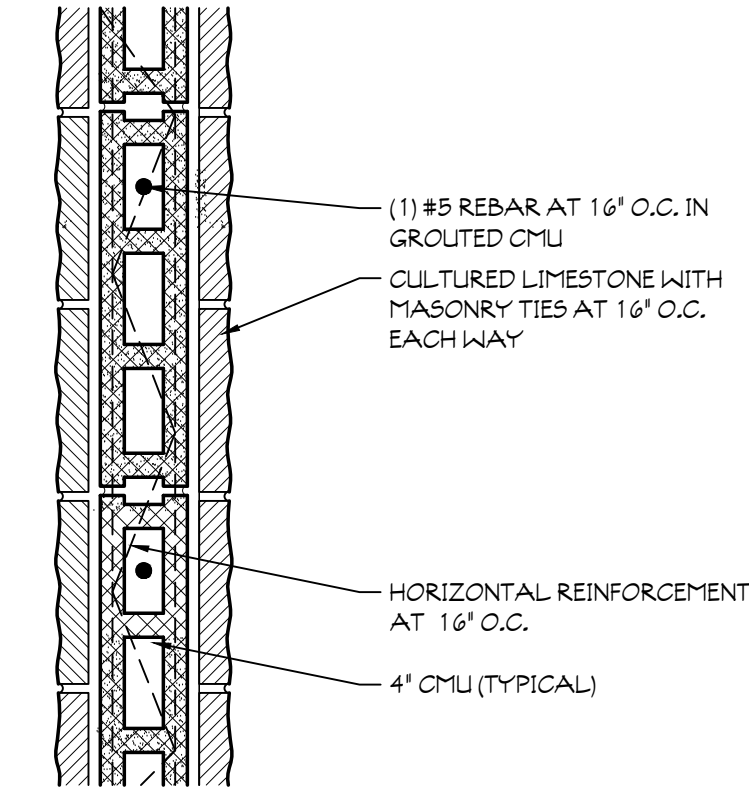
7c EXTERIOR WALL TYPE UL# U914 SCALE: 1 1/2" = 1'-0" FIRE: 3 HOUR - STC: 52-56
