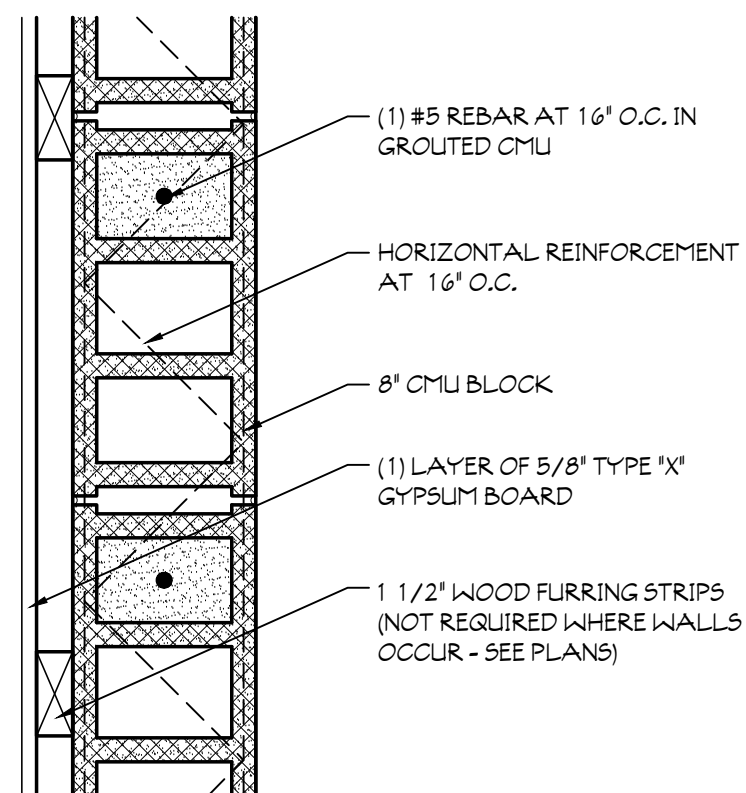
8 ELEVATOR WALL TYPE UL# U914 SCALE: 1 1/2" = 1'-0" FIRE: 3 HOUR - STC: N/A
