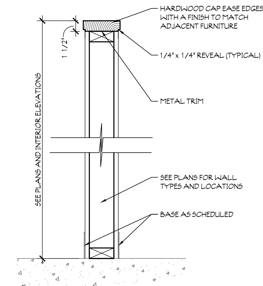
12 LOW HEIGHT WALL SECTION SCALE: 1 1/2" = 1'-0" @ STAIR FOURTH FLOOR, SEE STAIR SECTION
