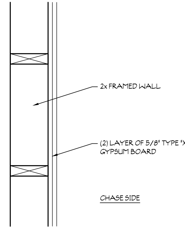
6b CHASE WALL TYPE UL# SCALE: 1 1/2" = 1'-0" FIRE: 1 HOUR - STC: N/A
