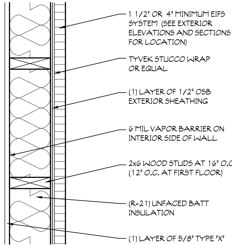
7a EXTERIOR WALL TYPE UL# U356 SCALE: 1 1/2" = 1'-0" FIRE: 1 HOUR - STC: 56
