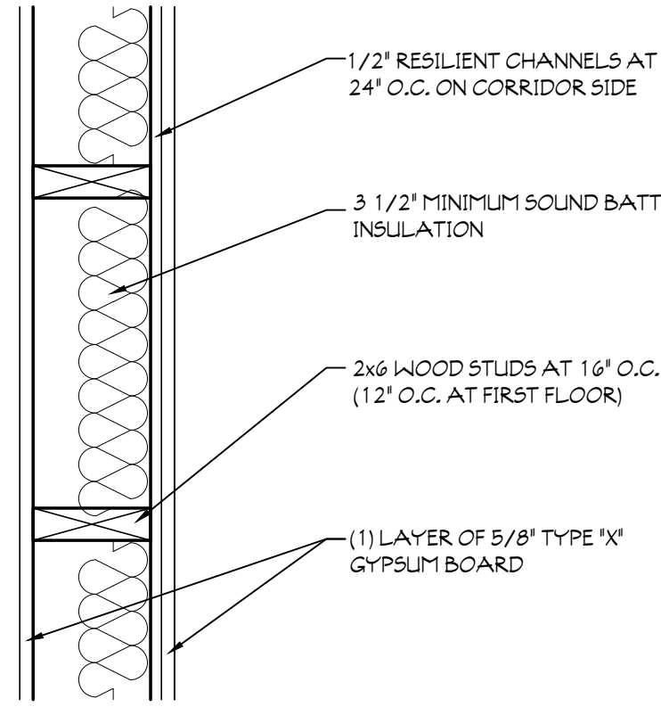
1 CORRIDOR WALL TYPE UL# U311 SCALE: 1 1/2" = 1'-0" FIRE: 1 HOUR - STC: 52
