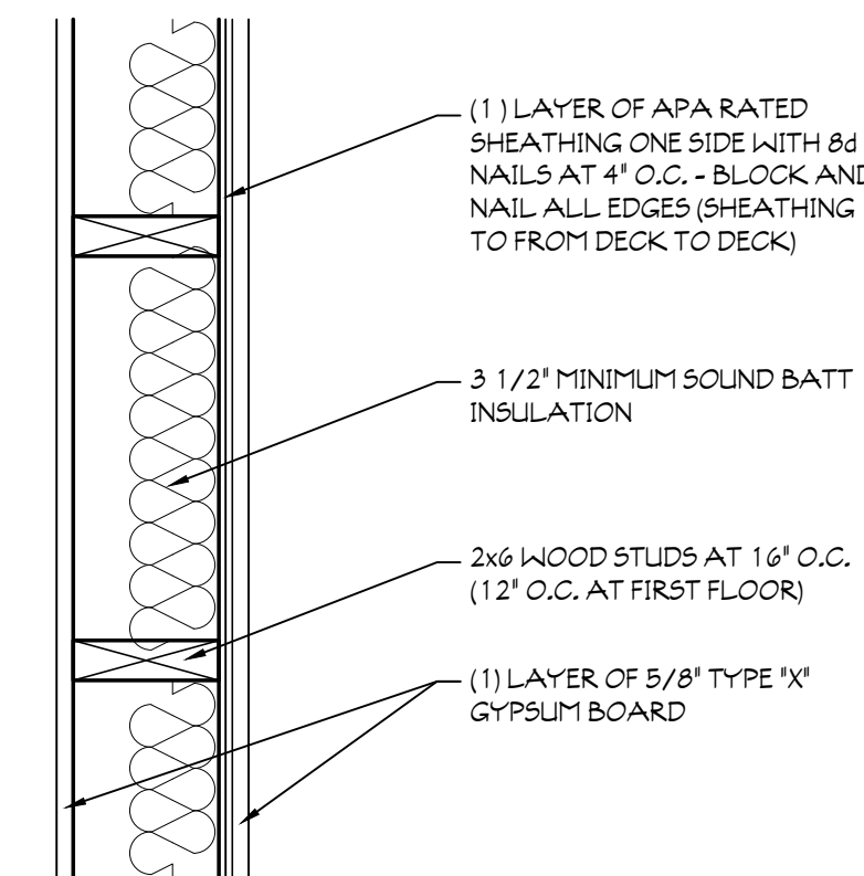
11 SHEAR WALL TYPE UL# U311 SCALE: 1 1/2" = 1'-0" FIRE: 1 HOUR - STC: 52
