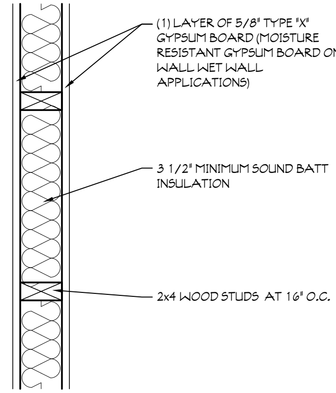
3 INTERIOR WALL TYPE UL# U333 SCALE: 1 1/2" = 1'-0" FIRE: 1 HOUR - STC: 36
