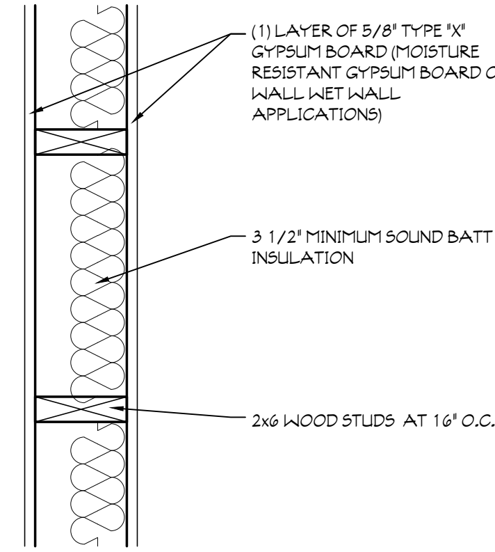
4 INTERIOR WALL TYPE UL# U305 SCALE: 1 1/2" = 1'-0" FIRE: 1 HOUR - STC: 38
