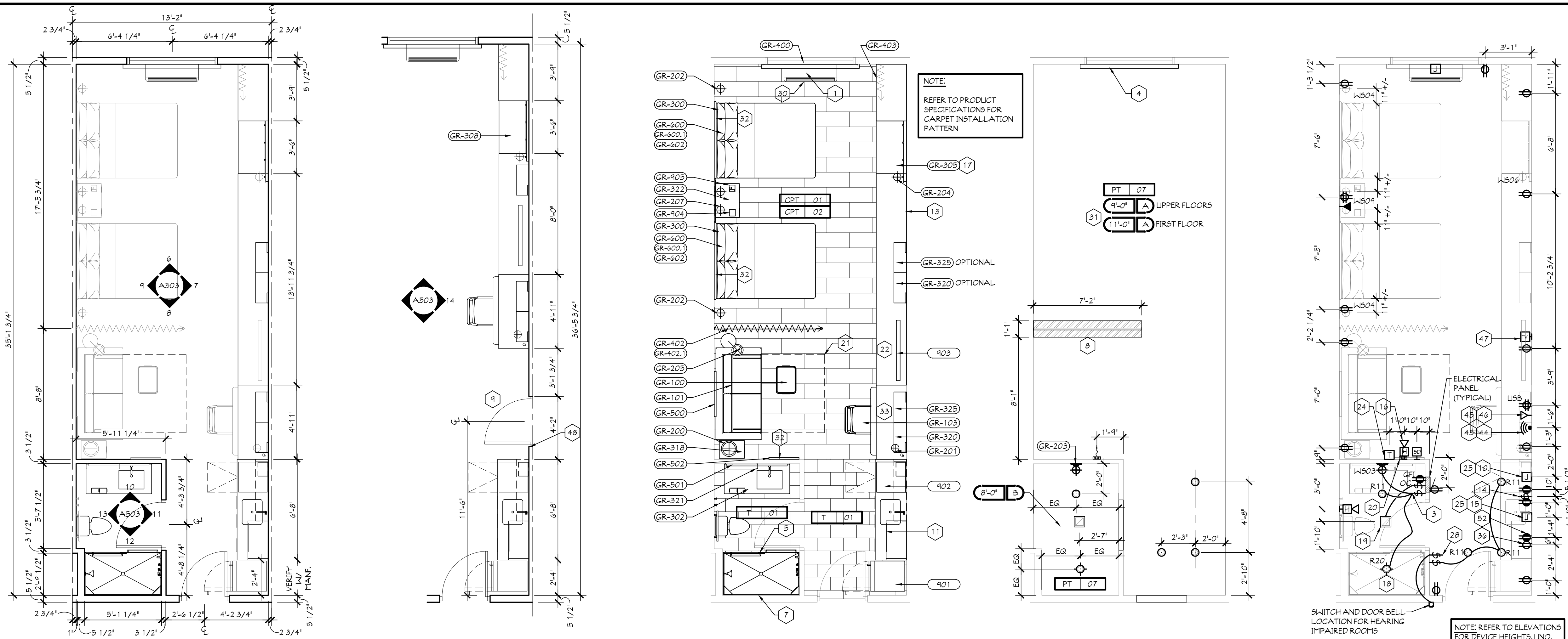
1 DOUBLE QUEEN STUDIO PLAN SCALE: 1/4" = 1'-0" 2 DOUBLE QUEEN CONNECTING PLAN SCALE: 1/4" = 1'-0" 3 DOUBLE QUEEN STUDIO FF&E PLAN SCALE: 1/4" = 1'-0" 4 DOUBLE QUEEN STUDIO CEILING SCALE: 1/4" = 1'-0" 5 DOUBLE QUEEN STUDIO ELEC. SCALE: 1/4" = 1'-0"
