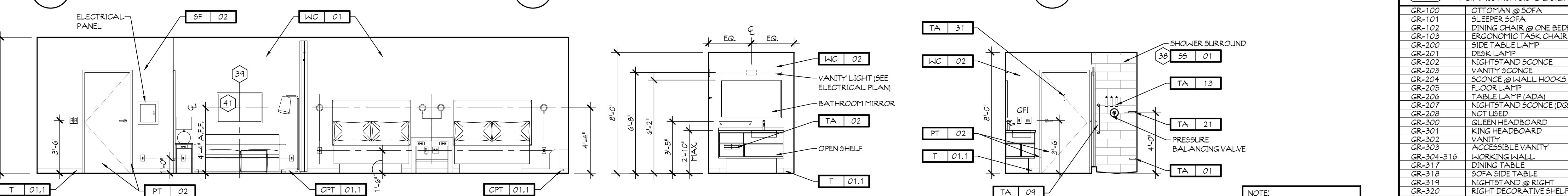
9 ROOM ELEVATION SCALE: 1/4" = 1'-0" 10 BATHROOM ELEVATION SCALE: 1/4" = 1'-0" 11 BATHROOM ELEVATION SCALE: 1/4" = 1'-0"
