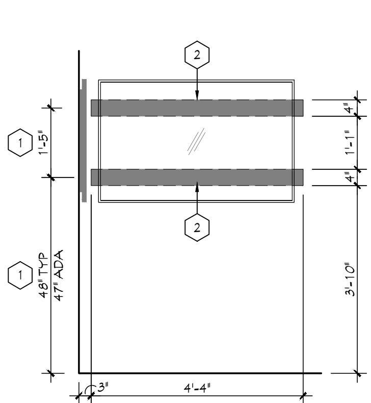
GR-503 - VANITY MIRROR
