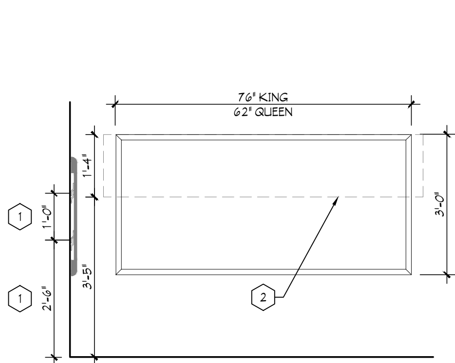
GR-300 - QUEEN HEADBOARD GR-301 - KING HEADBOARD
