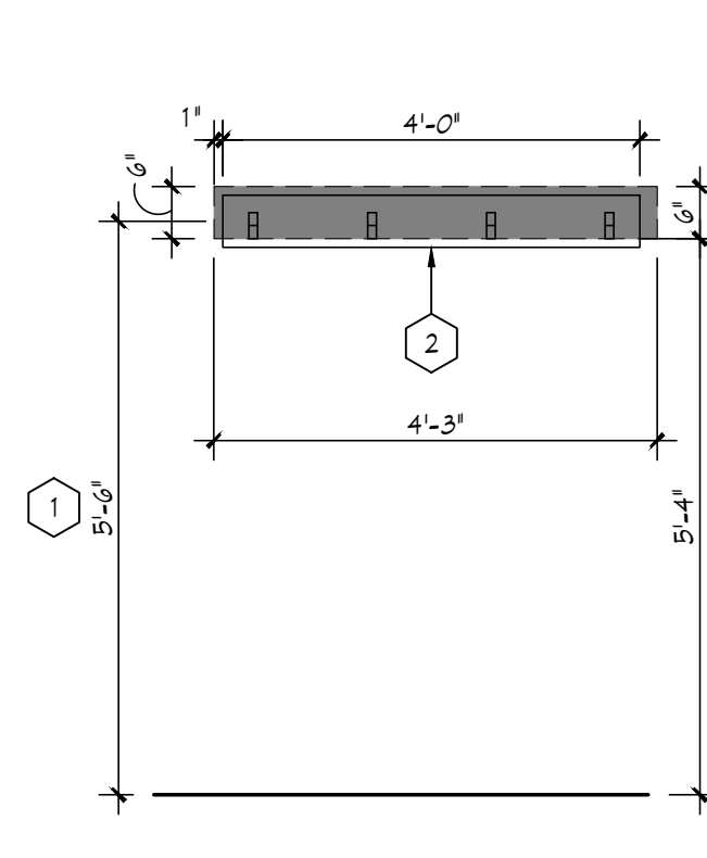
WORKING WALL - WALL HOOKS
