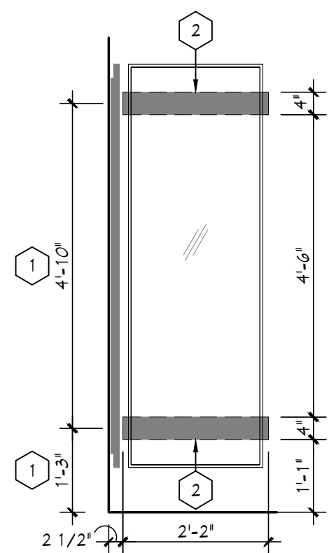
GR-504 - FULL LENGTH MIRROR
