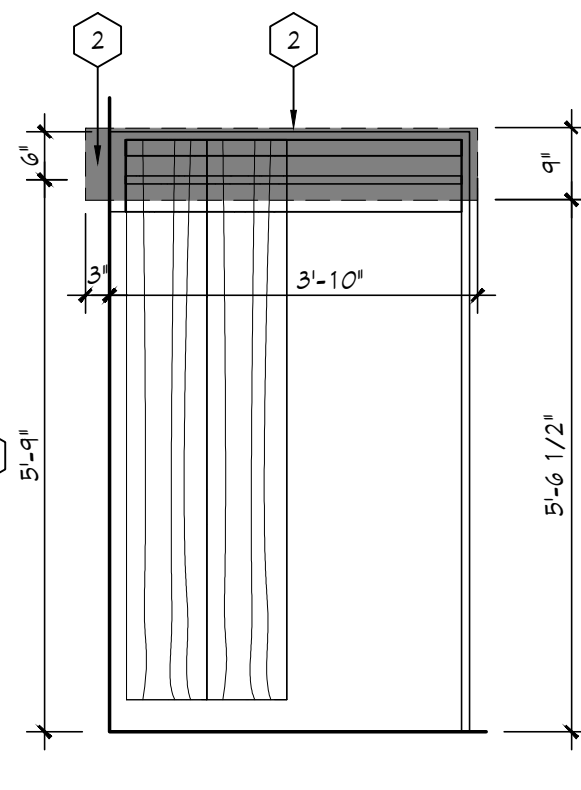
WORKING WALL - WARDROBE FRONT ELEVATION
