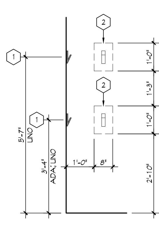
HD-04 - ROBE / TOWEL HOOKS, SURFACE MOUNTED
