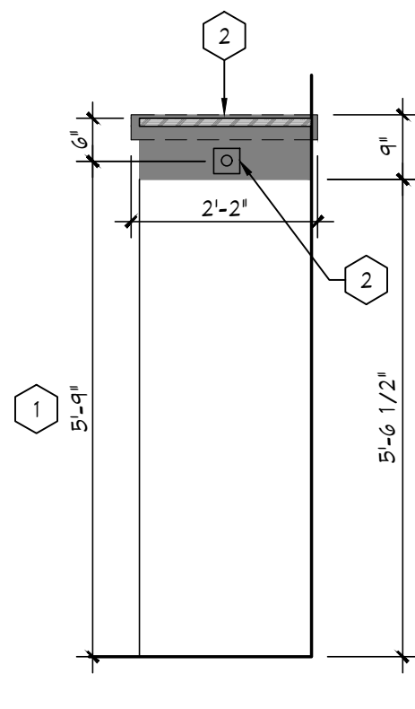
WORKING WALL - WARDROBE SIDE ELEVATION
