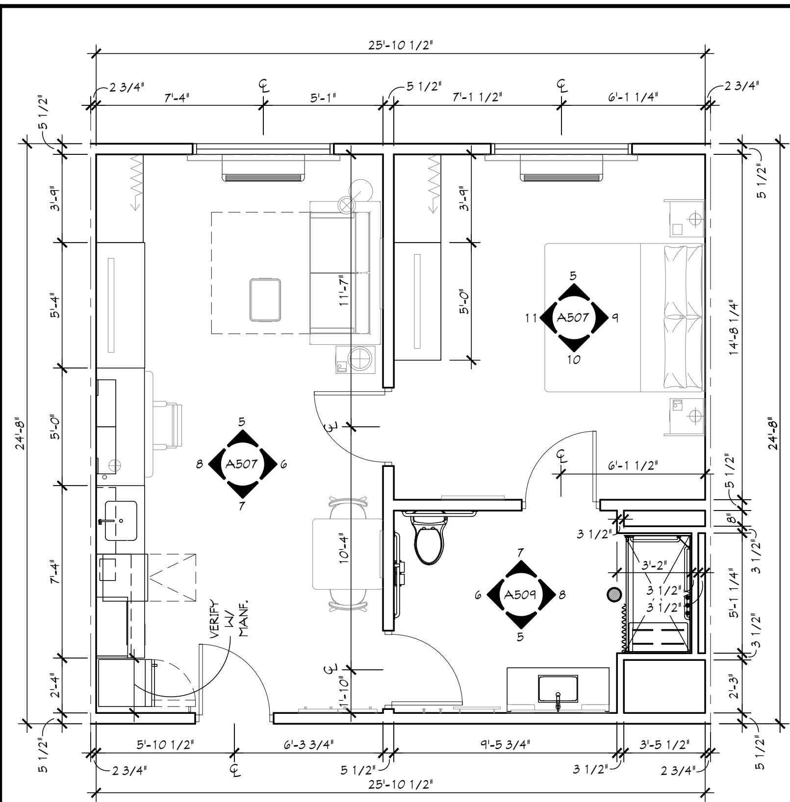
1 ACC. ONE BEDROOM ROLL-IN PLAN SCALE: 1/4" = 1'-0"
