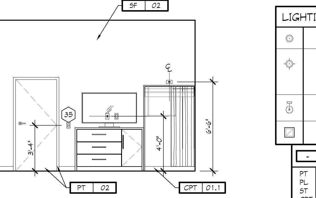
11 ROOM ELEVATION SCALE: 1/4" = 1'-0"
