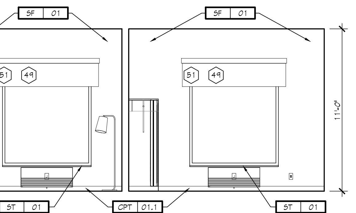
5 ROOM ELEVATION SCALE: 1/4" = 1'-0"
