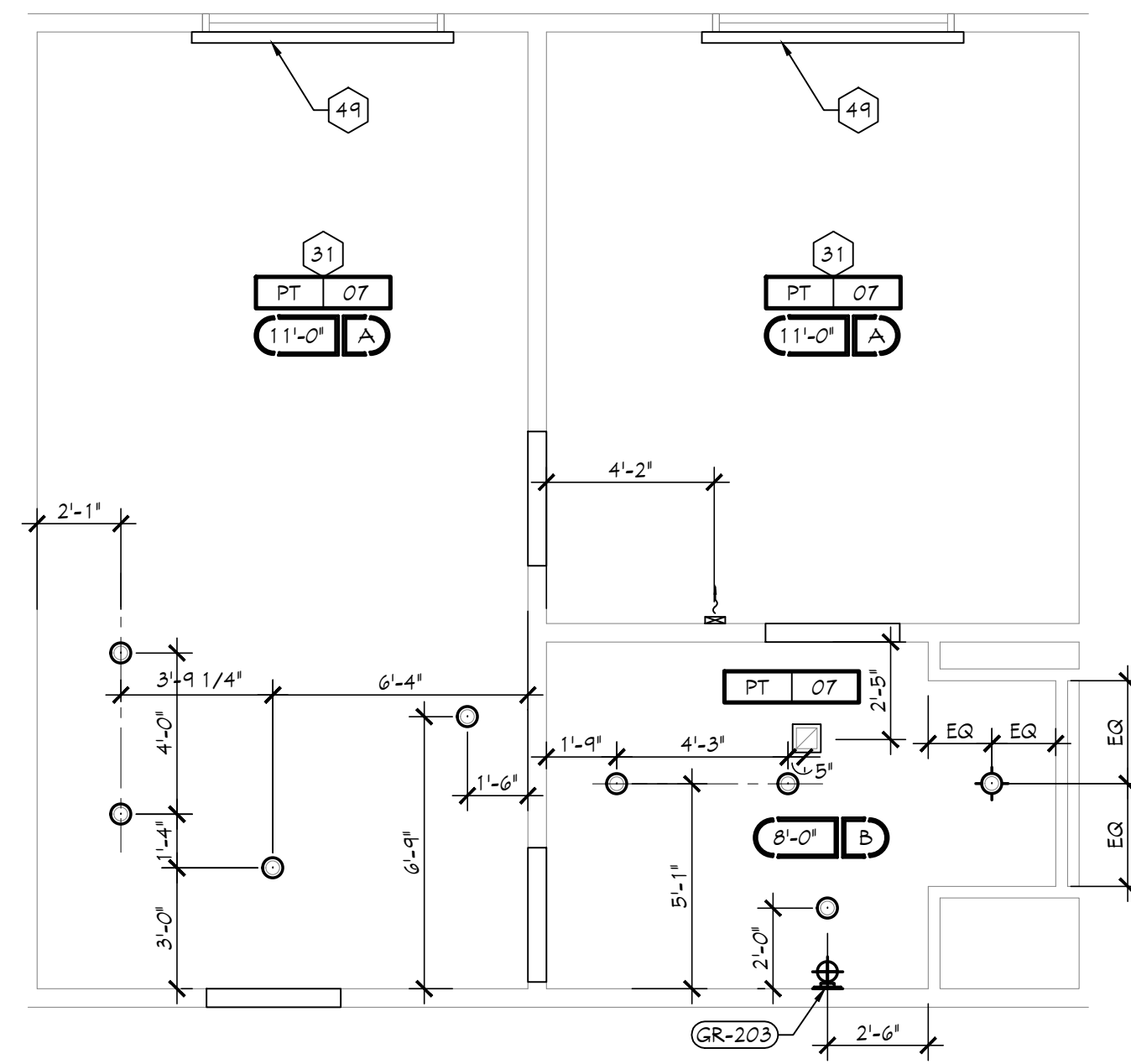
3 ACC. ONE BEDROOM ROLL-IN CEILING SCALE: 1/4" = 1'-0"
