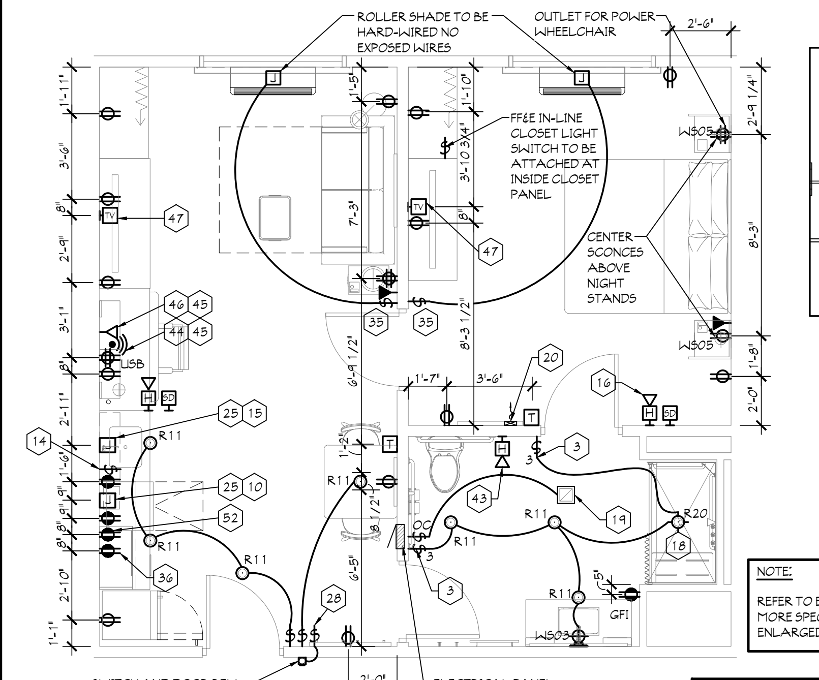
1 ACC. ONE BEDROOM ROLL-IN PLAN SCALE: 1/4" = 1'-0"
