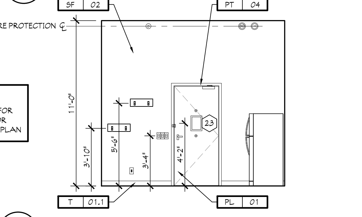
7 ROOM ELEVATION SCALE: 1/4" = 1'-0"
