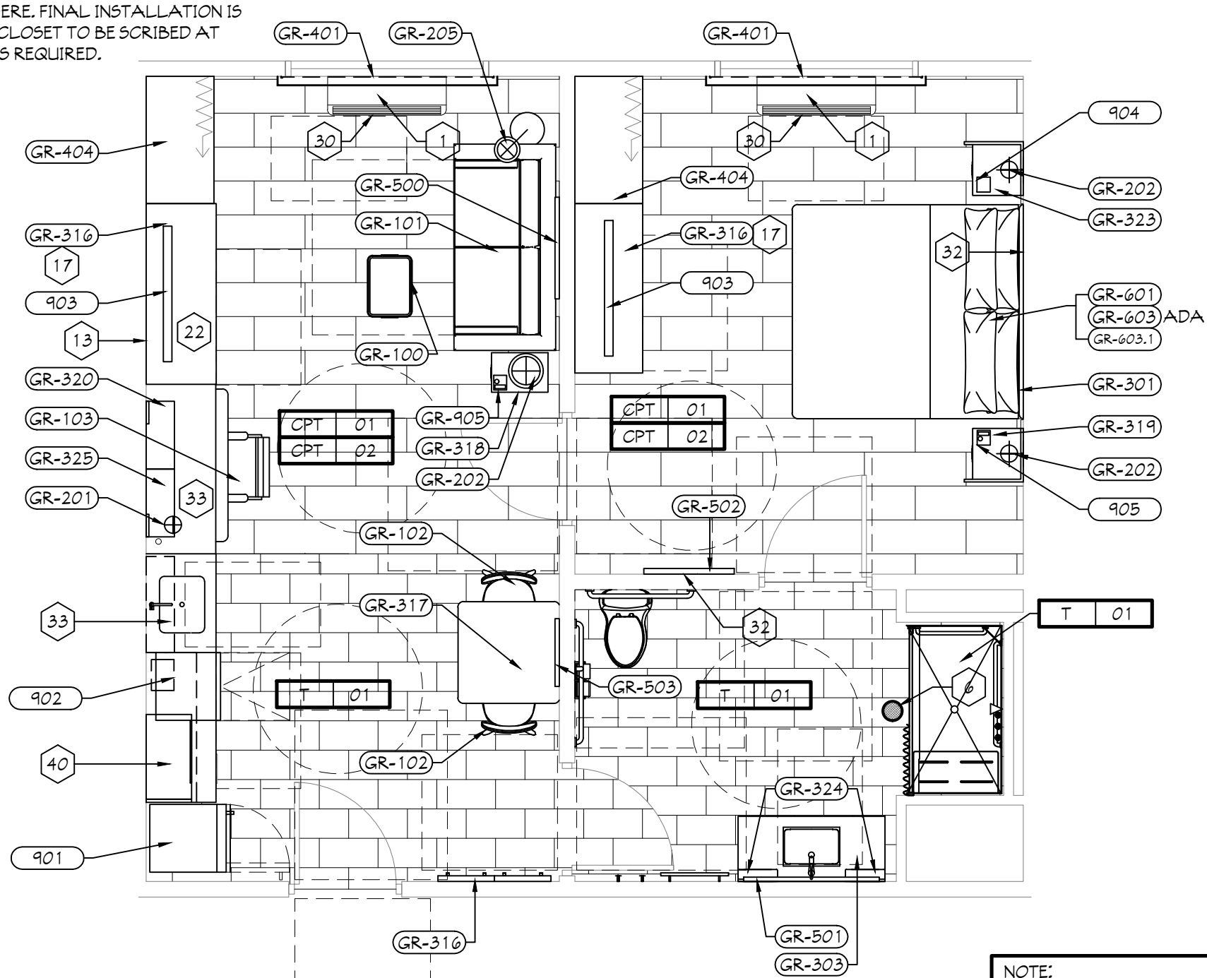
2 ACC. ONE BEDROOM ROLL-IN FF&E SCALE: 1/4" = 1'-0"
