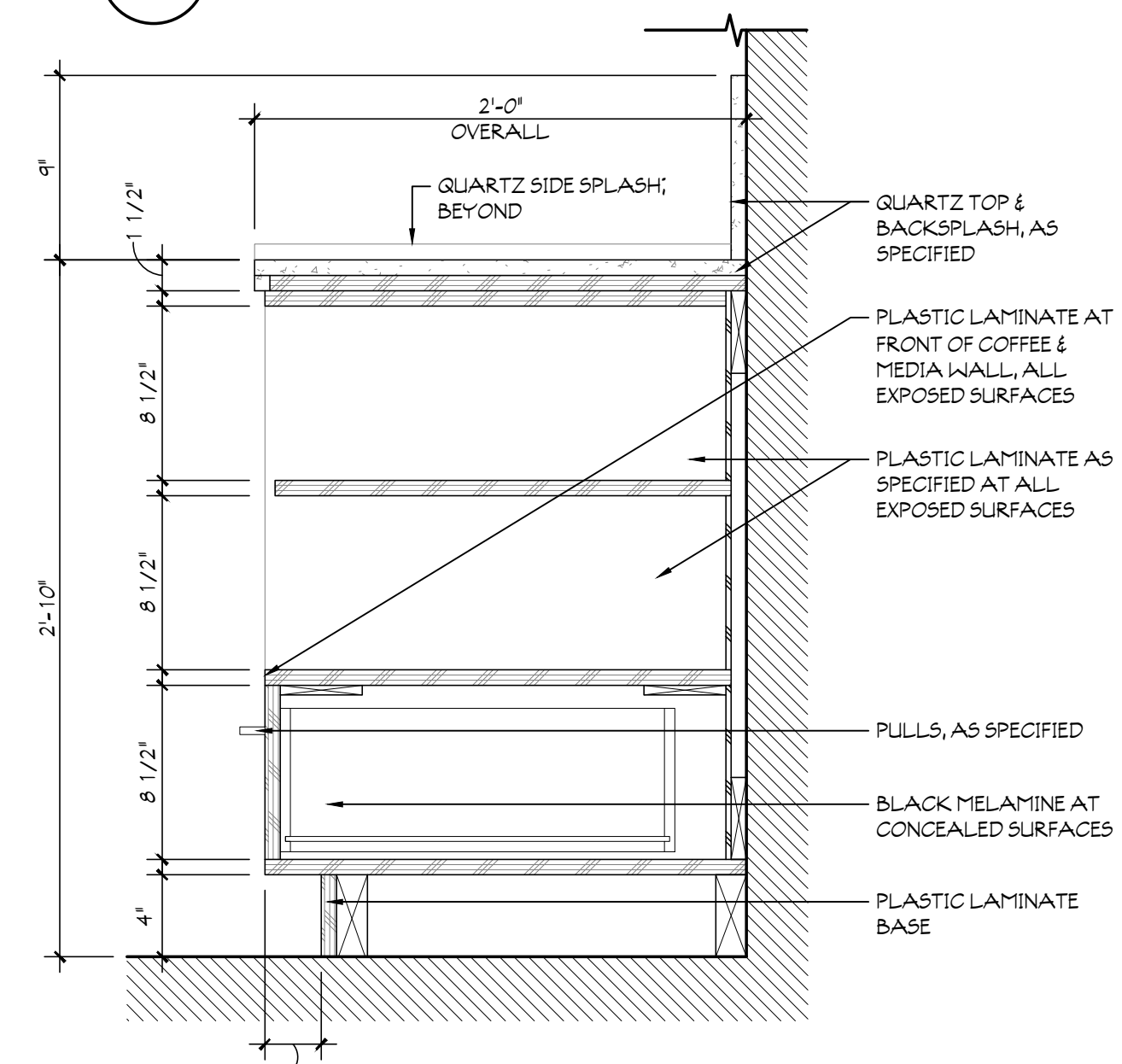
9 DETAIL - COFFEE/MEDIA-SHELVES SCALE: 1 1/2" = 1'-0"
