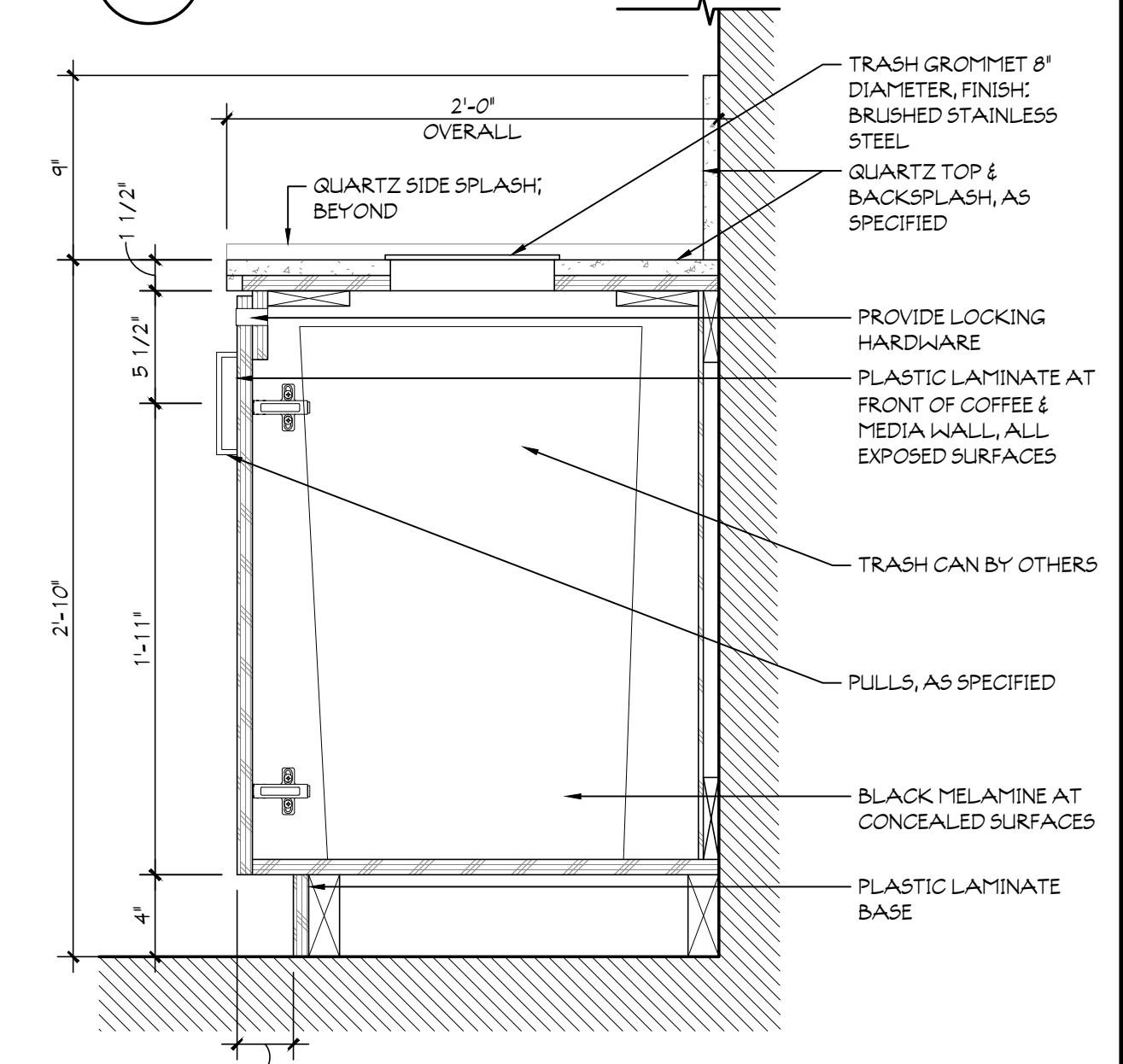
10 DETAIL - COFFEE/MEDIA-TRASH SCALE: 1 1/2" = 1'-0"
