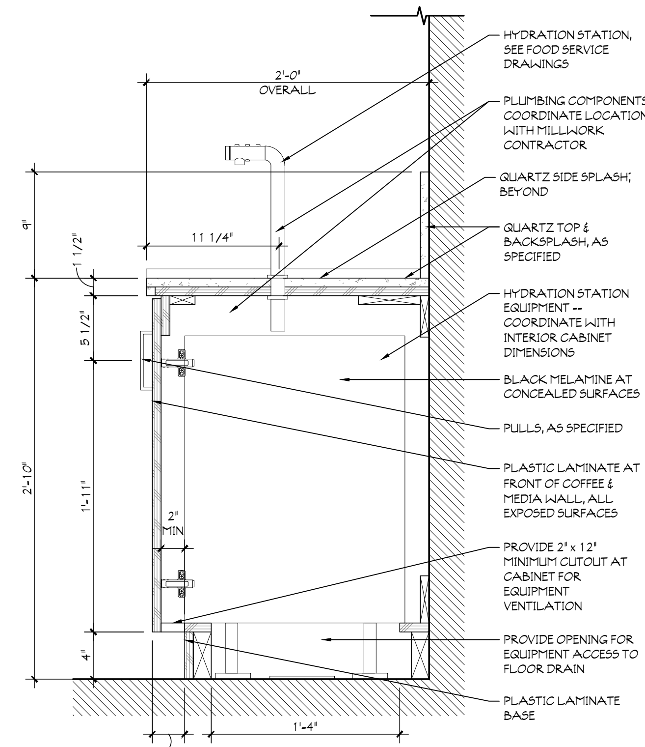
7 DETAIL - HYDRATION STATION SCALE: 1 1/2" = 1'-0"
