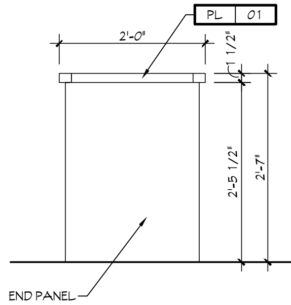
3 ELEVATION SCALE: 3/4" = 1'-0" SALES OFFICE
