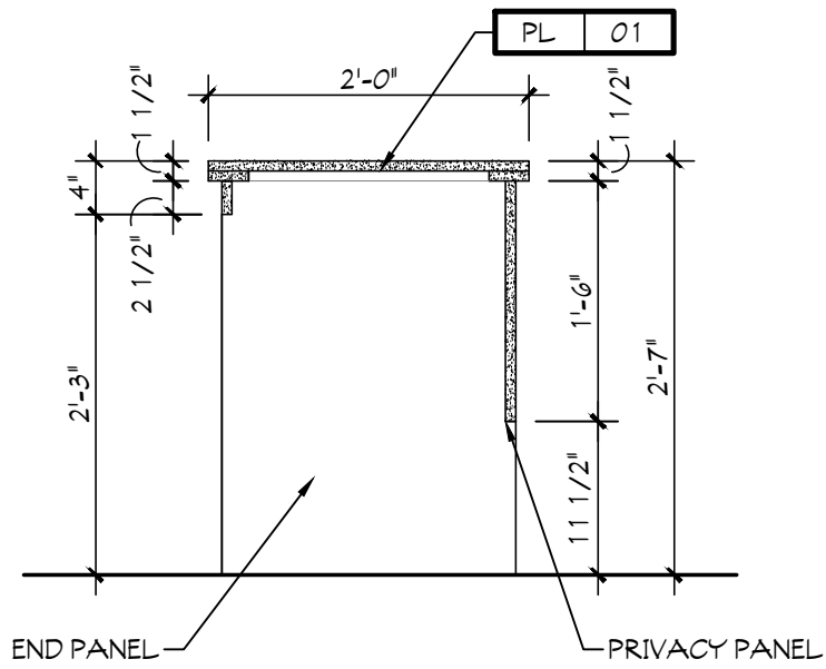
2 SECTION SCALE: 3/4" = 1'-0" SALES OFFICE
