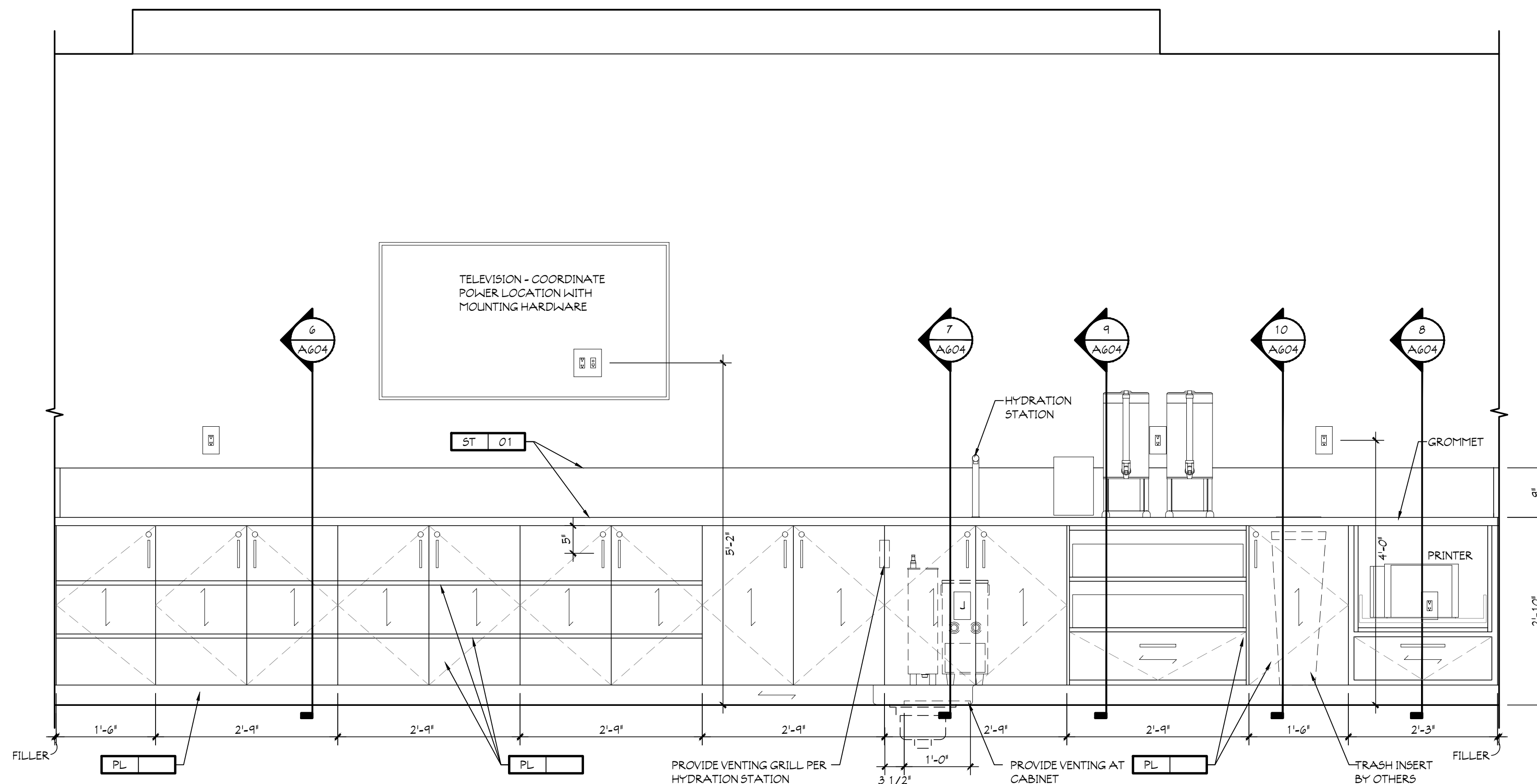
5 MEDIA WALL AND COFFEE BAR SCALE: 3/4" = 1'-0" ELEVATION
