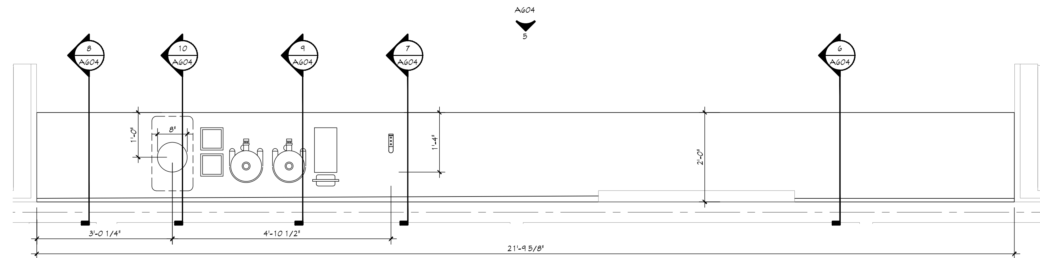
1 ELEVATION SCALE: 3/4" = 1'-0" SALES OFFICE
