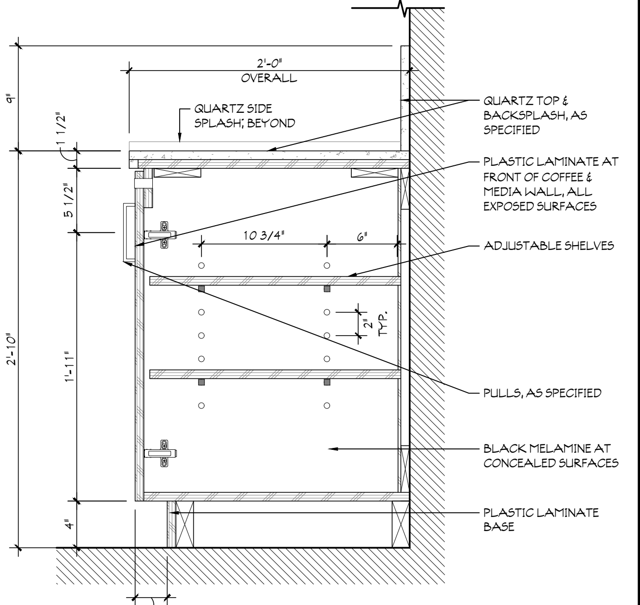
6 DETAIL - COFFEE/MEDIA-DOORS SCALE: 1 1/2" = 1'-0"
