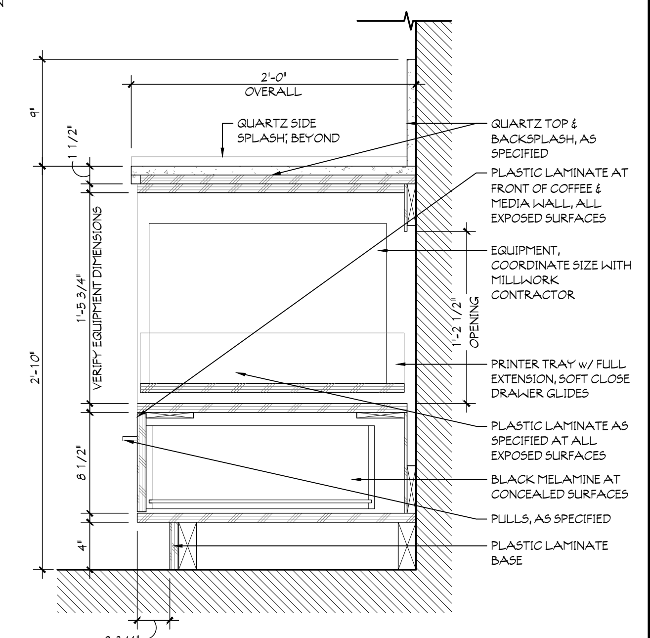
8 DETAIL - COFFEE/MEDIA-PRINTER SCALE: 1 1/2" = 1'-0"
