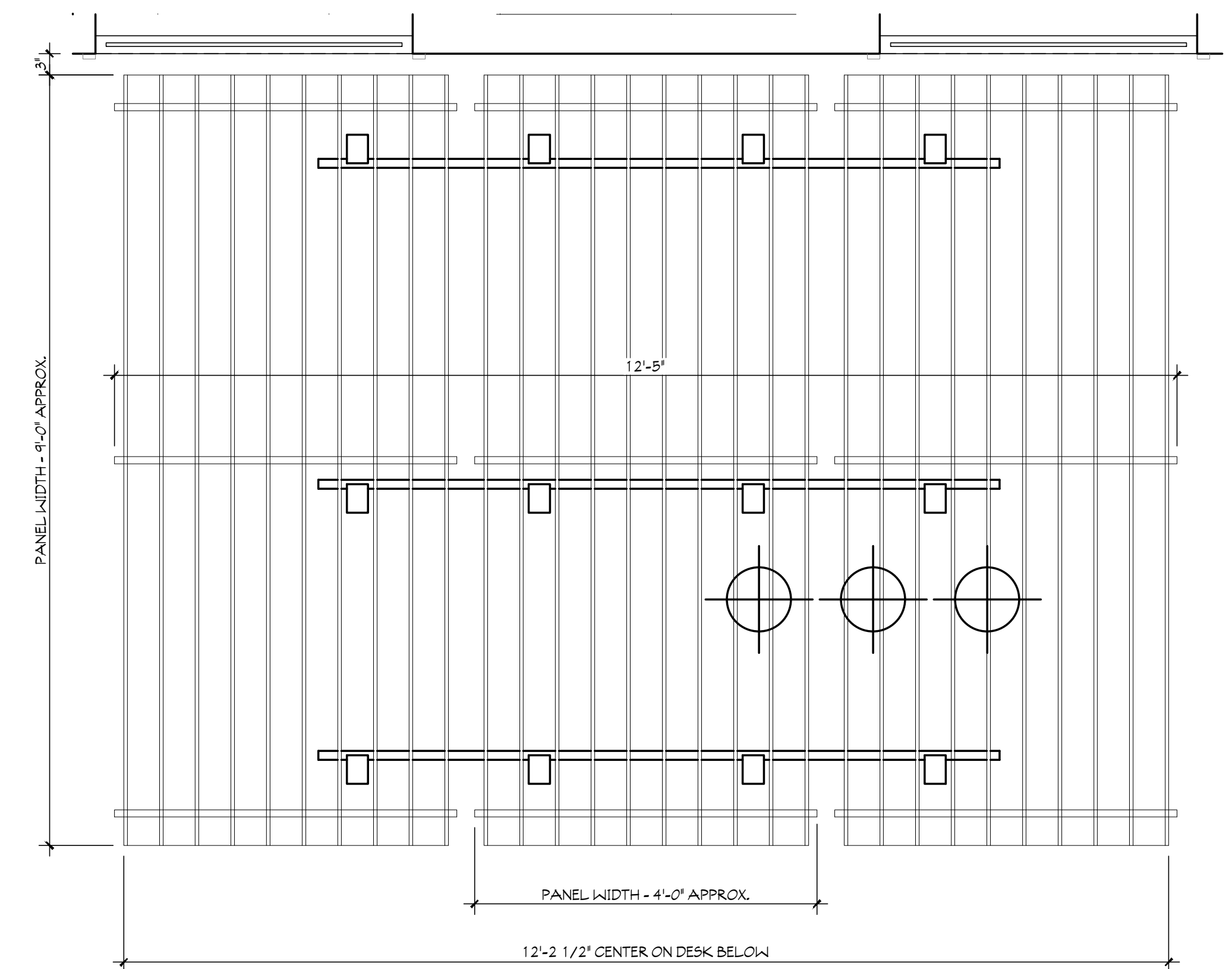
1 RCP - RECEPTION BAFFLE CEILING SCALE: 3/4" = 1'-0"
