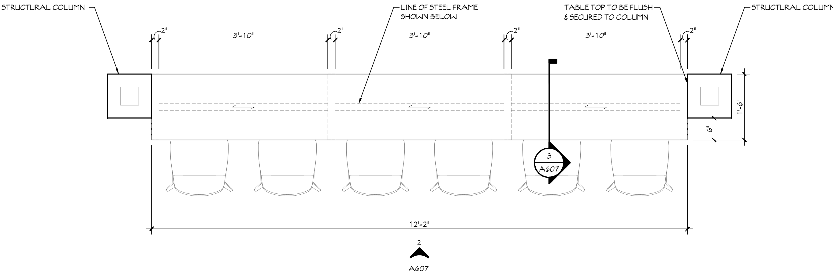
1 BREAKFAST PERCH PLAN SCALE: 3/4" = 1'-0"
