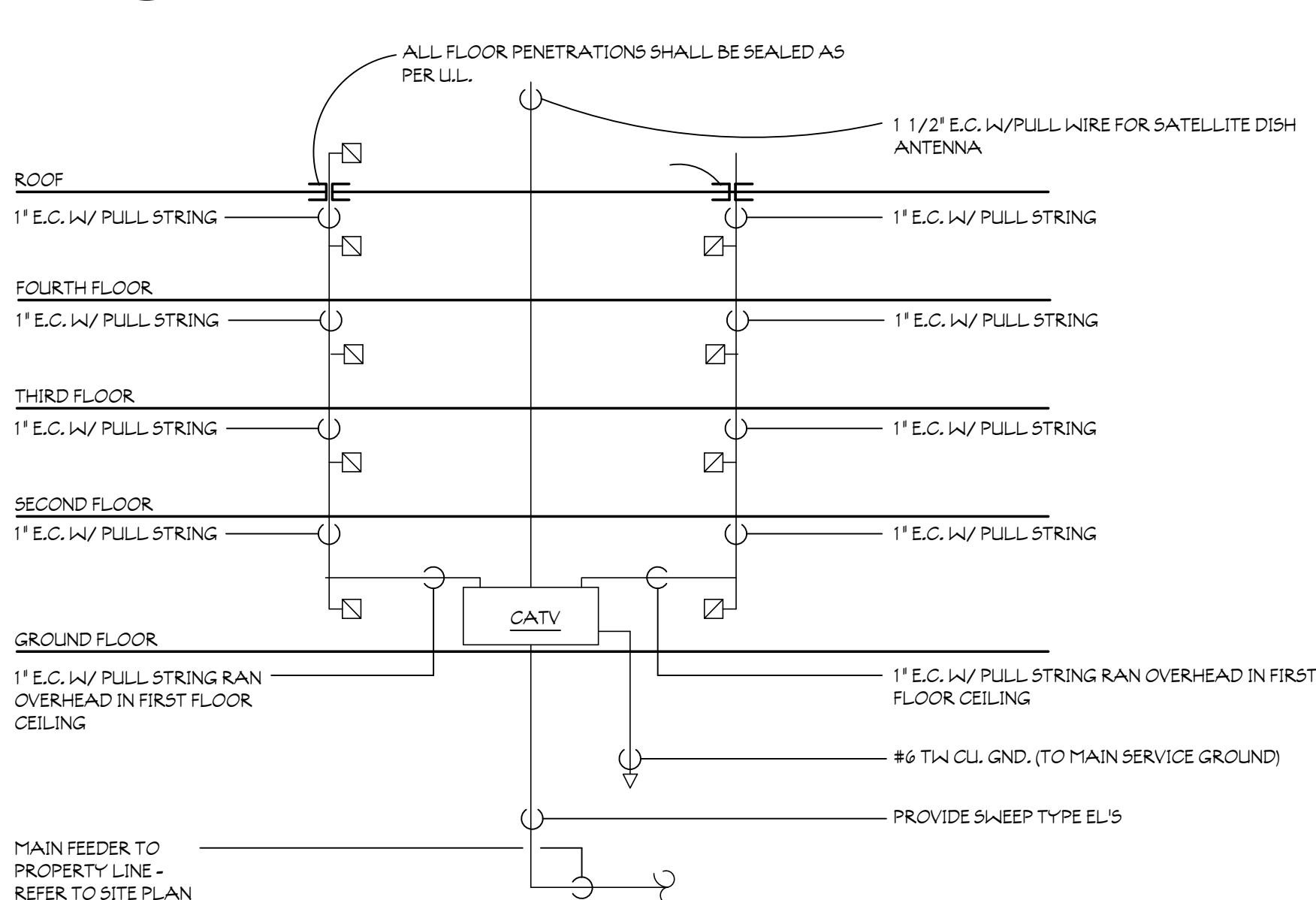
8 TYP. GUEST ROOM CABLE T.V. RISER DIAGRAM SCALE: NOT TO SCALE
