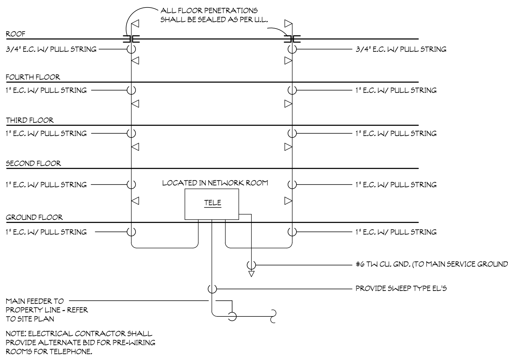
7 TYP. GUEST ROOM TELEPHONE RISER DIAGRAM SCALE: NOT TO SCALE
