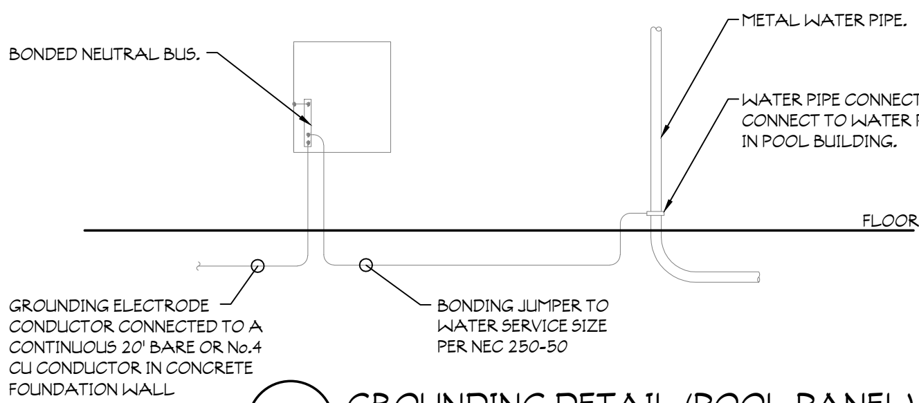
6 GROUNDING DETAIL (POOL PANEL) SCALE: NOT TO SCALE
