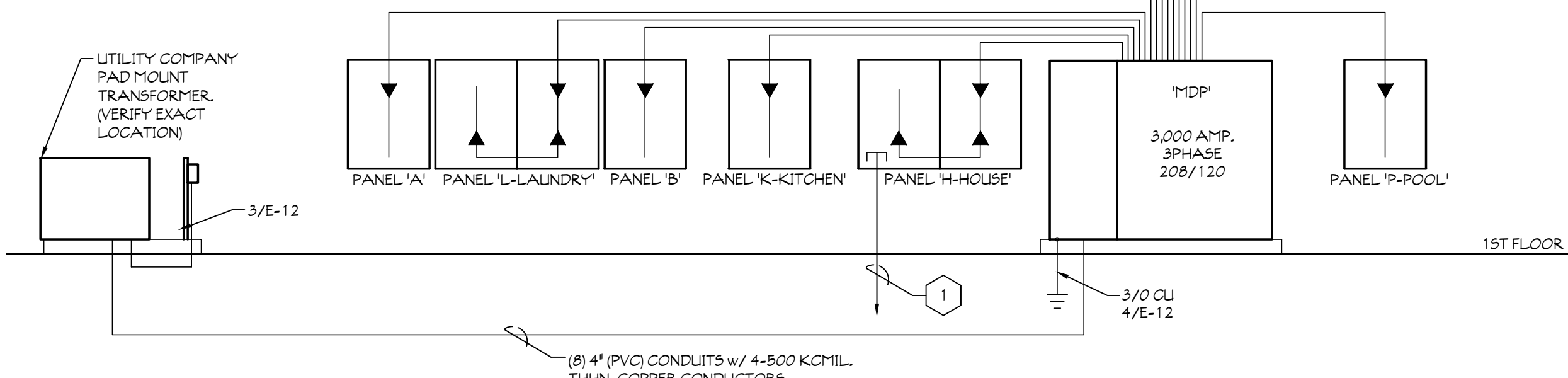
1 POWER RISER DIAGRAM SCALE: NOT TO SCALE
