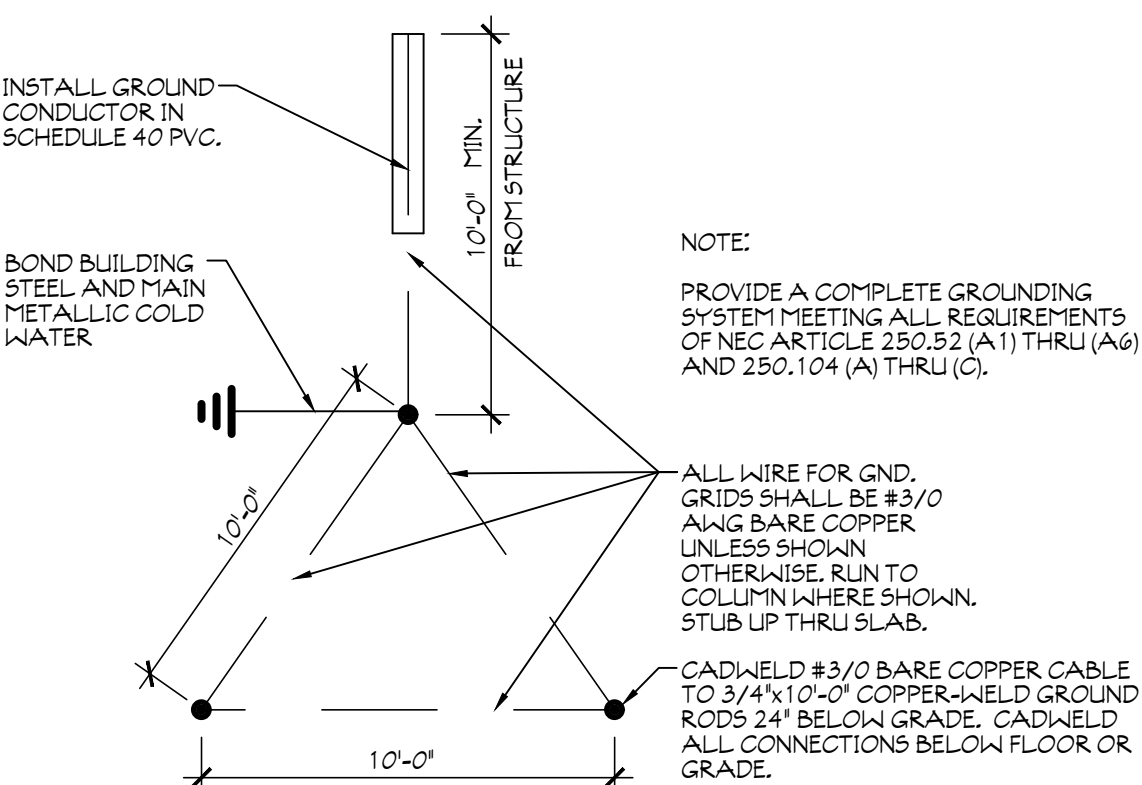
2 GROUNDING DETAIL SCALE: NOT TO SCALE
