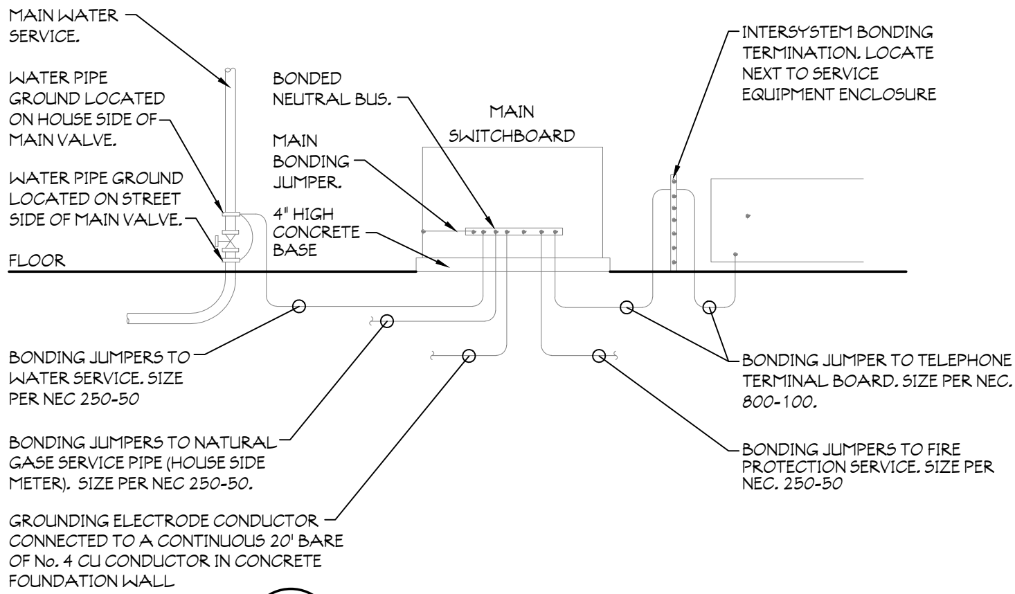
5 SYSTEM GROUNDING DETAIL SCALE: NOT TO SCALE
