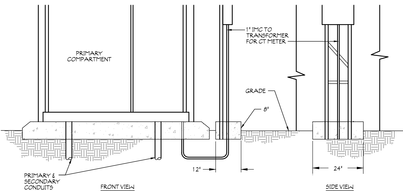
4 TRANSFORMER METER DETAIL SCALE: NOT TO SCALE
