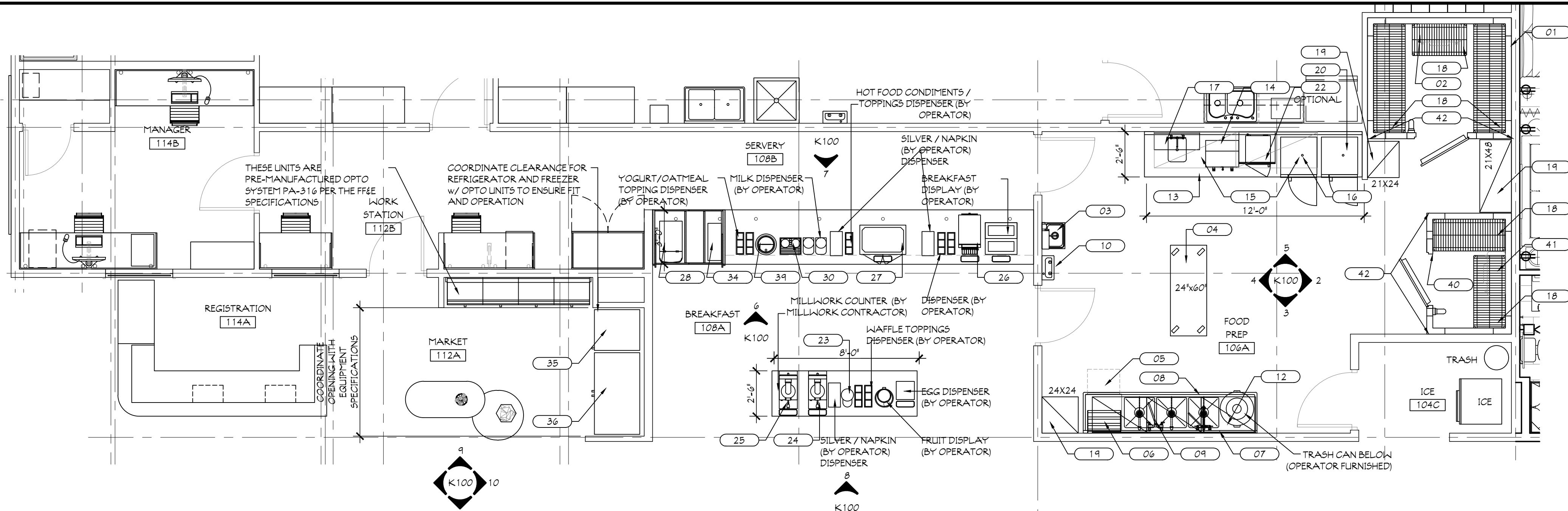
1 ENLARGED EQUIPMENT FLOOR PLAN SCALE: 1/4" = 1'-0"
