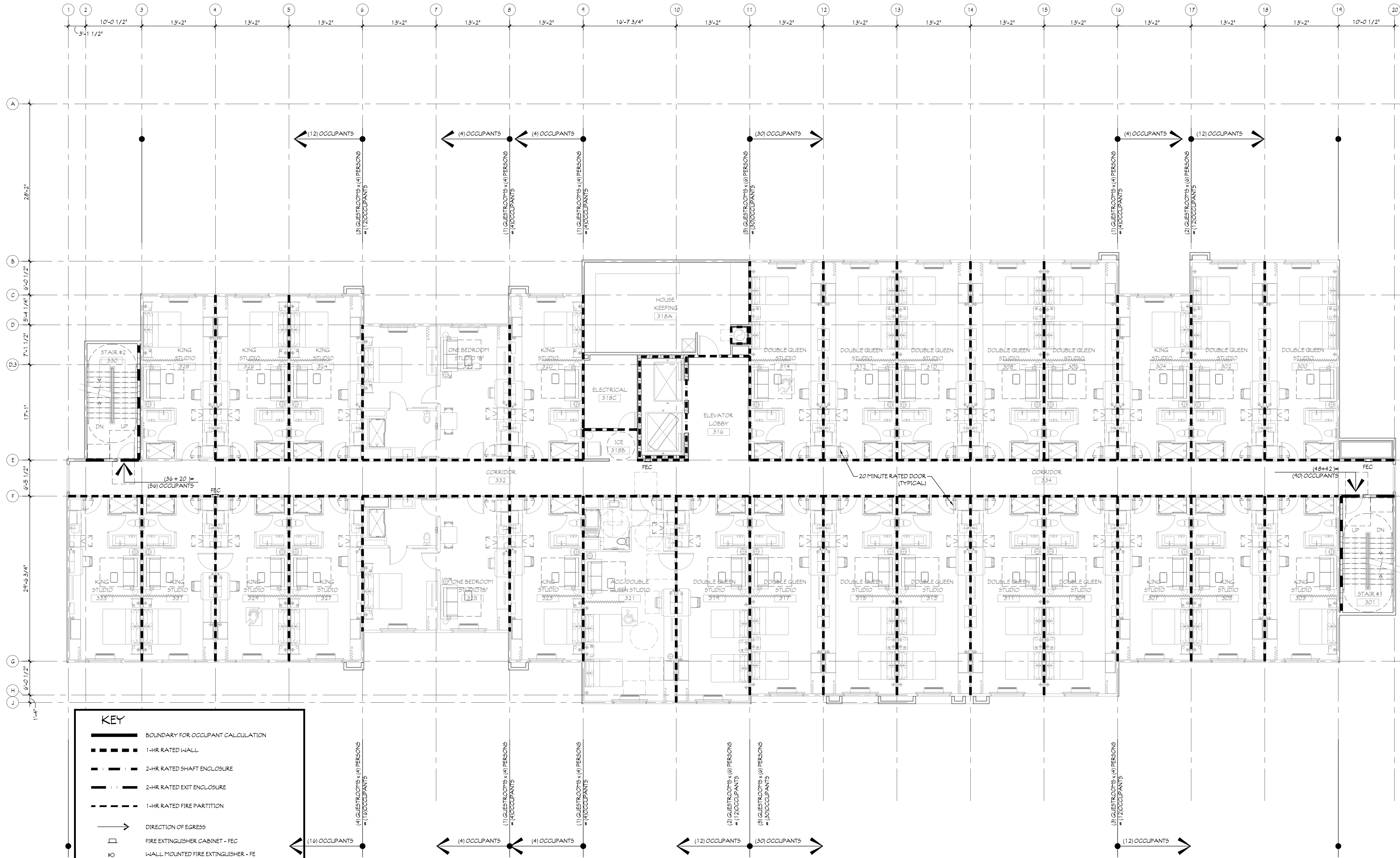
1 THIRD FLOOR LIFE SAFETY PLAN SCALE: 1/8" = 1'-0"
