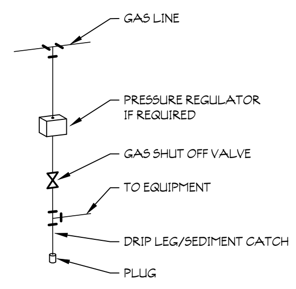
2 GAS LINE DROP TO EQUIPMENT DETAIL SCALE: NOT TO SCALE
