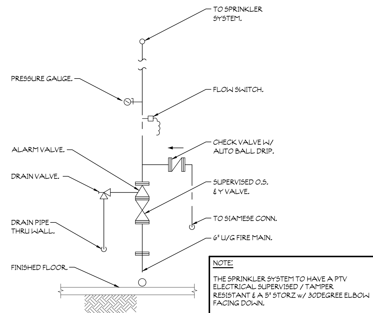
4 TYPICAL WET PIPE SPRINKLER RISER SCALE: NOT TO SCALE
