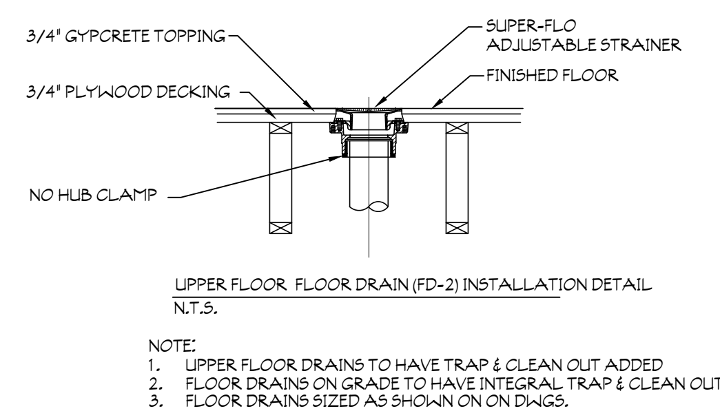
6 FLOOR DRAIN DETAIL SCALE: NOT TO SCALE
