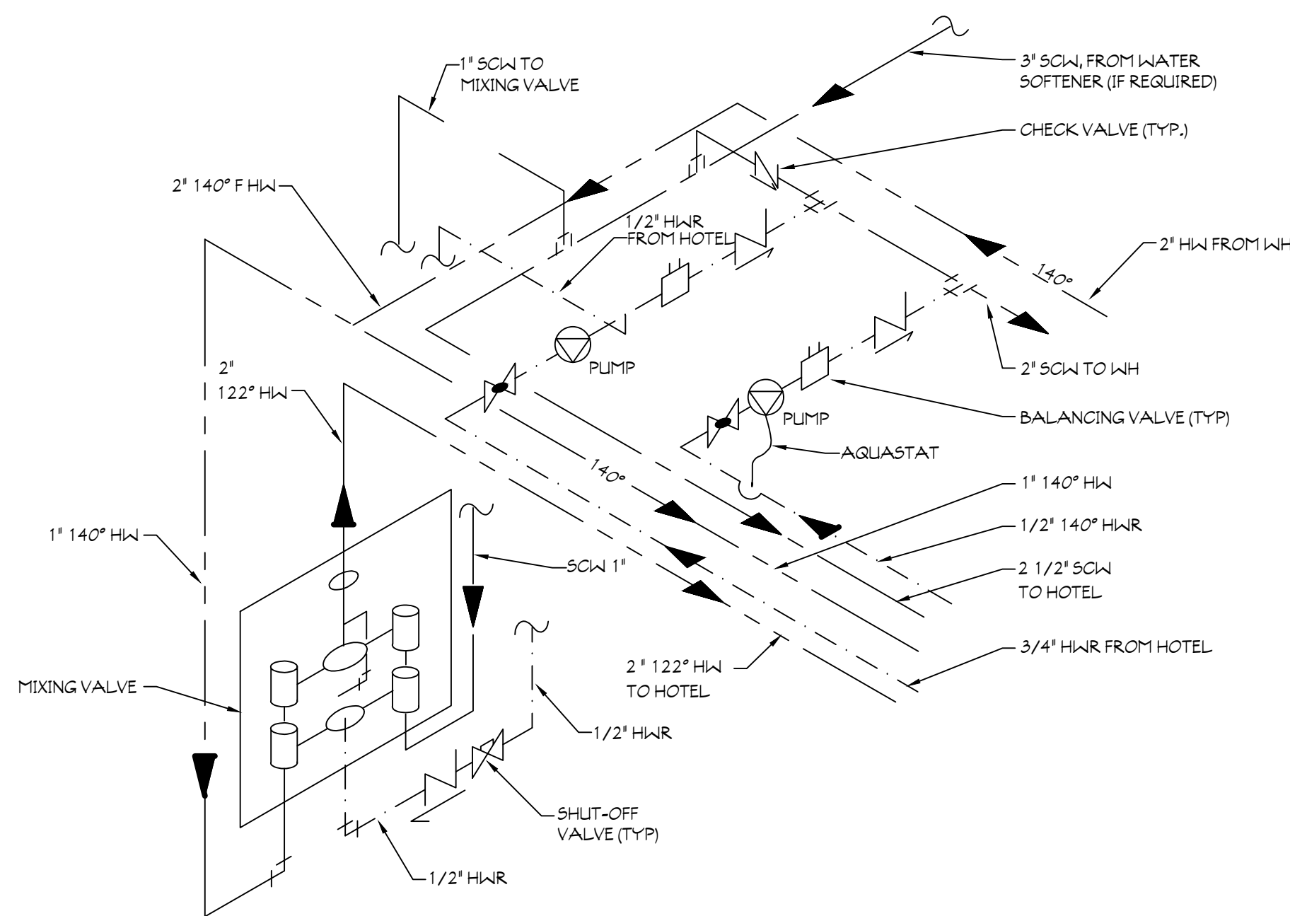
1 TMV & HOT WATER RETURN DIAGRAM SCALE: NOT TO SCALE
