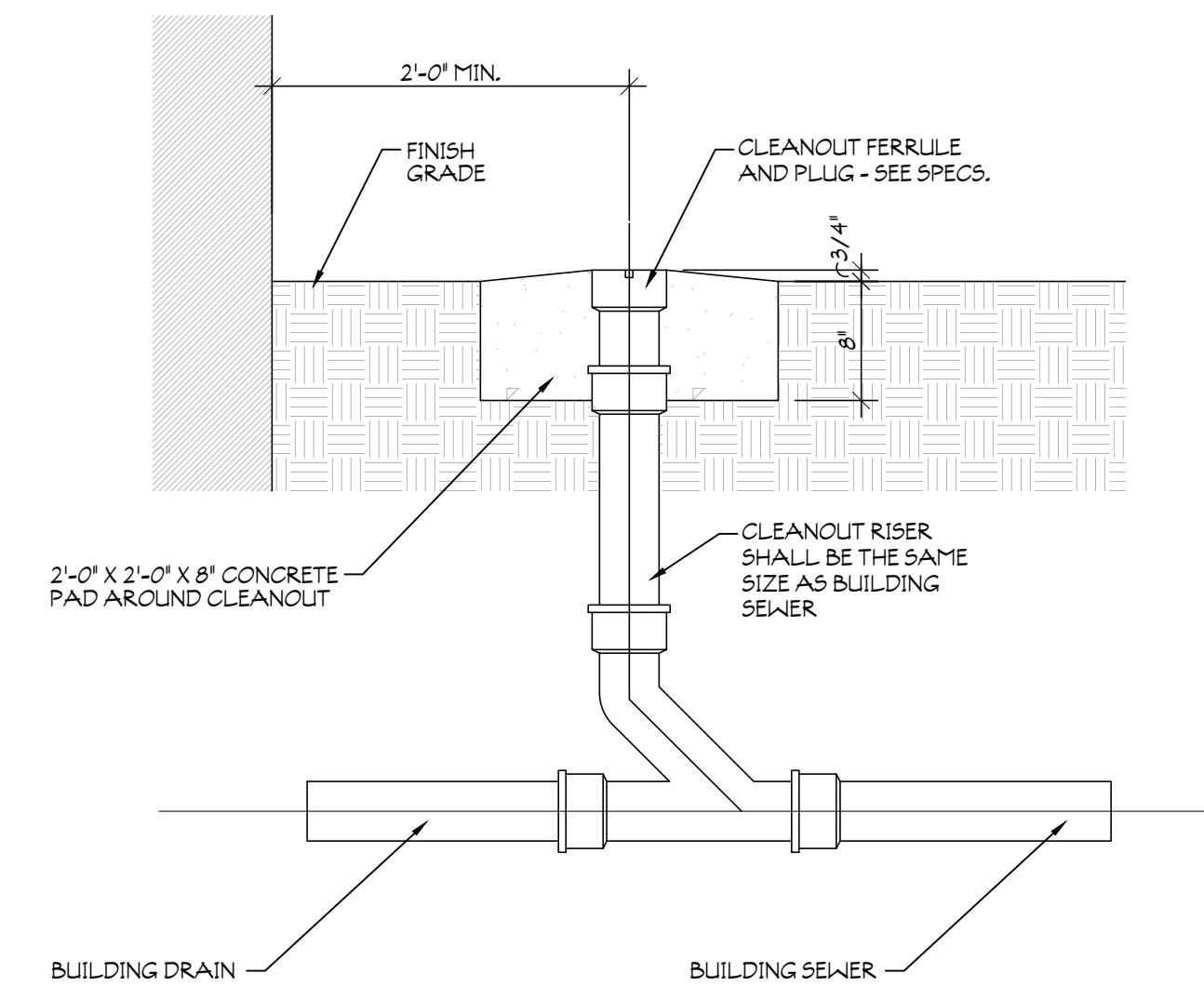
7 TYPICAL EXTERIOR CLEANOUT SCALE: NOT TO SCALE
