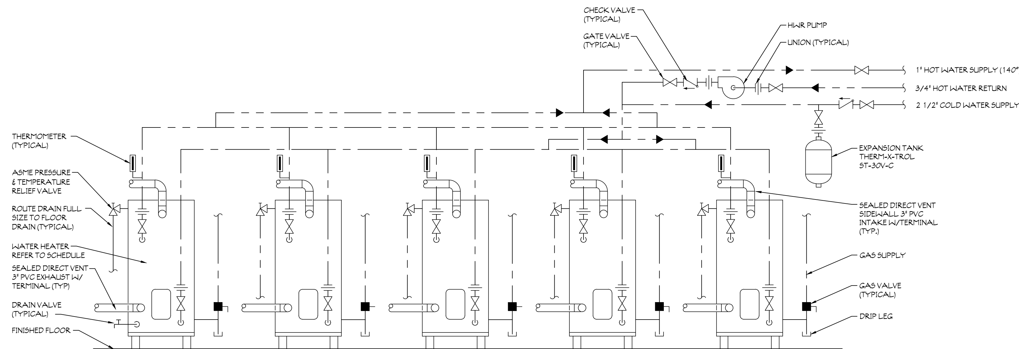
2 WATER HEATER PIPING DETAIL SCALE: NOT TO SCALE
