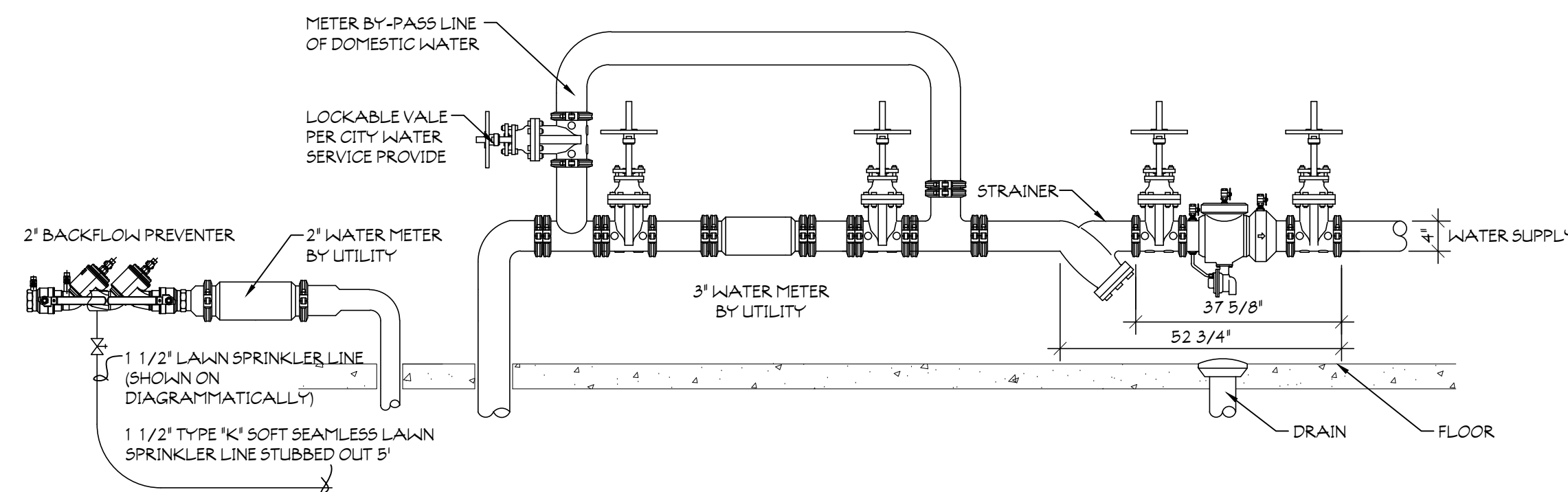
8 TYPICAL 2" LAWN SPRINKLER RISER SCALE: NOT TO SCALE
