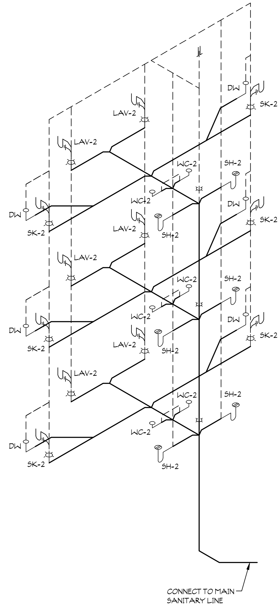
2 SANITARY RISER DIAGRAM SCALE: NOT TO SCALE
