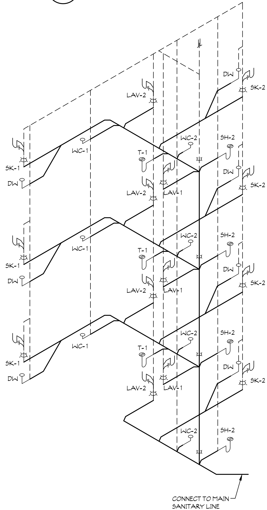
6 SANITARY RISER DIAGRAM SCALE: NOT TO SCALE
