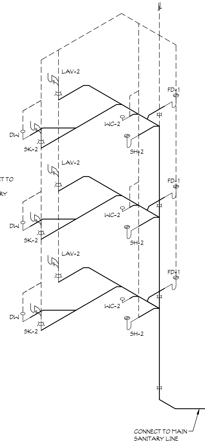
11 SANITARY RISER DIAGRAM SCALE: NOT TO SCALE
