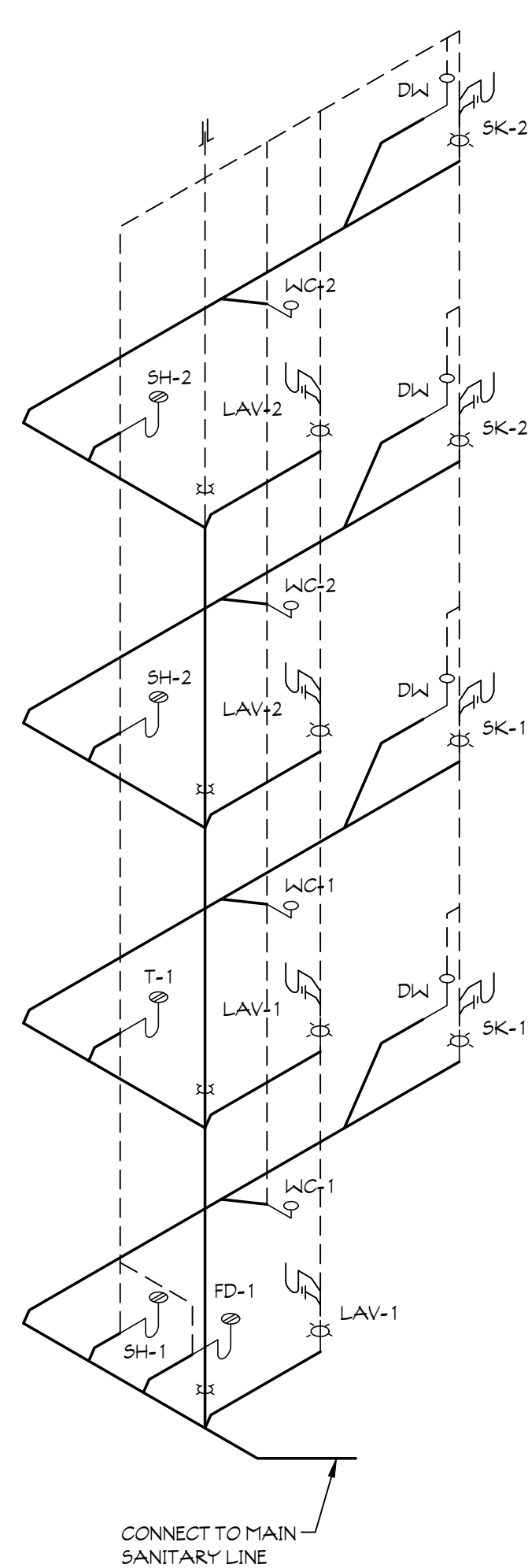
7 SANITARY RISER DIAGRAM SCALE: NOT TO SCALE
