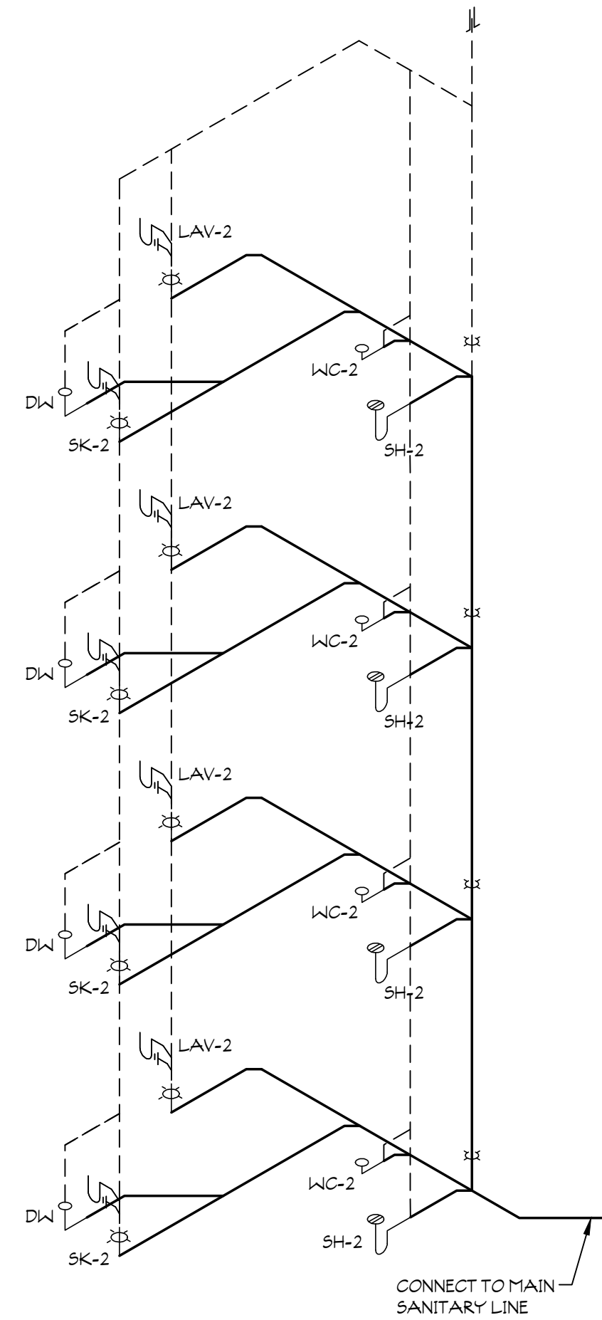
3 SANITARY RISER DIAGRAM SCALE: NOT TO SCALE
