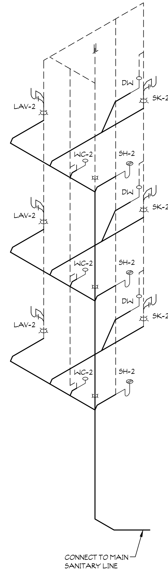
4 SANITARY RISER DIAGRAM SCALE: NOT TO SCALE
