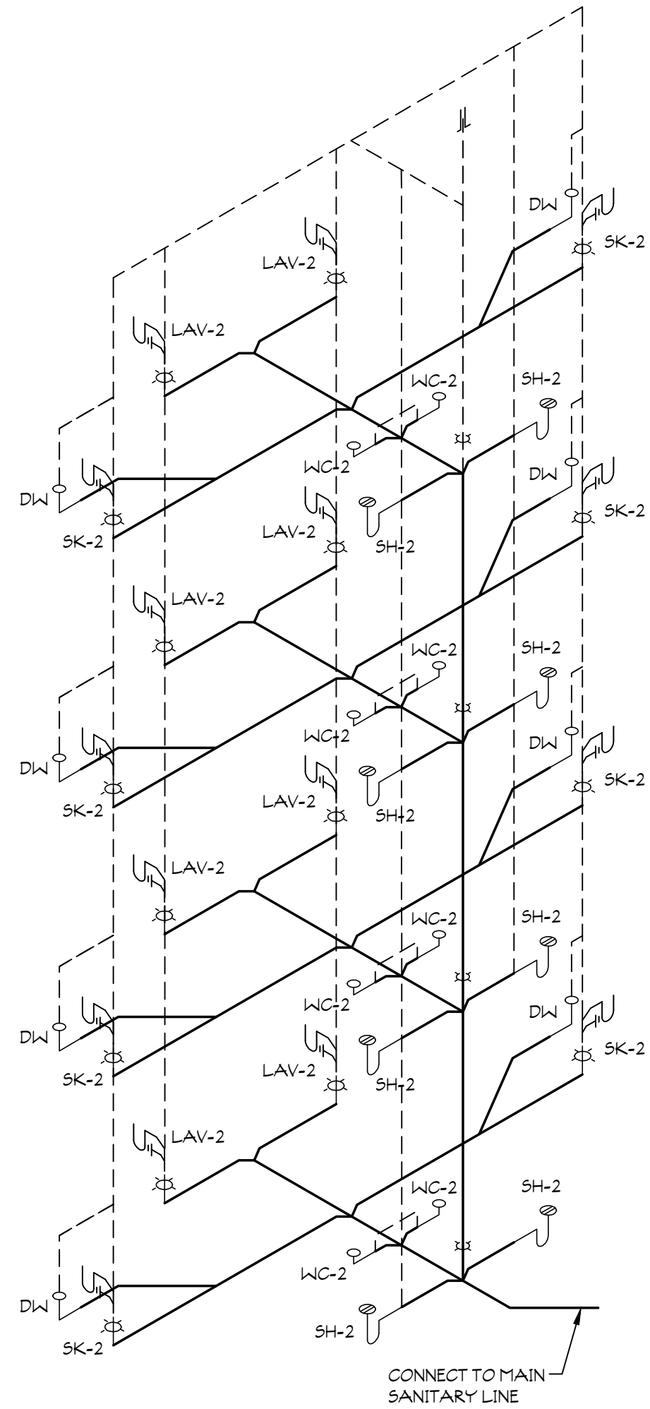
1 SANITARY RISER DIAGRAM SCALE: NOT TO SCALE
