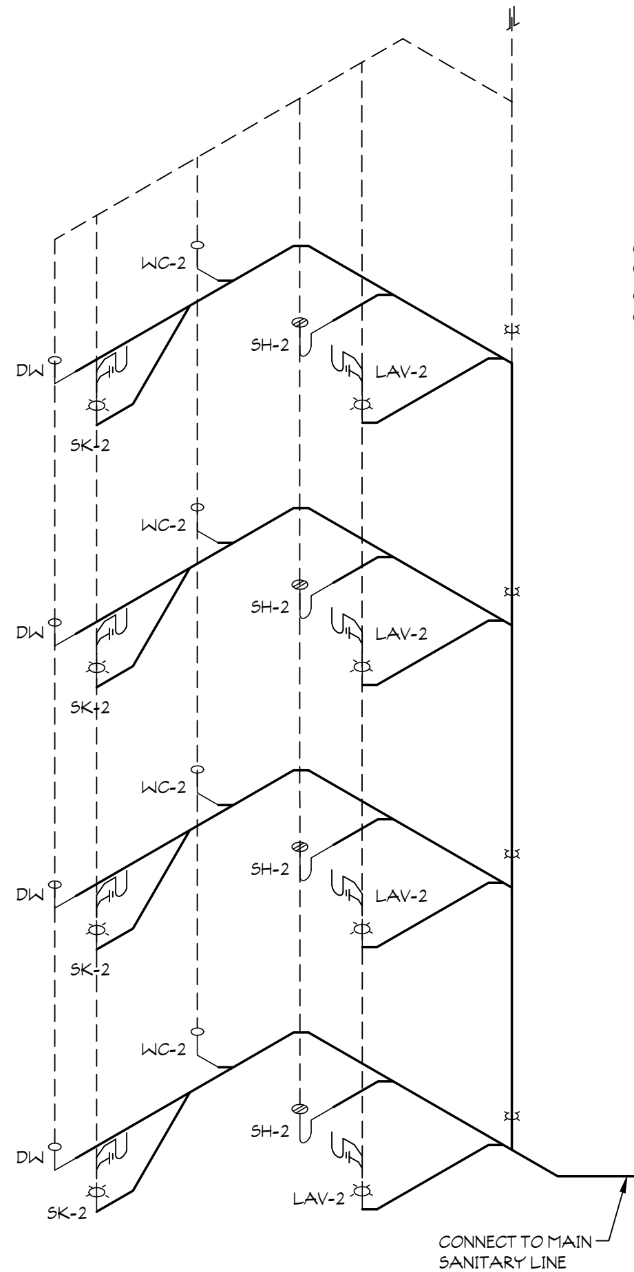
8 SANITARY RISER DIAGRAM SCALE: NOT TO SCALE
