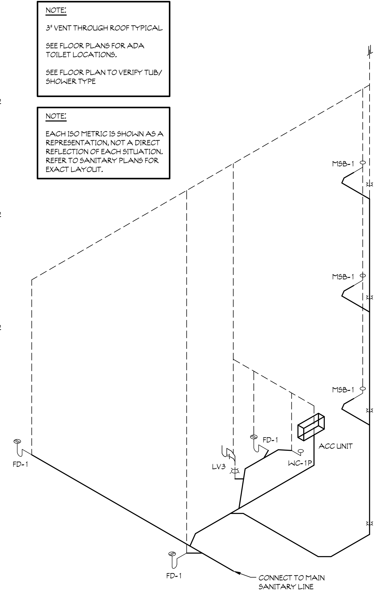
5 SANITARY RISER DIAGRAM SCALE: NOT TO SCALE
