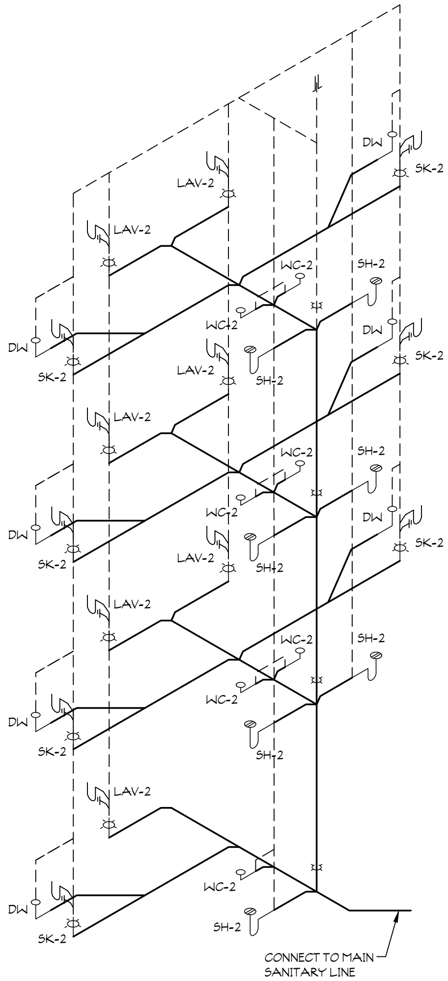
2 SANITARY RISER DIAGRAM SCALE: NOT TO SCALE
