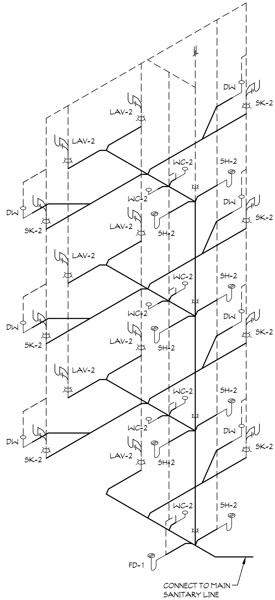
1 SANITARY RISER DIAGRAM SCALE: NOT TO SCALE
