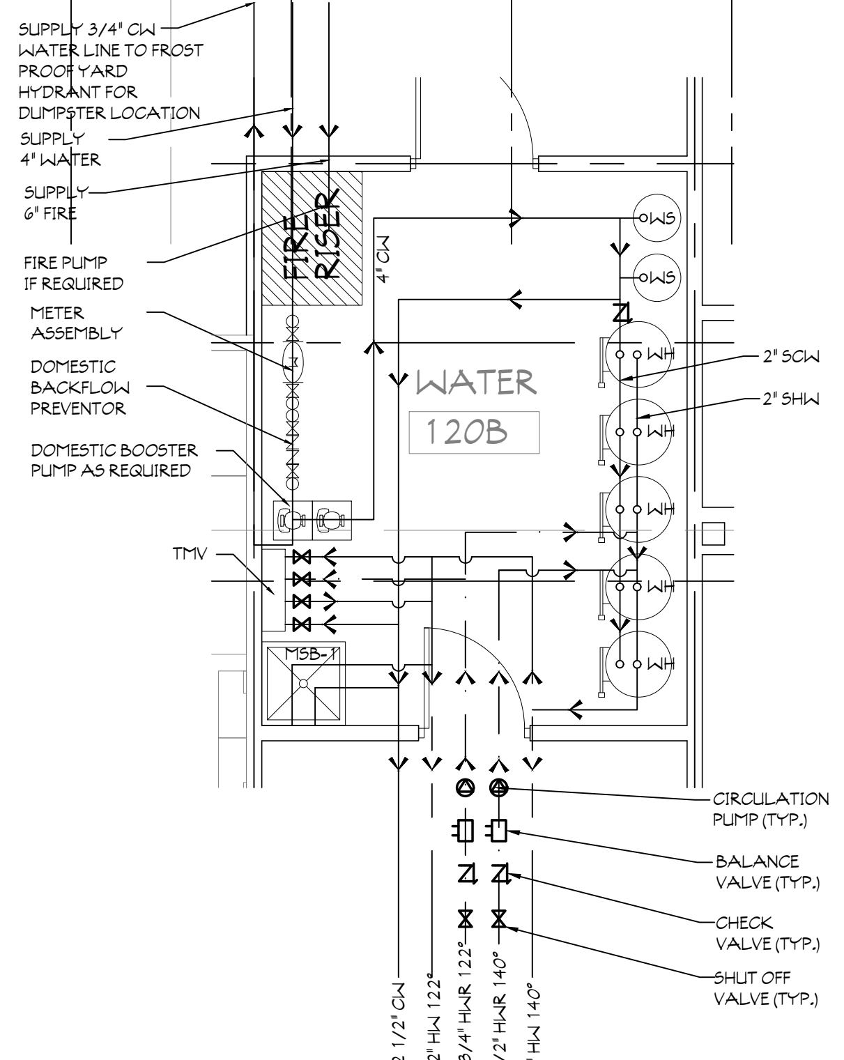
2 WATER ROOM SCALE: 1/4" = 1'-0"
