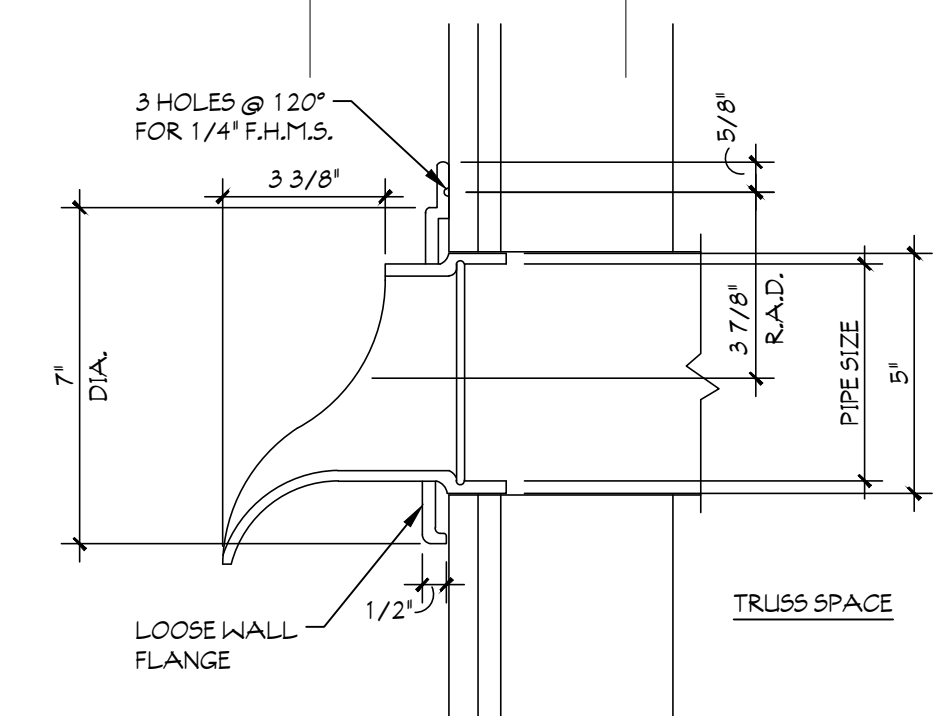
2 OVERFLOW NOZZLE DETAIL SCALE: 3/4" = 1'-0"
