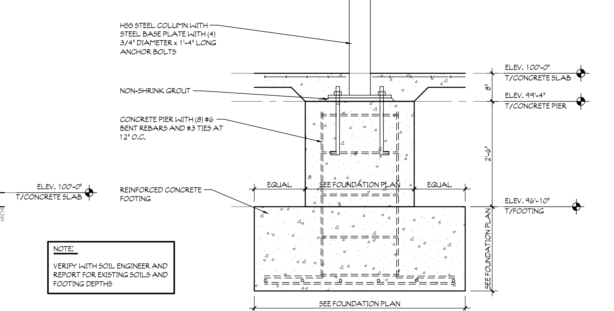
12 CANOPY COLUMN SCALE: 3/4" = 1'-0"
