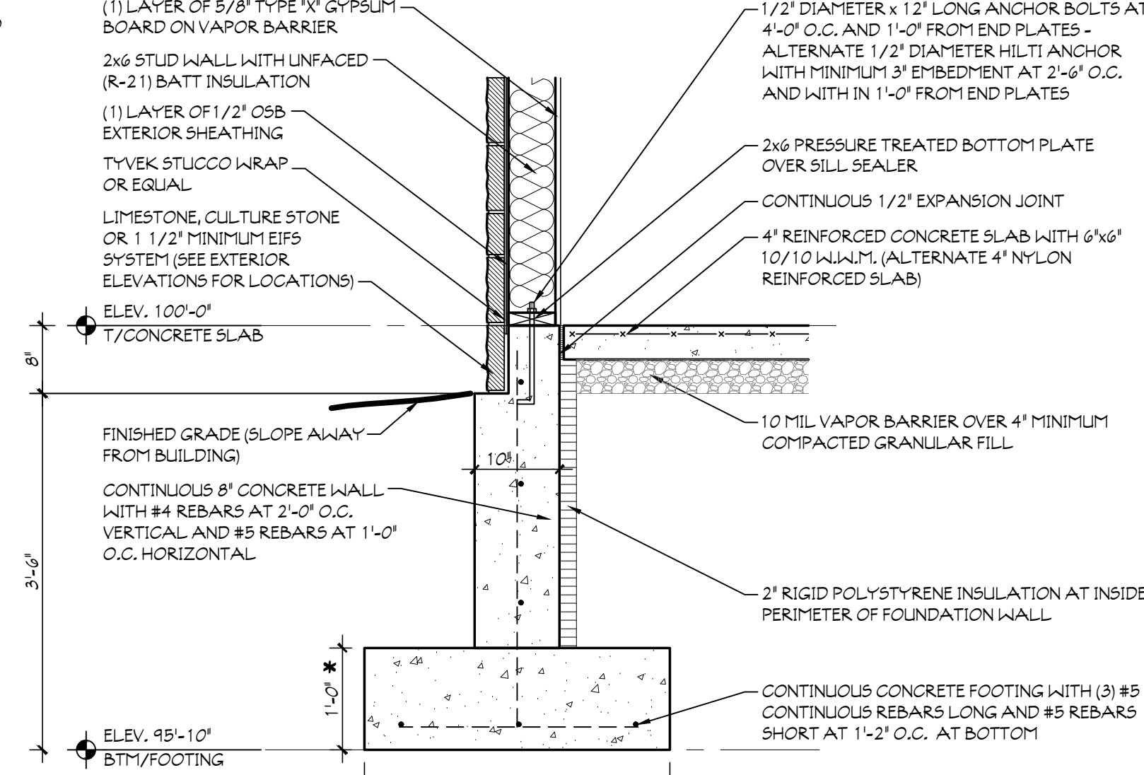
3 FOUNDATION SECTION SCALE: 3/4" = 1'-0"
