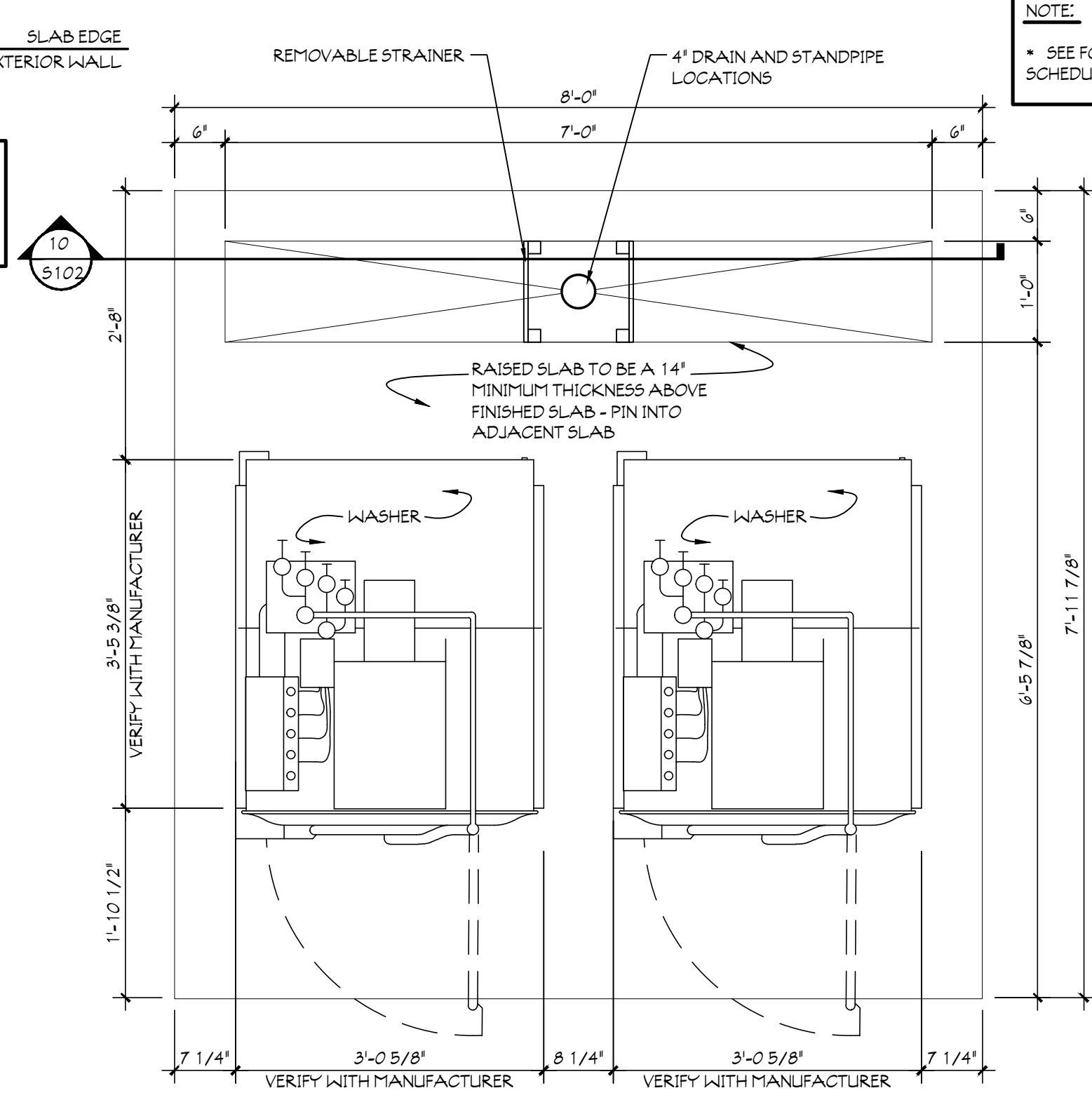
9 WASHER PAD PLAN SCALE: 3/4" = 1'-0"
