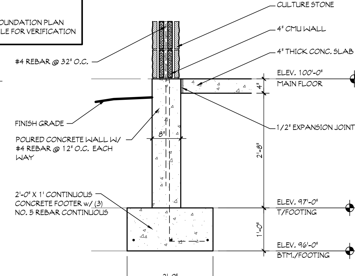
13 PATIO WALL FOOTING SCALE: 3/4" = 1'-0"
