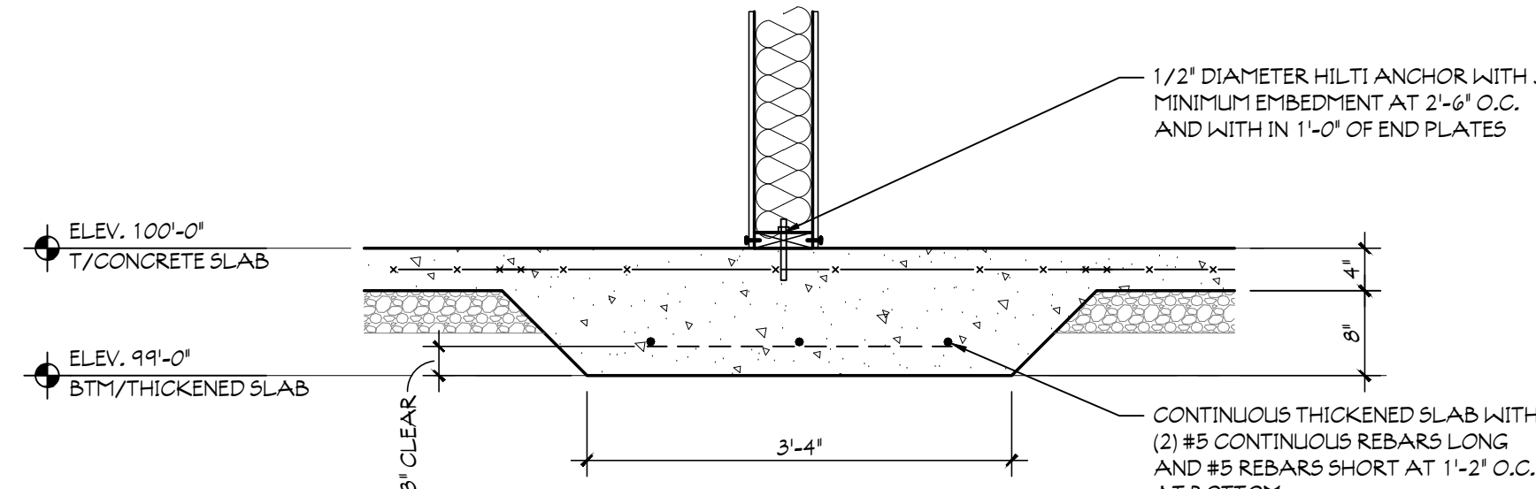
5a THICKENED SLAB SCALE: 3/4" = 1'-0"
