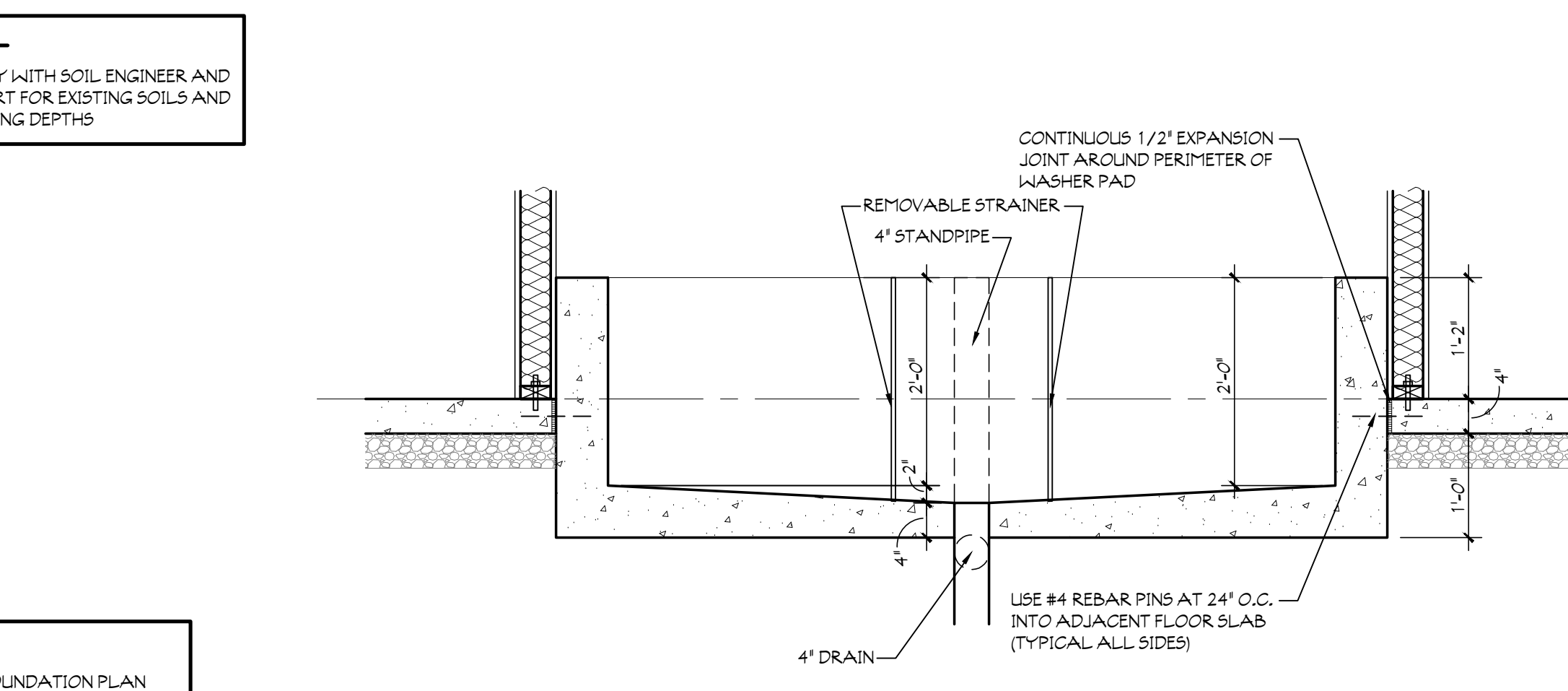
10 WASHER SECTION SCALE: 3/4" = 1'-0"
