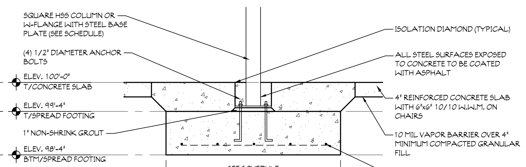
6 SPREAD FOOTING SCALE: 3/4" = 1'-0"
