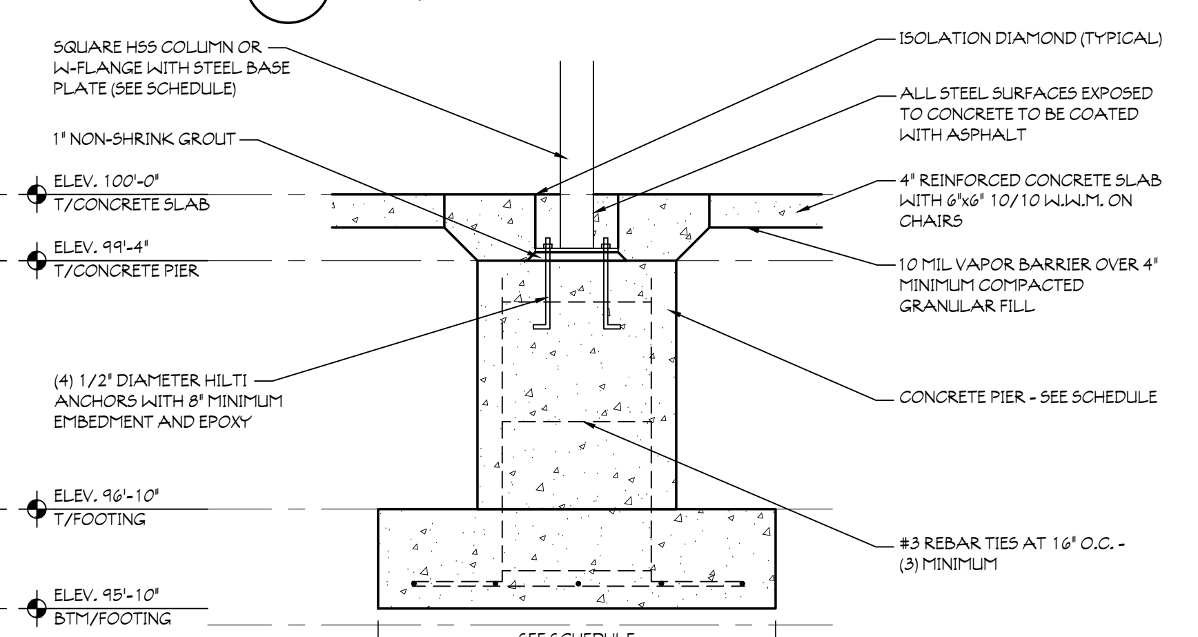
7 PIER/FOOTING SECTION SCALE: 3/4" = 1'-0"
