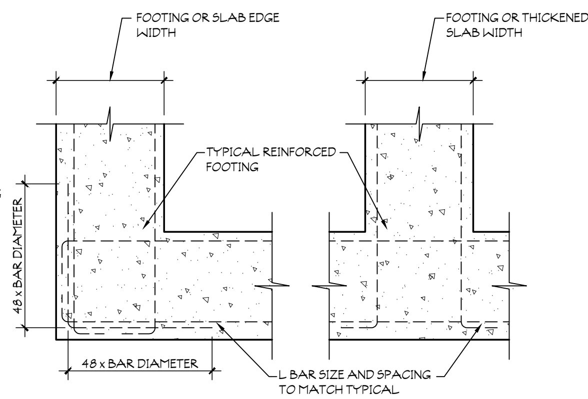
2 FOOTING DETAIL SCALE: 3/4" = 1'-0"
