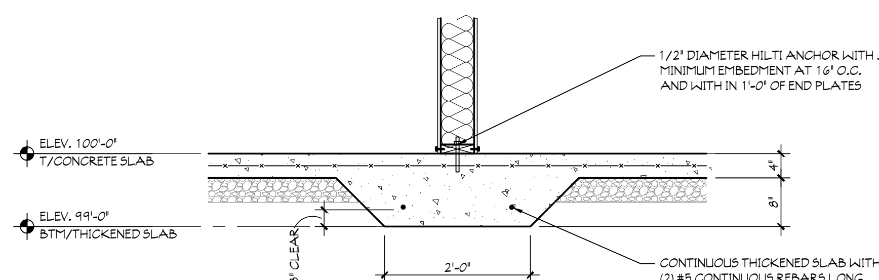
5b THICKENED SLAB SCALE: 3/4" = 1'-0"
