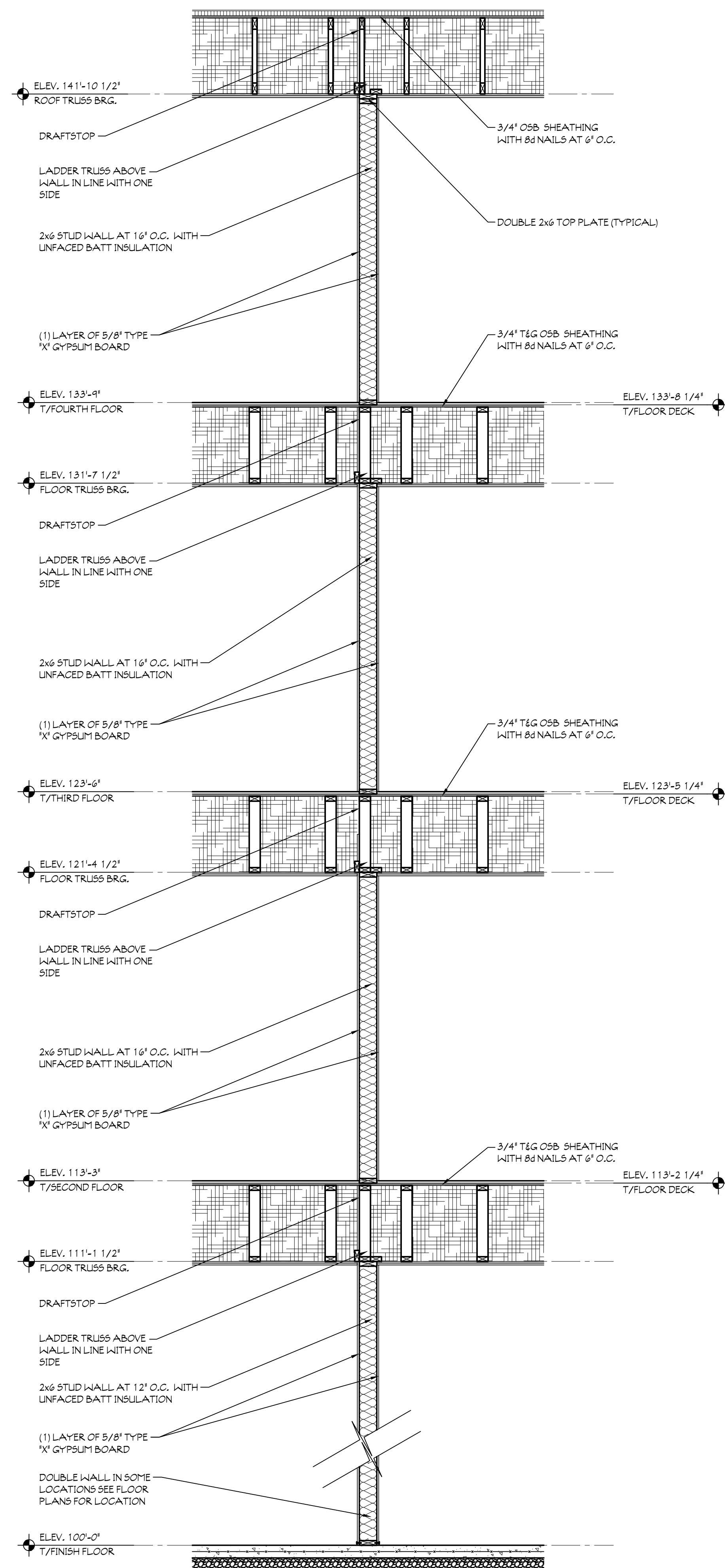
1 PARTY WALL DETAIL #1 SCALE: 1/2" = 1'-0" WALL ALL FLOORS
