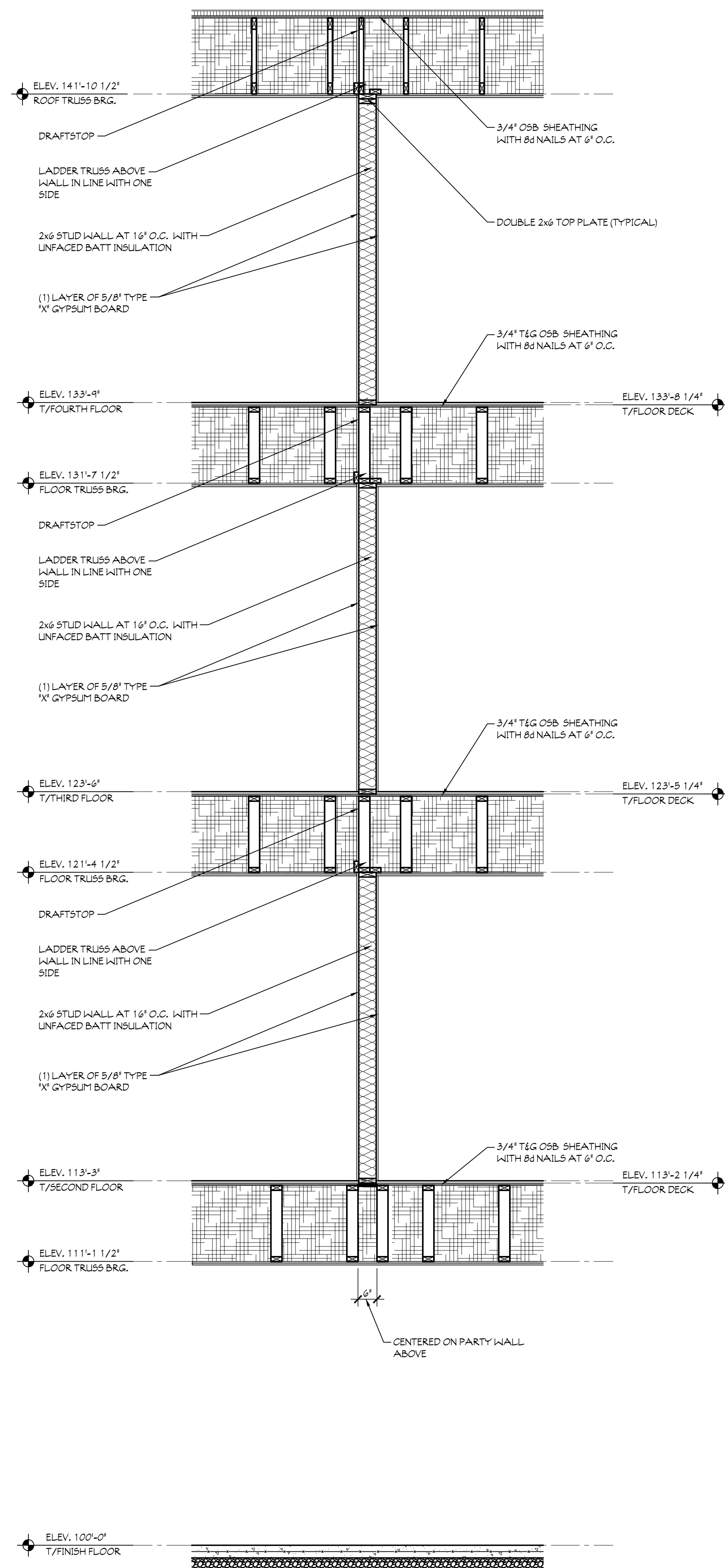
2 PARTY WALL DETAIL #2 SCALE: 1/2" = 1'-0" NO WALL 1ST FLOOR
