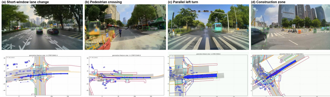
Figure 2: Four anonymized real-vehicle deployment scenarios: (a) short-window lane change, (b) pedestrian crossing, (c) parallel left turn, and (d) construction zone. Top: forward-camera frame. Bottom: the planner’s bird’s-eye view at the same moment, with the selected trajectory in blue.
