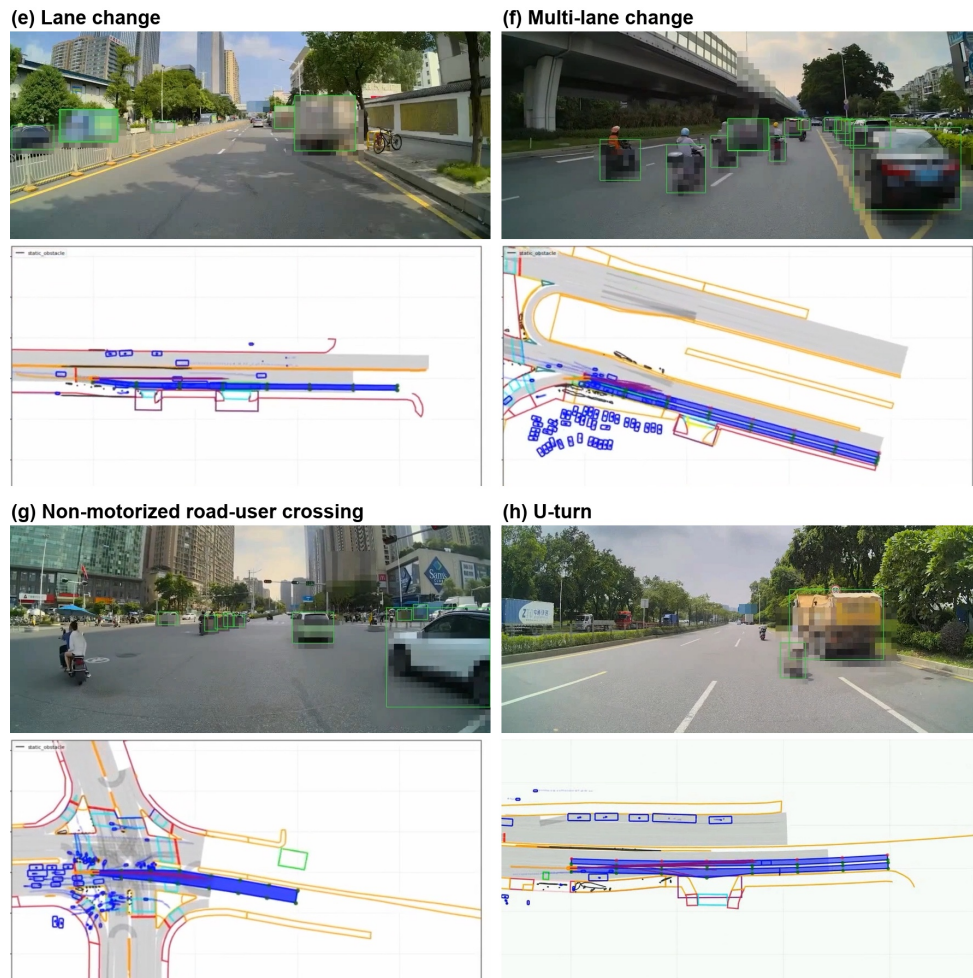
Figure 5: Real-vehicle deployment scenarios (2/2): (e) lane change, (f) multi-lane change, (g) non-motorized road-user crossing, and (h) U-turn.
