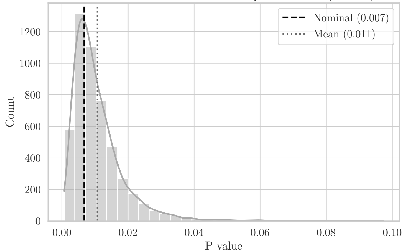
MC Distribution of P-values for QRS Distance (C1 XY)
