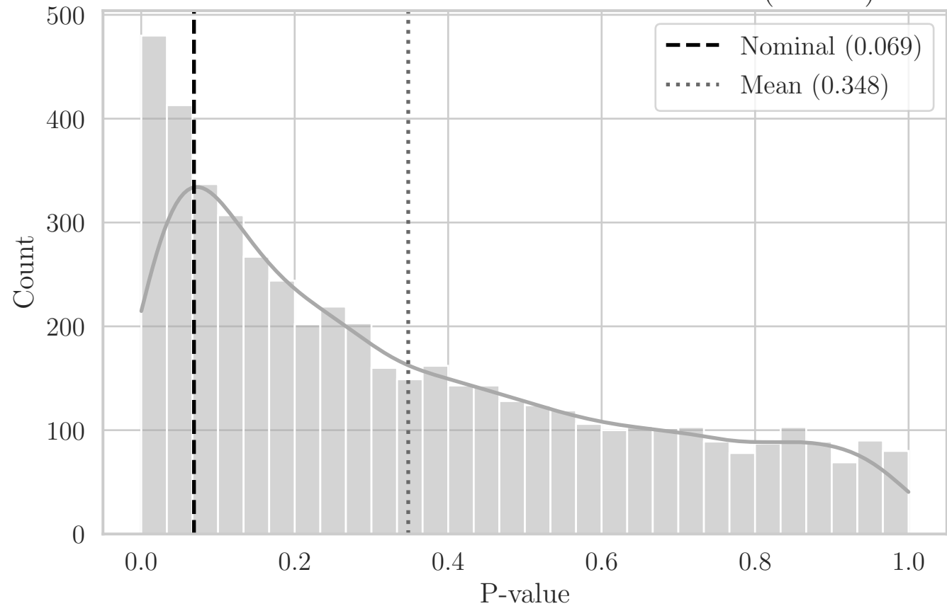
MC Distribution of P-values for ST Distance (C1 XY)
