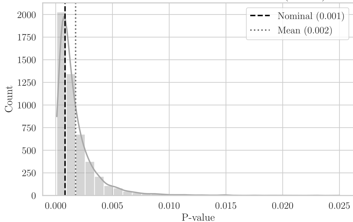
MC Distribution of P-values for T Area_Net (C1 XY)
