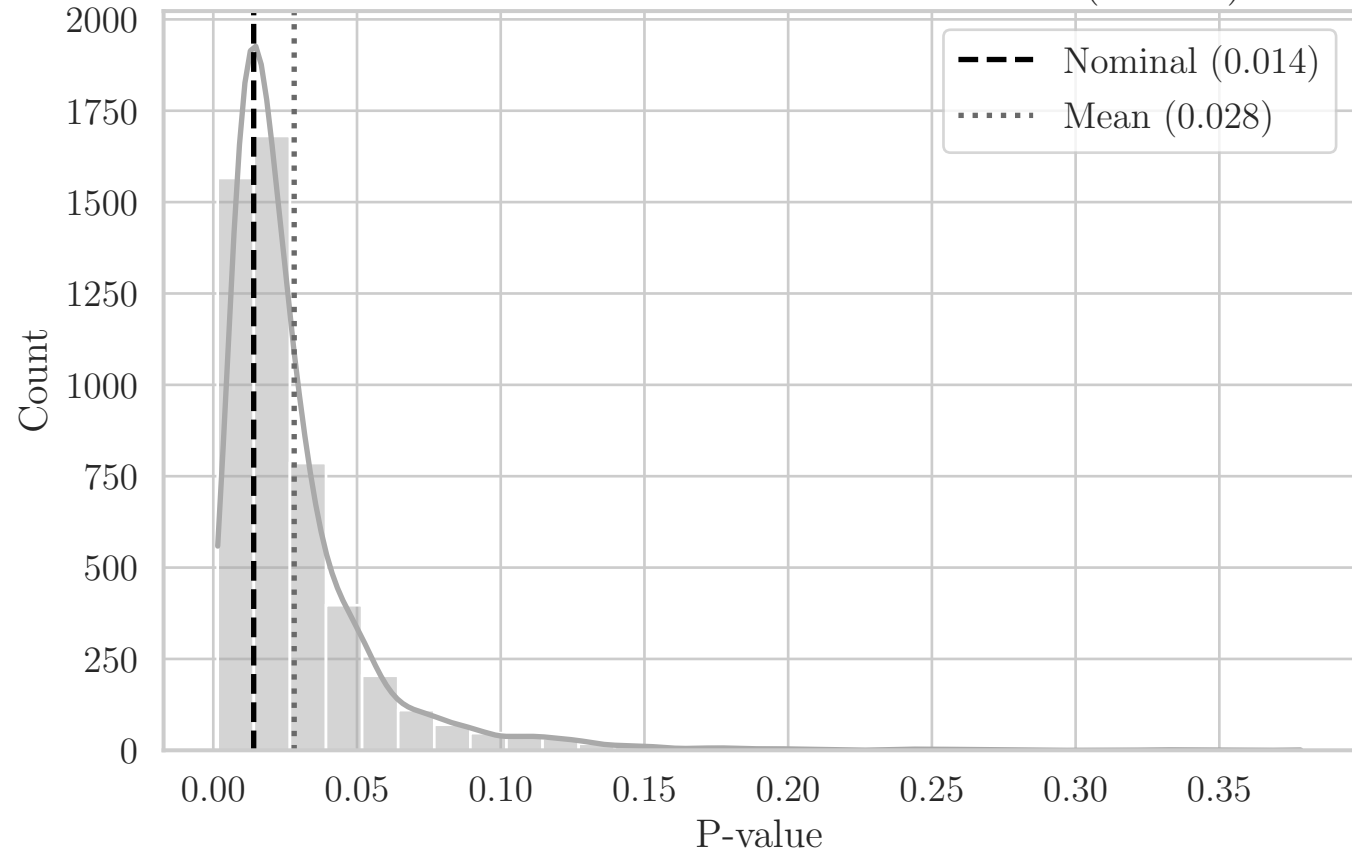
MC Distribution of P-values for T Distance (C1 XY)
