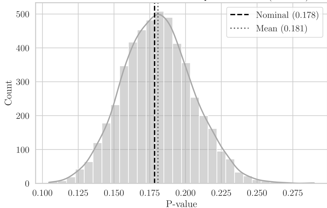
MC Distribution of P-values for QRS Area_Net (EY XY)
