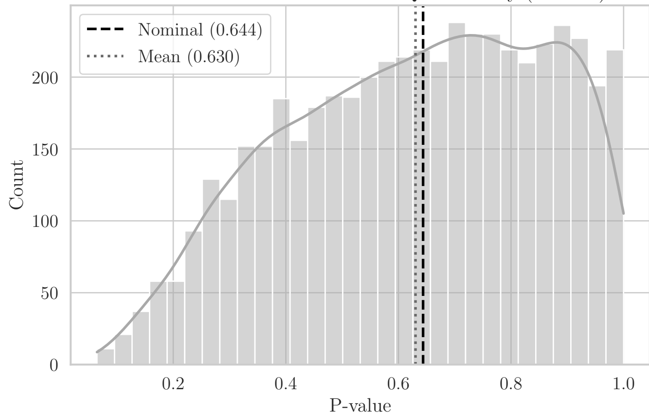
MC Distribution of P-values for QRS Solidity (EY XY)
