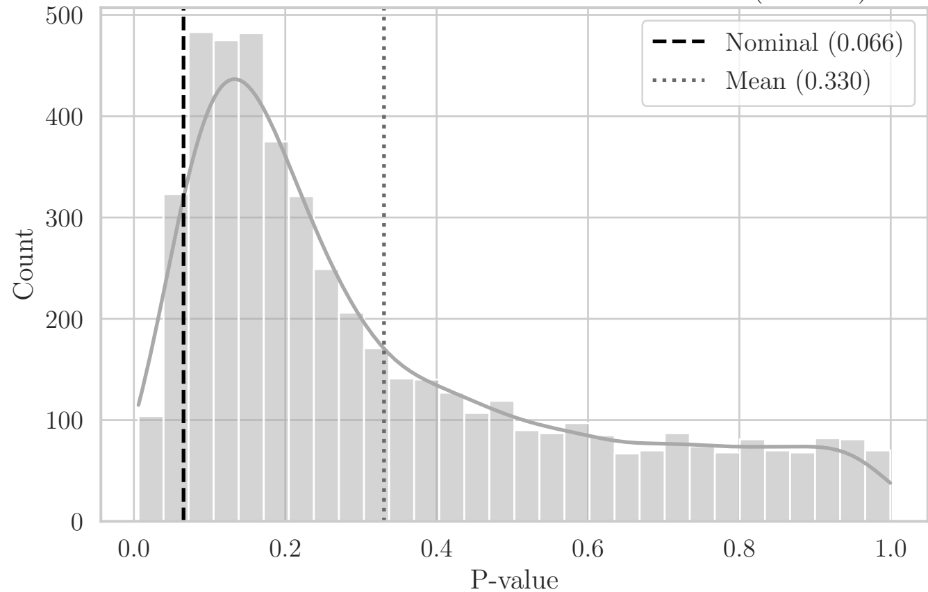
MC Distribution of P-values for ST Area_Hull (EY XY)
