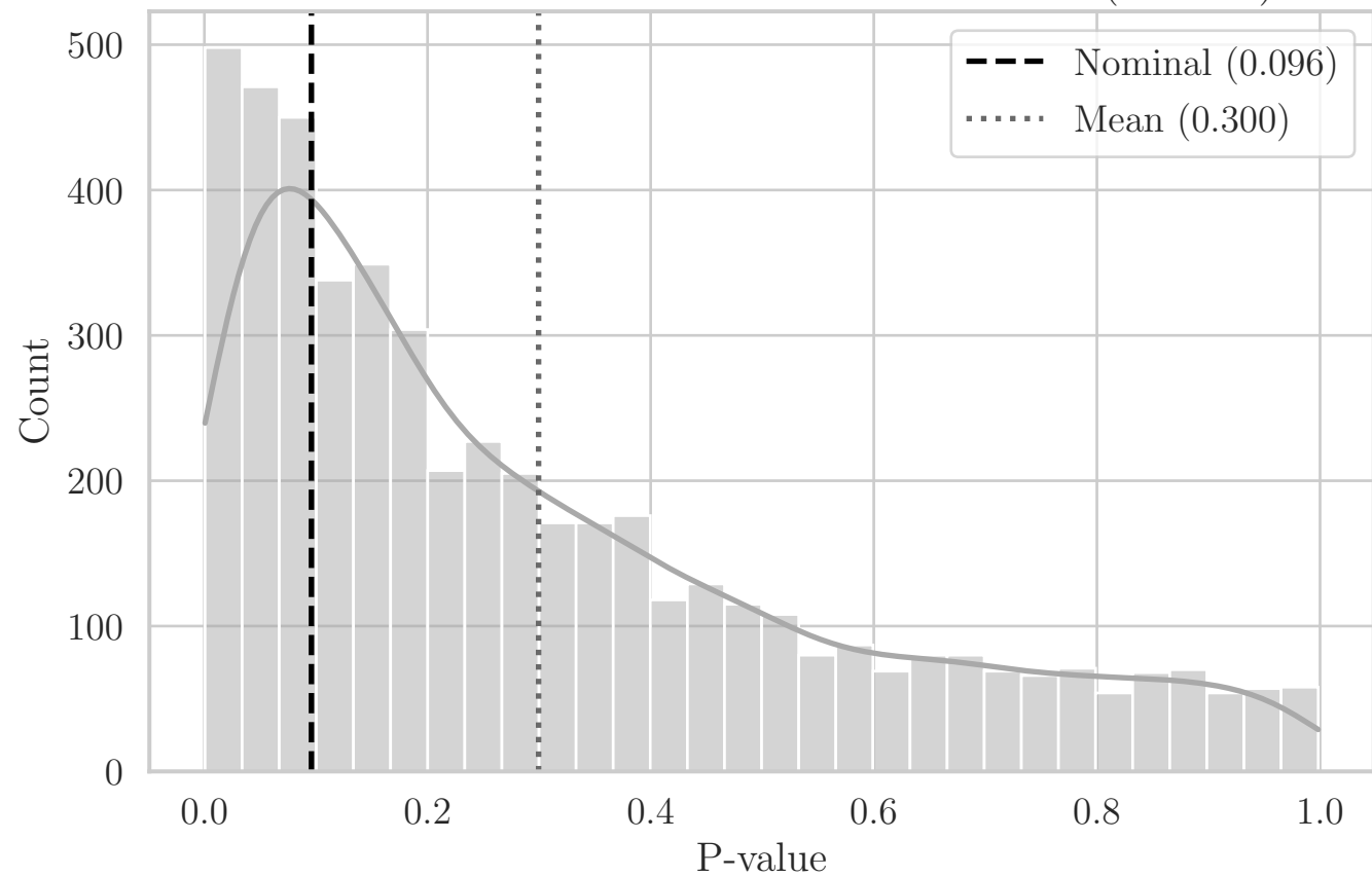
MC Distribution of P-values for ST Distance (EY XY)
