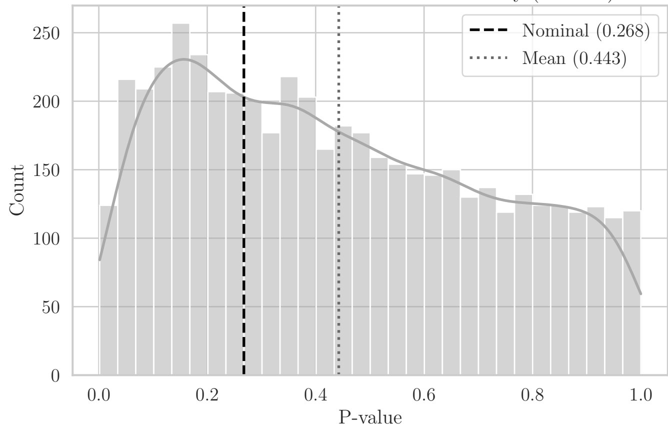
MC Distribution of P-values for ST Solidity (EY XY)
