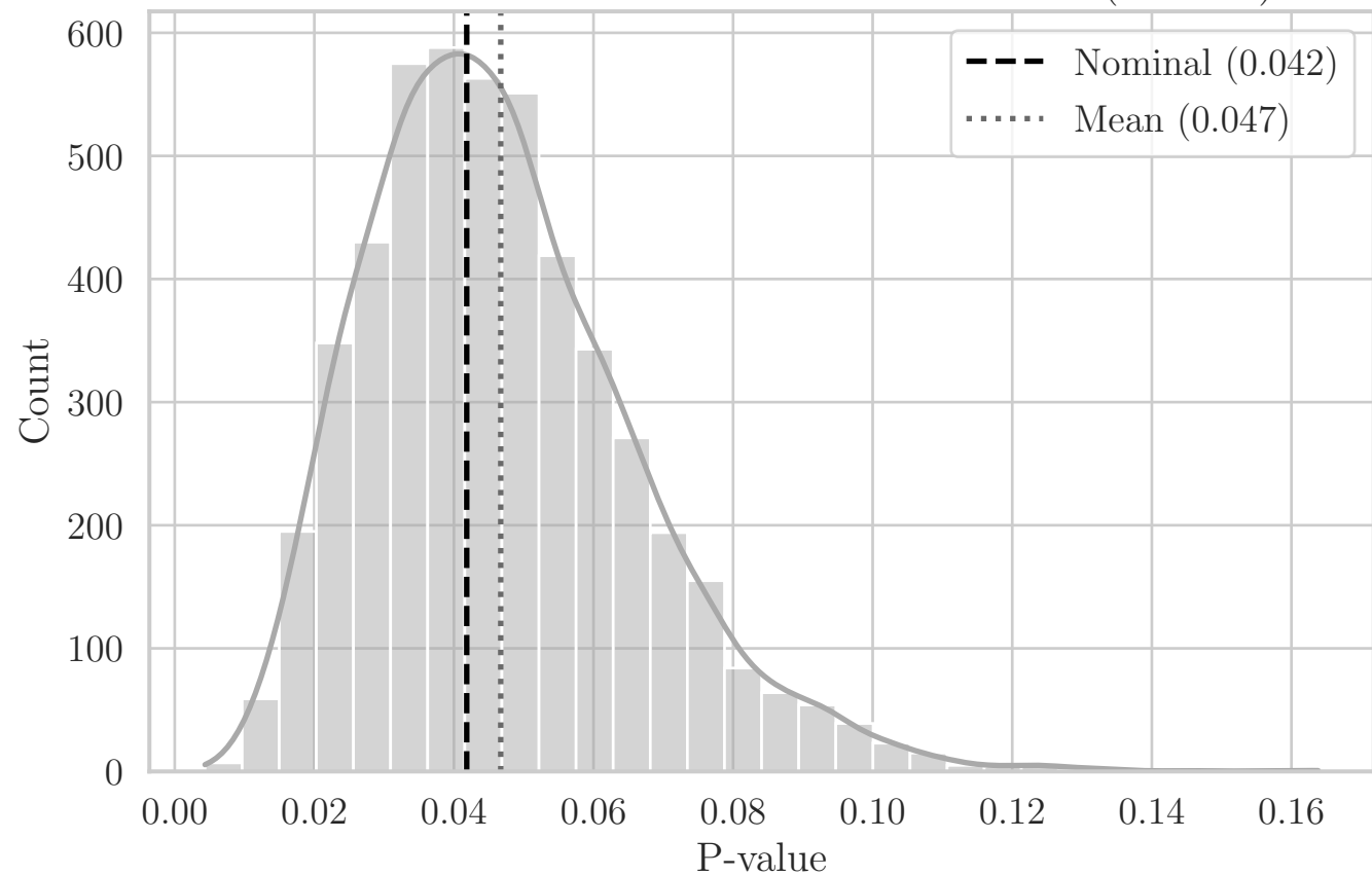
MC Distribution of P-values for T Area_Hull (EY XY)
