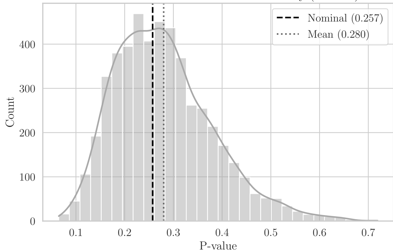
MC Distribution of P-values for T Solidity (EY XY)
