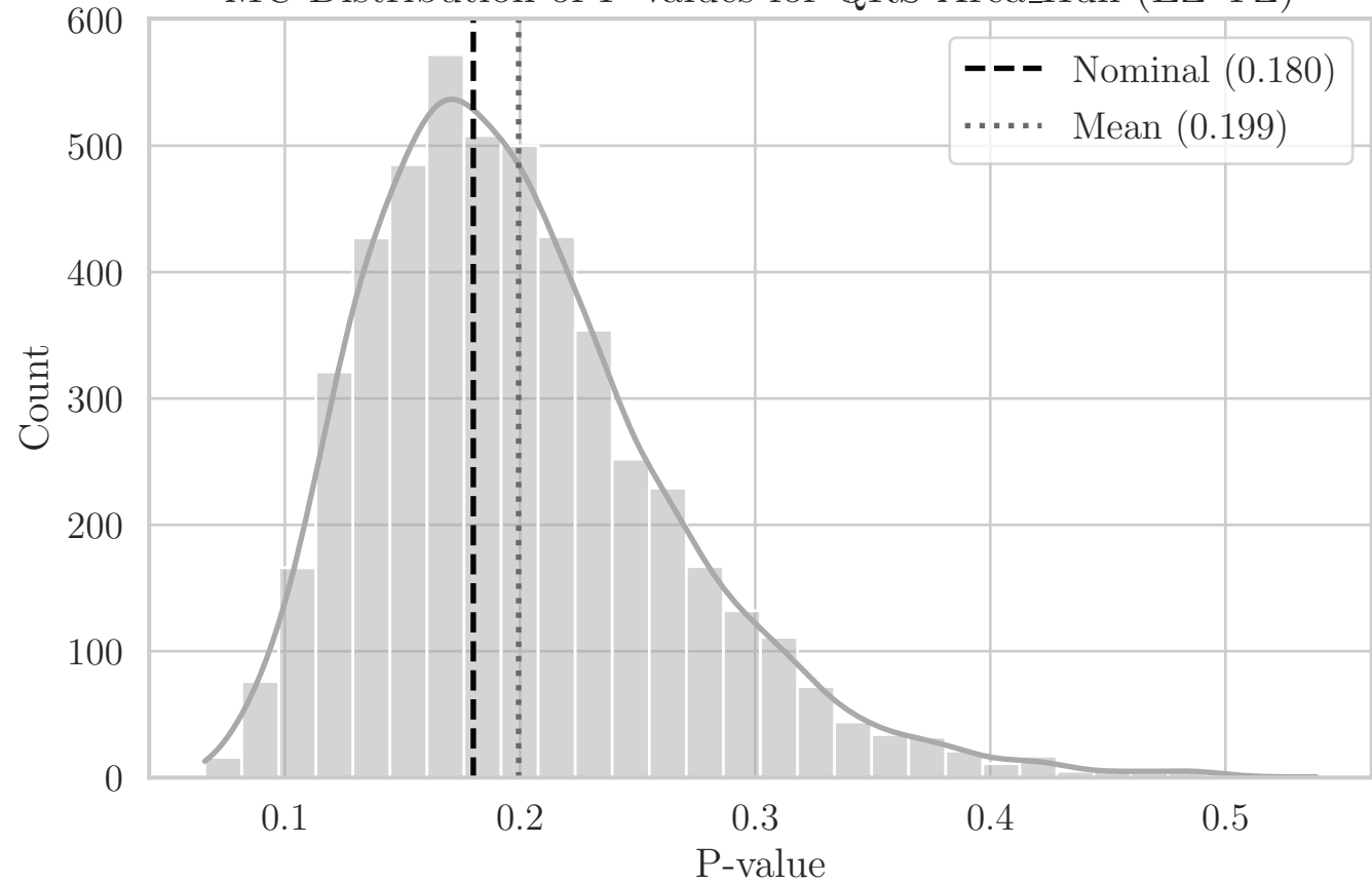
MC Distribution of P-values for QRS Area_Hull (EZ YZ)
