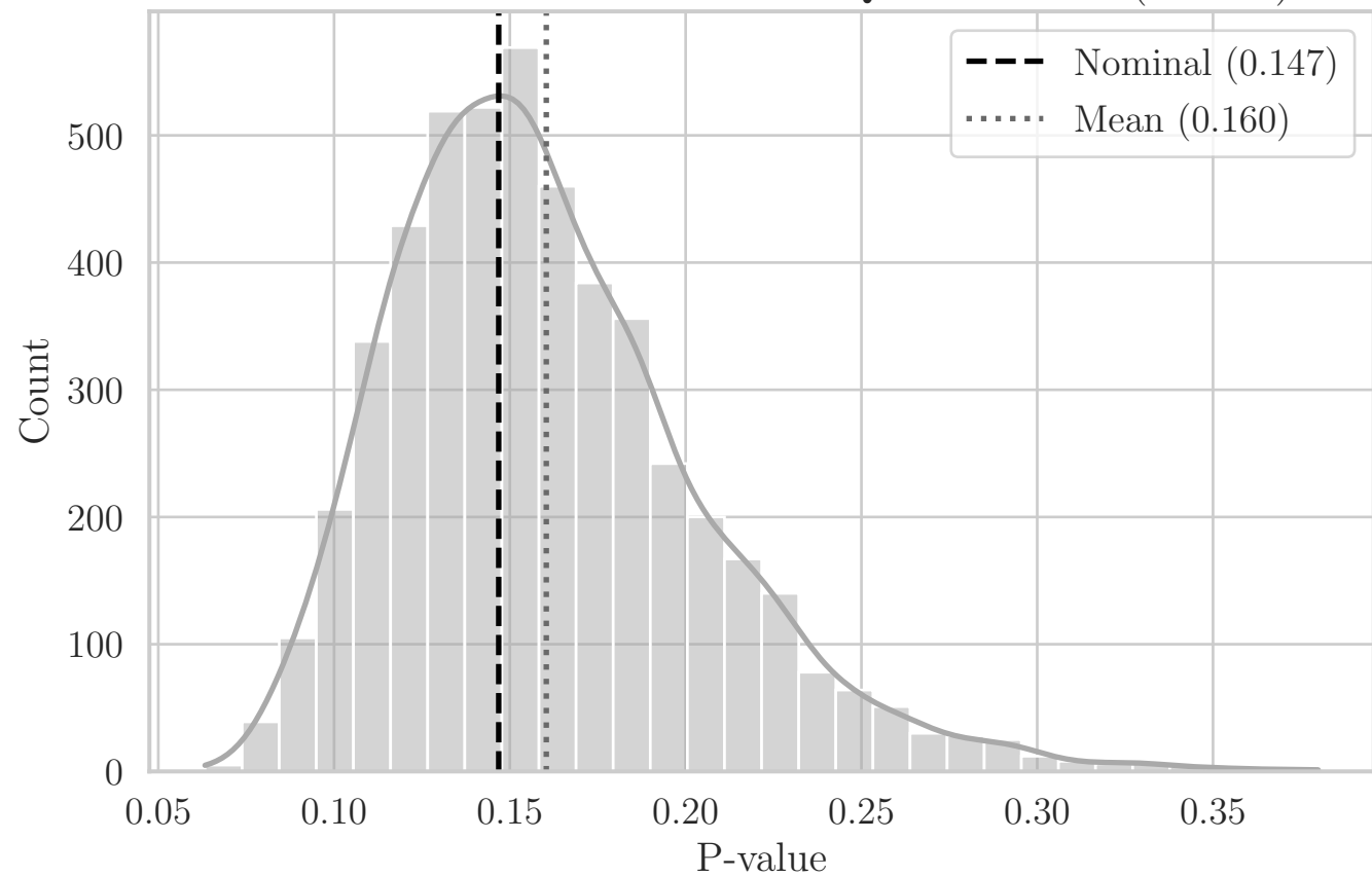
MC Distribution of P-values for QRS Area_Net (EZ YZ)
