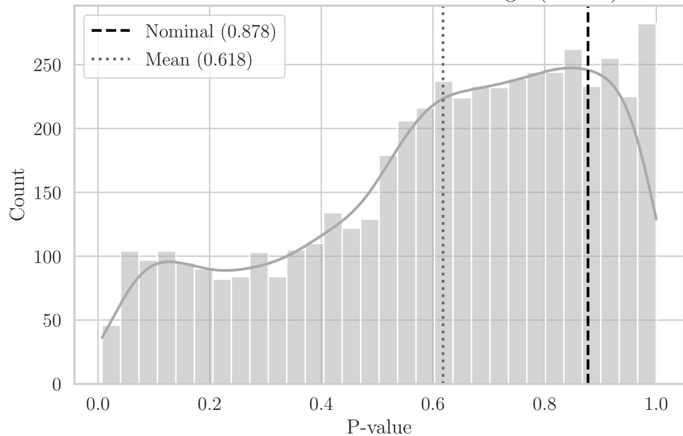
MC Distribution of P-values for ST Angle (EZ YZ)
