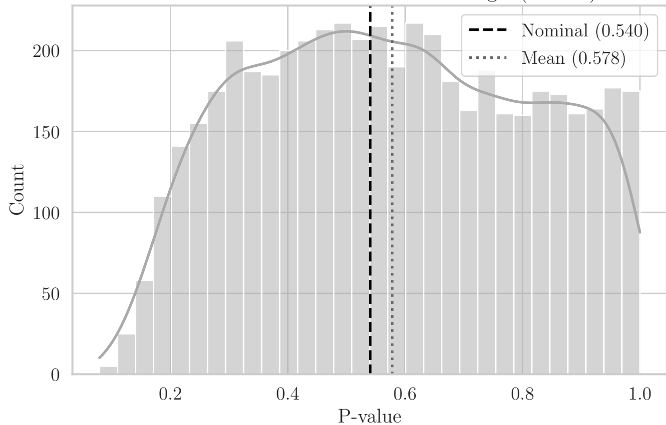
MC Distribution of P-values for T Angle (EZ YZ)
