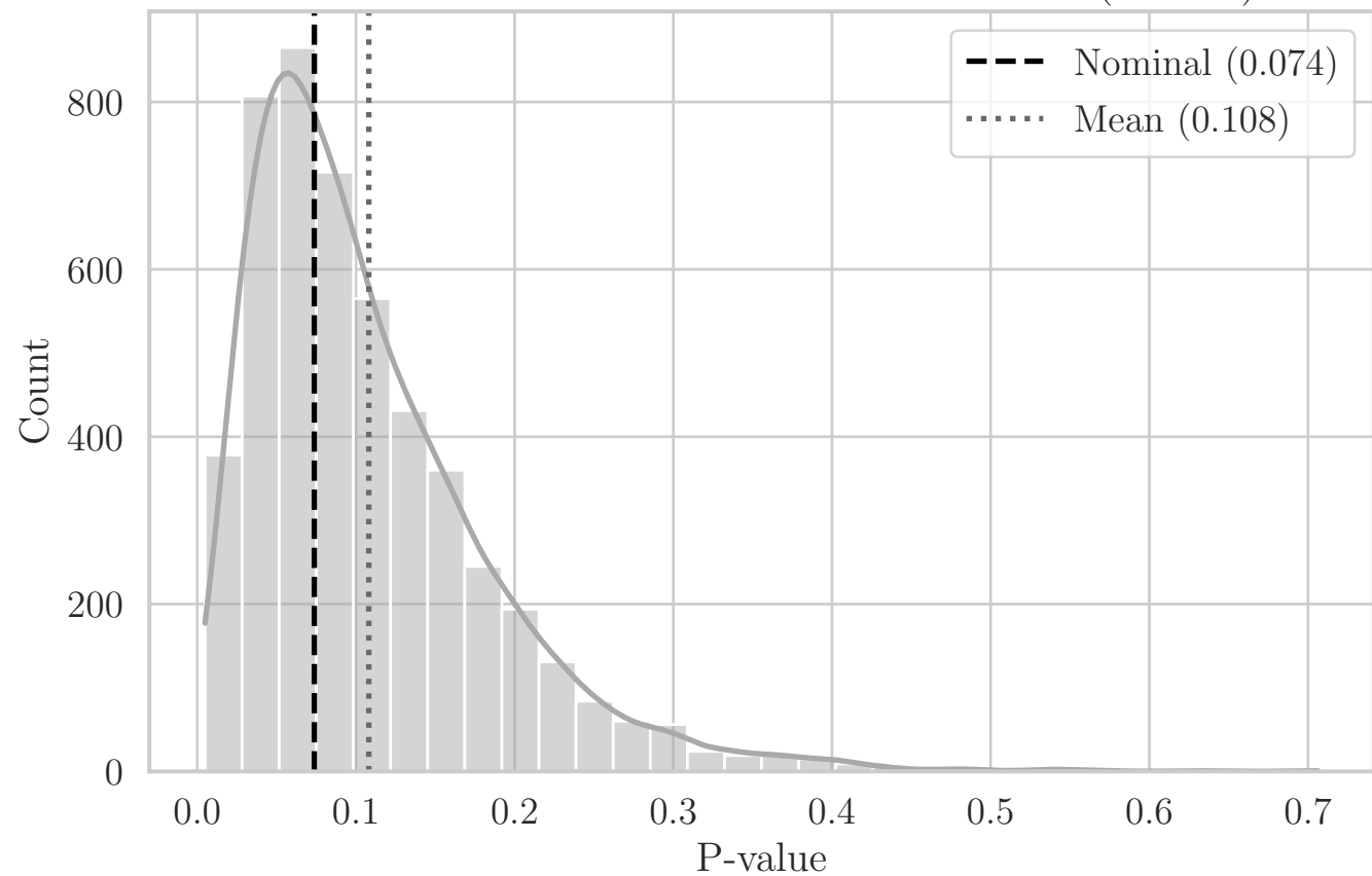
MC Distribution of P-values for T Distance (EZ YZ)
