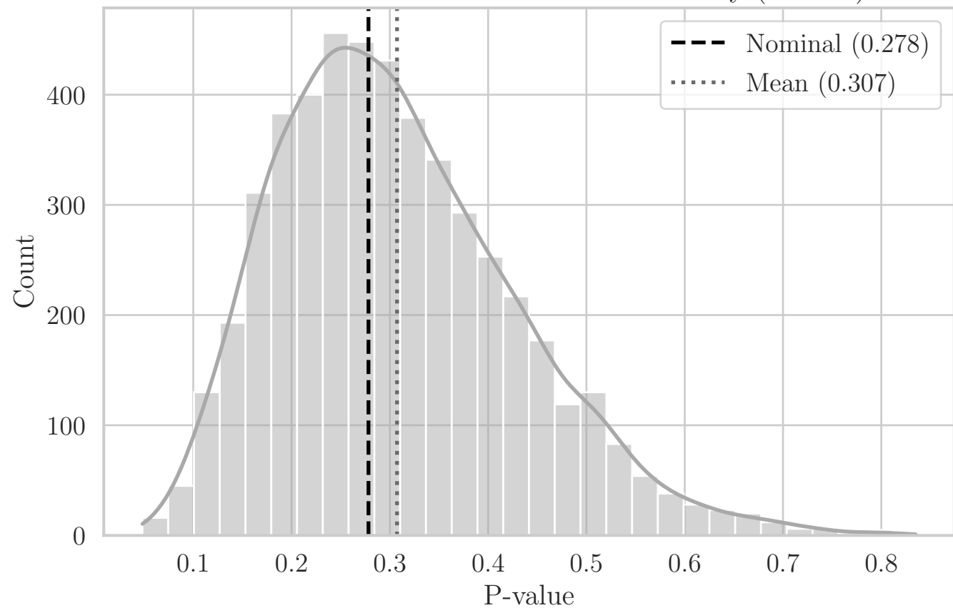
MC Distribution of P-values for T Solidity (EZ YZ)
