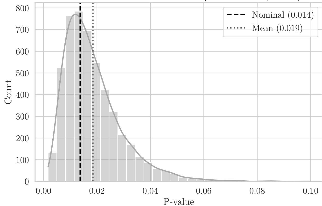
MC Distribution of P-values for QRS Distance (F0 YZ)
