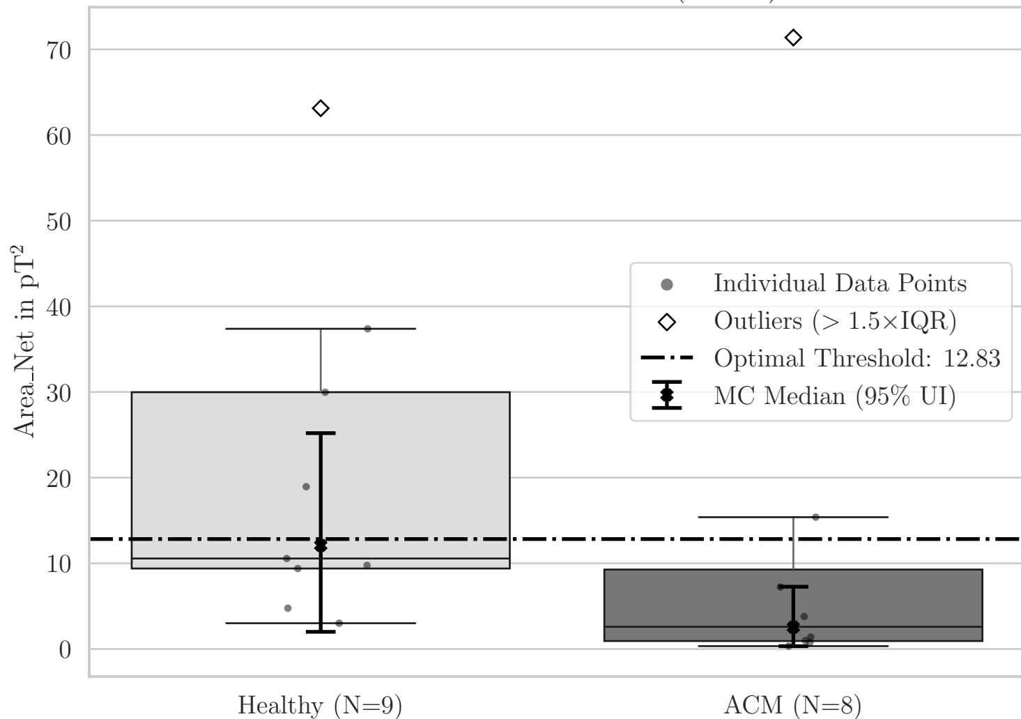
Box Plot for ST Area_Net (F0 YZ)
