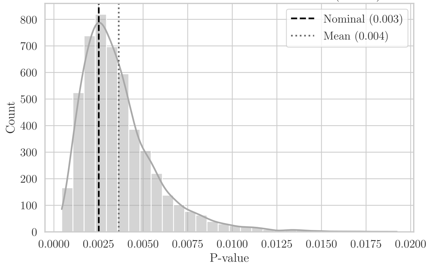
MC Distribution of P-values for T Area_Hull (F0 YZ)
