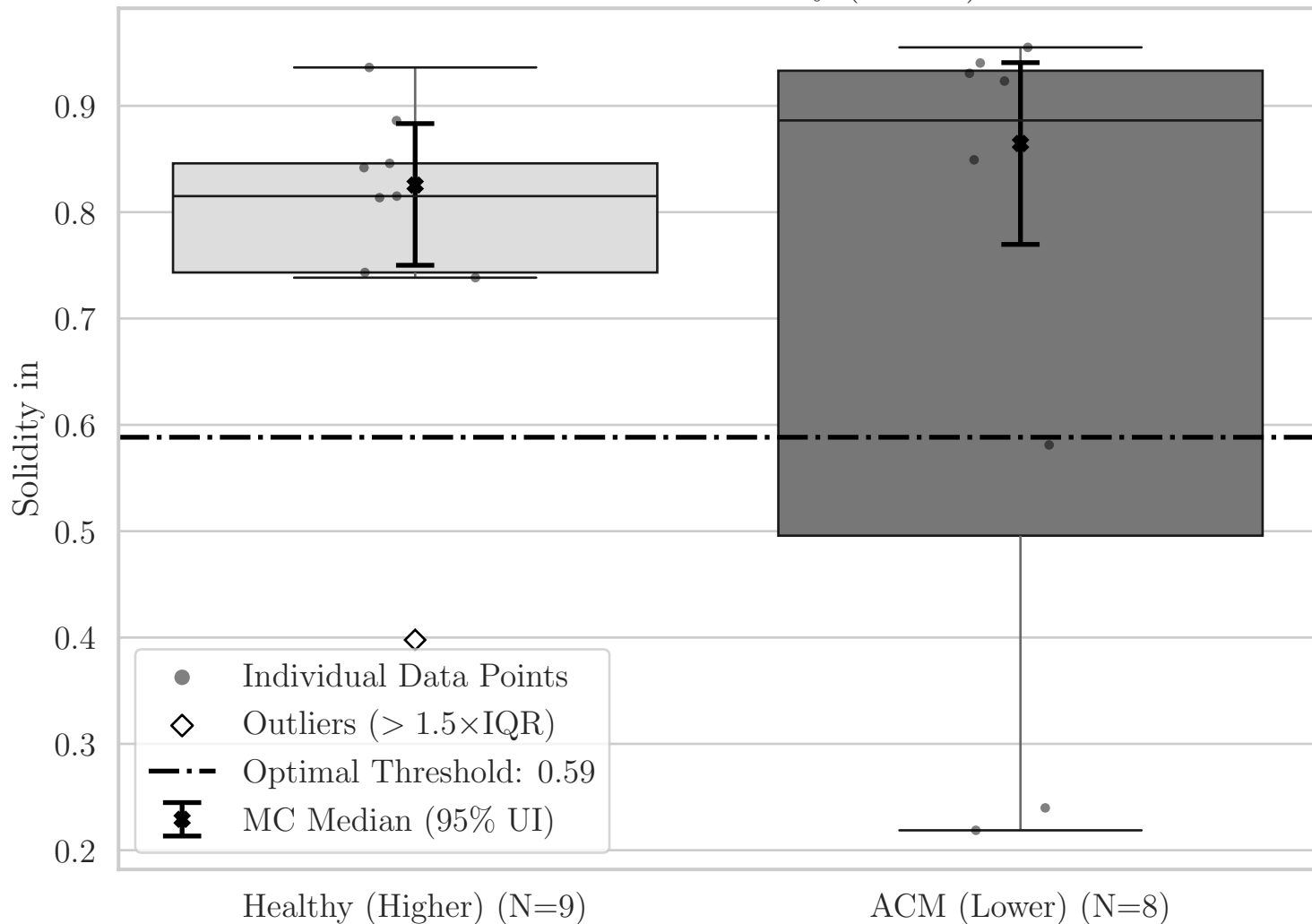
Box Plot for T Solidity (F0 YZ)
