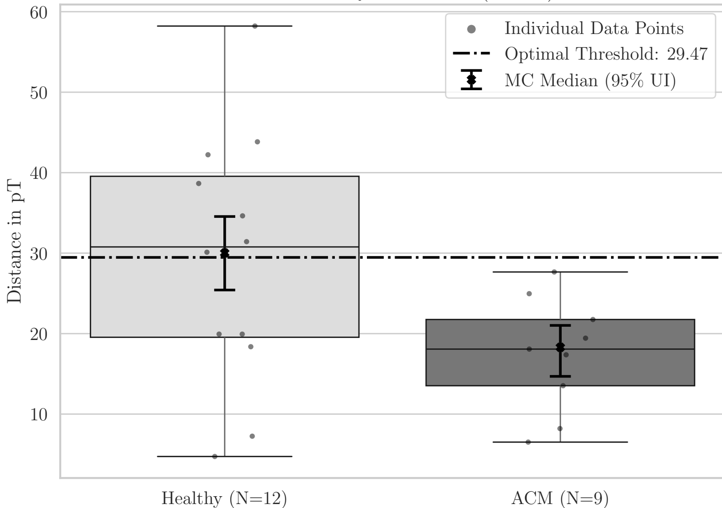
Box Plot for QRS Distance (F1 YZ)
