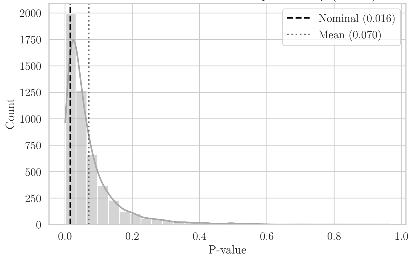
MC Distribution of P-values for QRS Solidity (F1 YZ)
