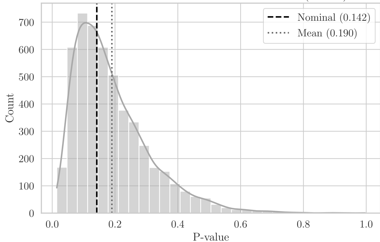
MC Distribution of P-values for T Distance (F1 YZ)
