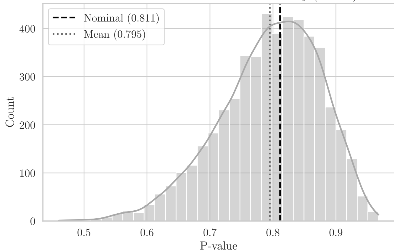
MC Distribution of P-values for T Solidity (F1 YZ)
